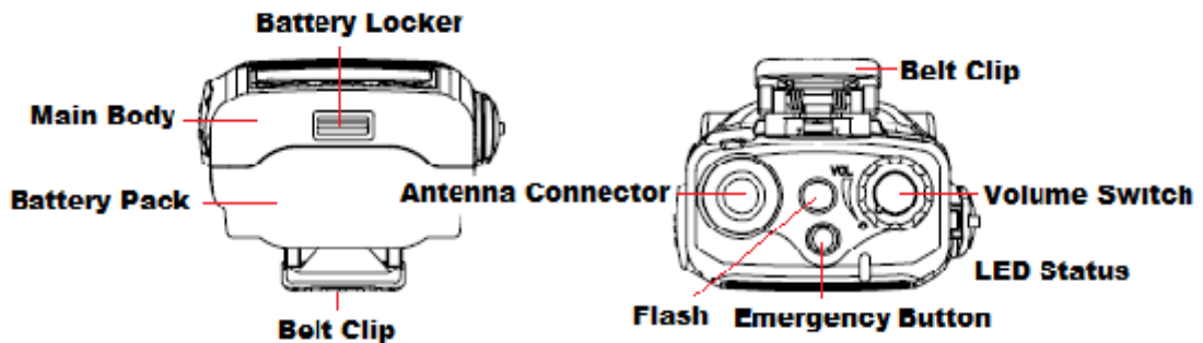
Figure 4-1) Appearance of XR Series Radio
