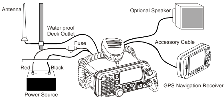
Figure 1. General Installation
