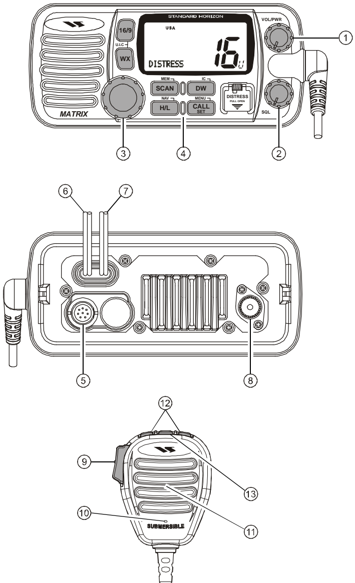
Figure 3. Controls and Connectors
