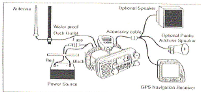
Figure 2. General Installation
