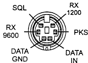
(as viewed from the rear panel)
