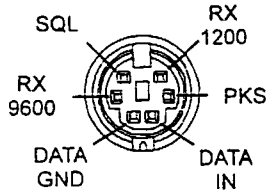
(as viewed from the rear panel)
