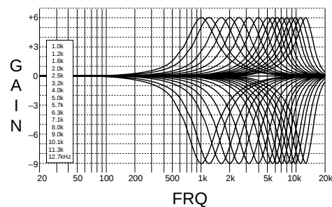
▲ PEQ Frequency Range FRQ 1.0 ~ 12.7 kHz Q 1.85 (fixed)
