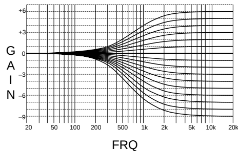
▲ HIGH Frequency Range GAIN +6 ~ -9 dB
