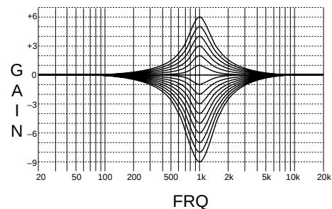
▲ PEQ Frequency Range GAIN +6 ~ -9 dB Q 1.85 (fixed)
