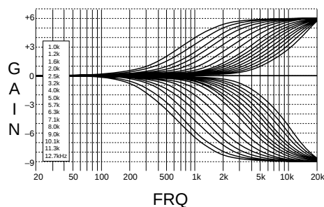
▲ HIGH Frequency Range FRQ 1.0 ~ 12.7 kHz
