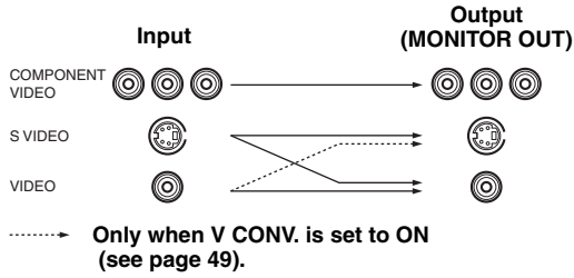
Signal flow inside this unit (HTR-5750)
