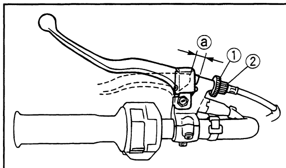
1. Locknut 2. Adjusting bolt a. 5 ~ 8 mm (0.2 ~ 0.3 in)
