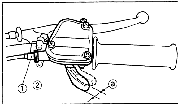
1. Adjusting bolt a. 3 ~ 5 mm (0.12 ~ 0.20 in)
