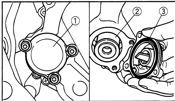
1. Oil filter cover 2. Oil filter 3. O-ring
