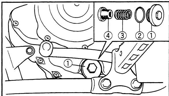
1. Drain plug (oil strainer) 2. O-ring 3. Compression spring 4. Oil strainer
