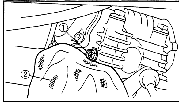
1. Oil gallery bolt
