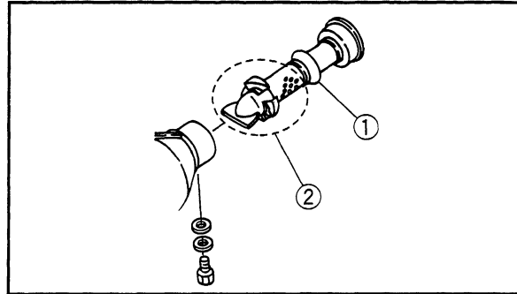
1. Tailpipe 2. Spark arrester
