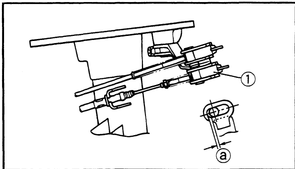
1. Adjusting nut (brake cable) a. 0 ~ 1 mm (0 ~ 0.04 in)
