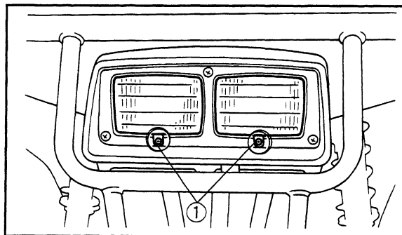
1. Adjusting screw (x 2)
