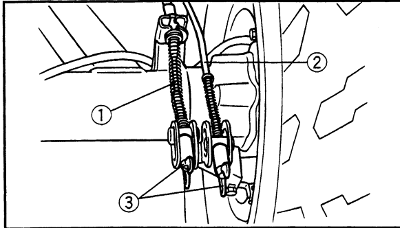
1. Brake cable 2. Brake rod 3. Adjusting nut (x 2)
