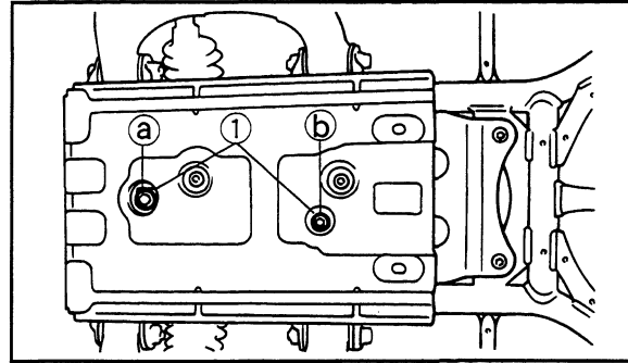
1. Drain plug (x2) a. Front drain plug b. Rear drain plug
