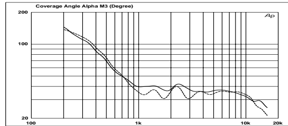
• Figure 10: Nominal Coverage @ -6 dB (Degrees)
