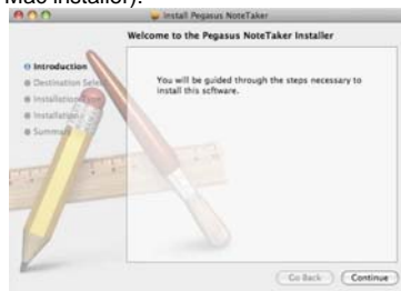
Figure 1: NoteTaker Installer
