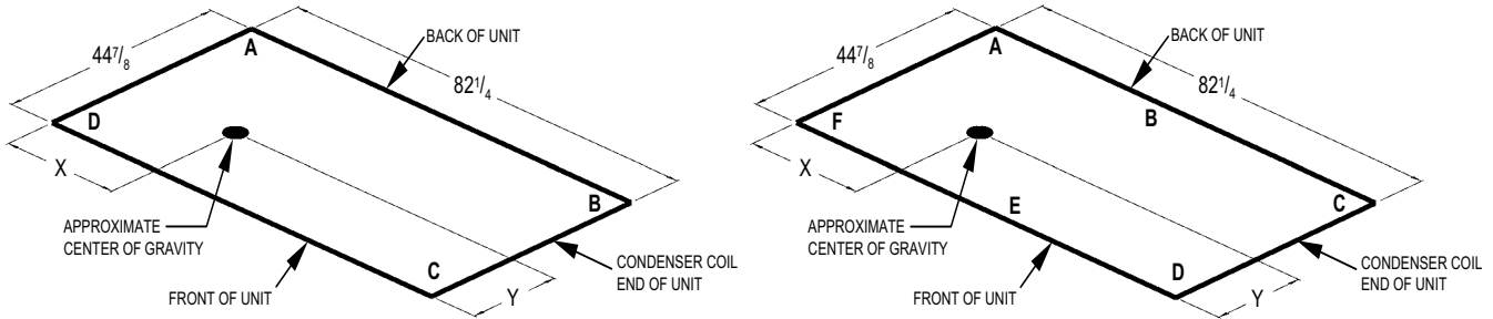
FIGURE 10 - FOUR AND SIX POINT LOADING
