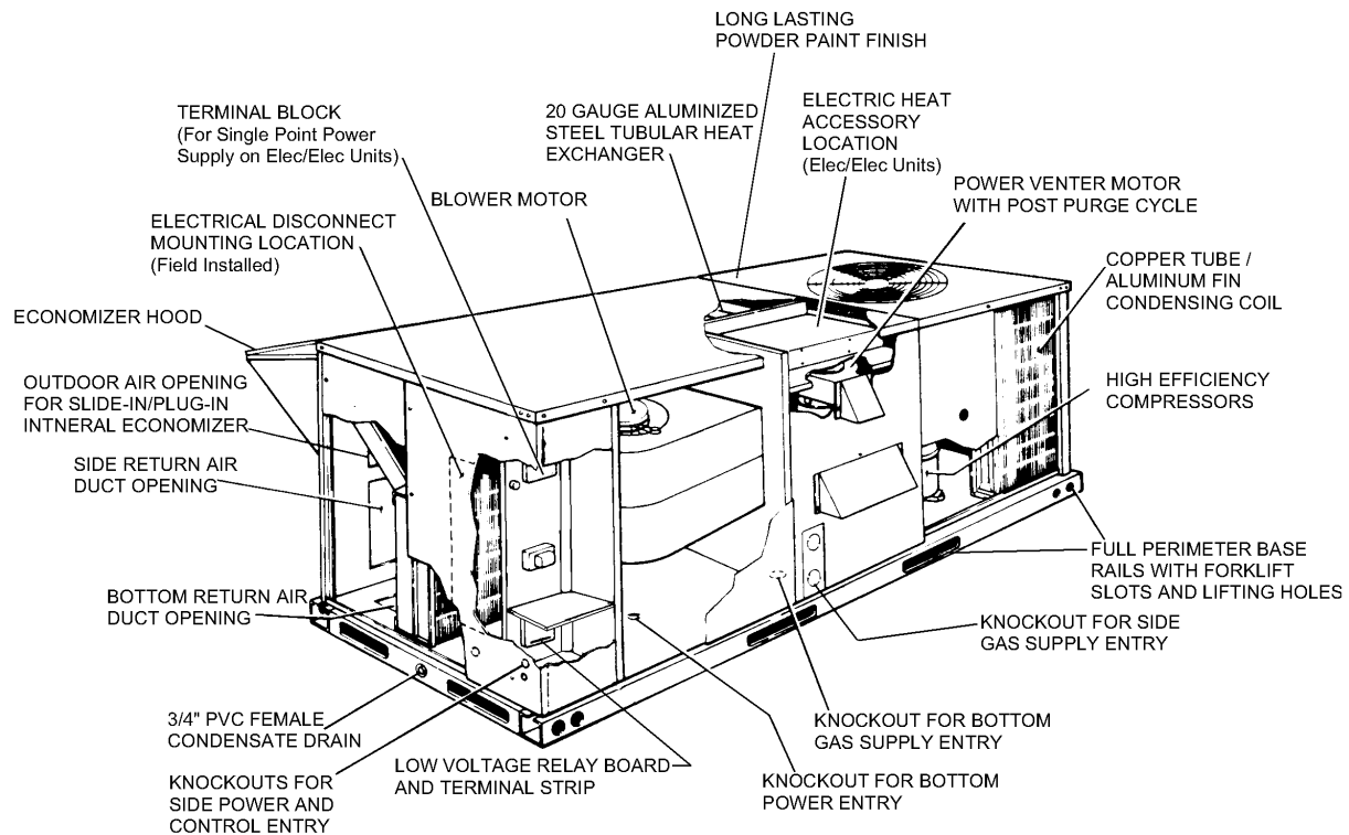
FIGURE 1 - UNIT CUTAWAY
