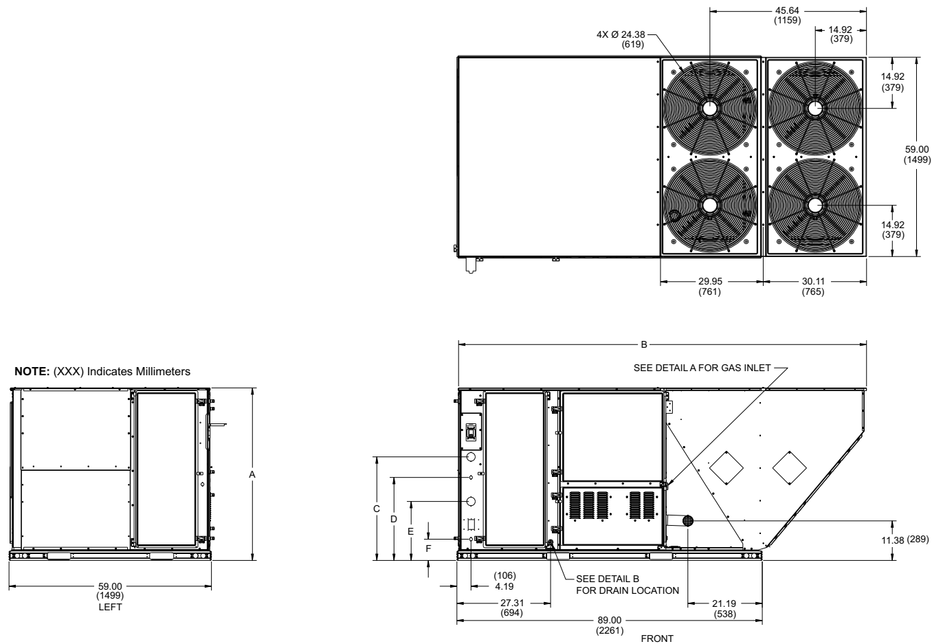
ZF090-150 Unit Physical Dimensions Imperial
