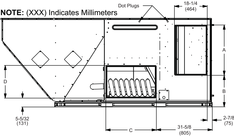
ZF Side Duct Dimensions Imperial
