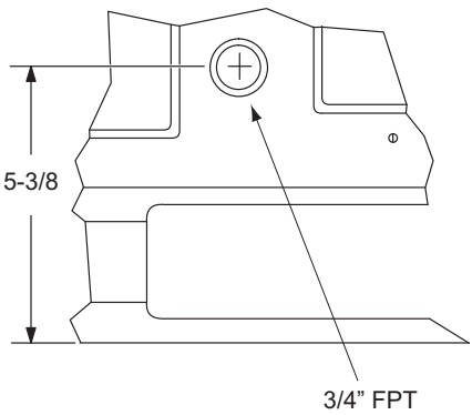
42" CABINET
