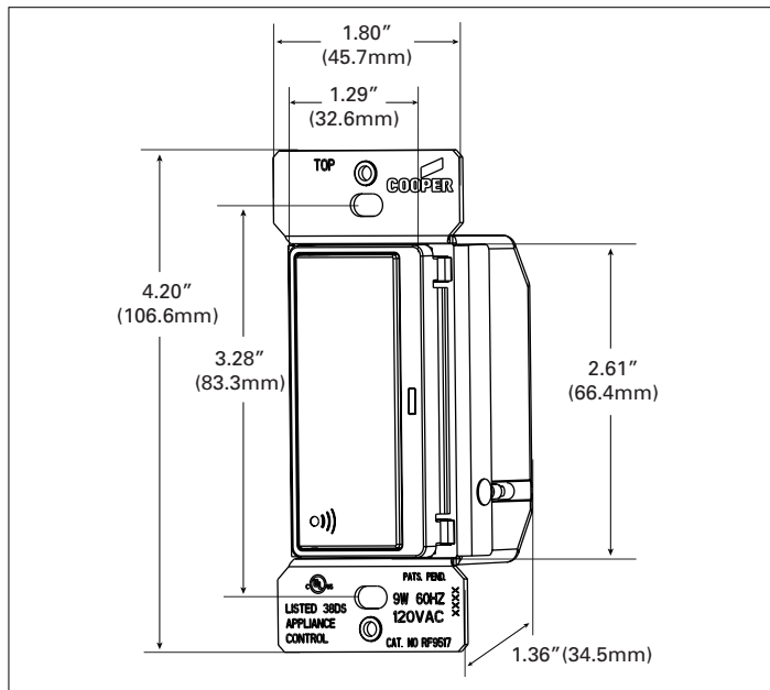
Figure 1. RF9517
