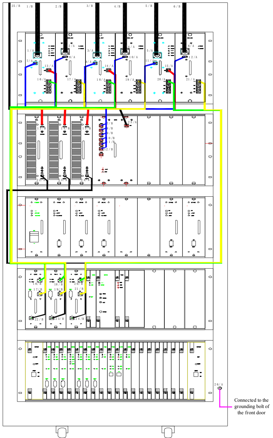
Fig. 7.2-6 Front Panel Wiring for the Rack of the Single-carrier Three-sector BTS
