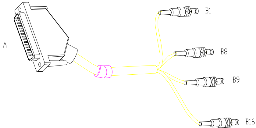
Fig. 7.4-1 Terminals of the 100Ω Cable
