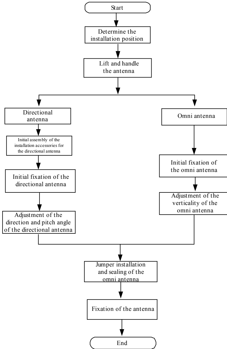
Fig. 10.3-1 Antenna Installation Flow
