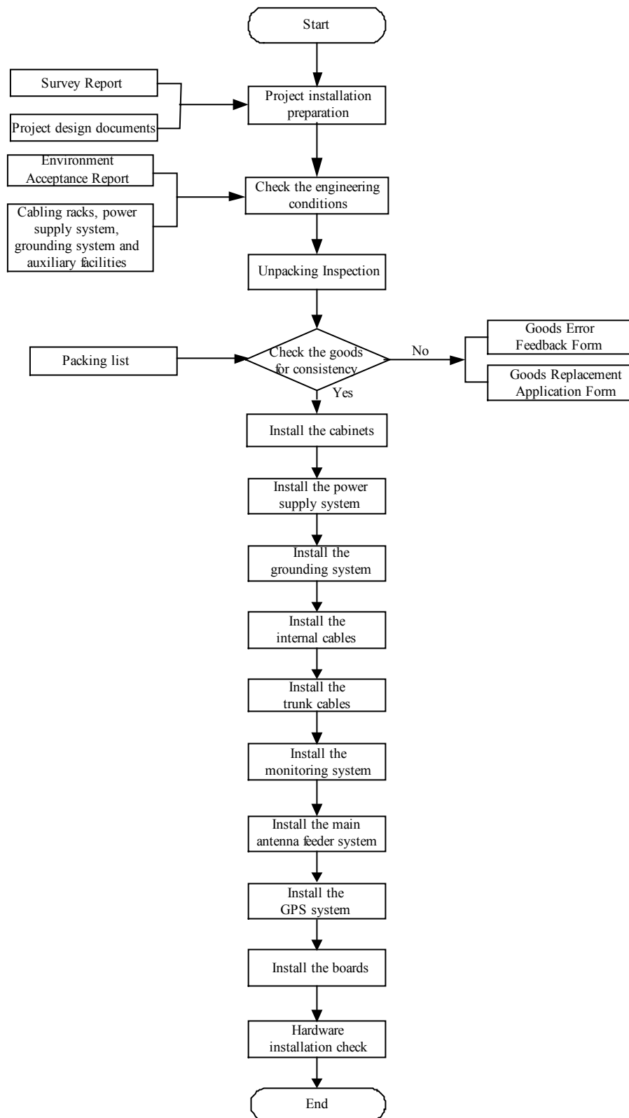
Fig. 1.2-1 Hardware Installation Flow
