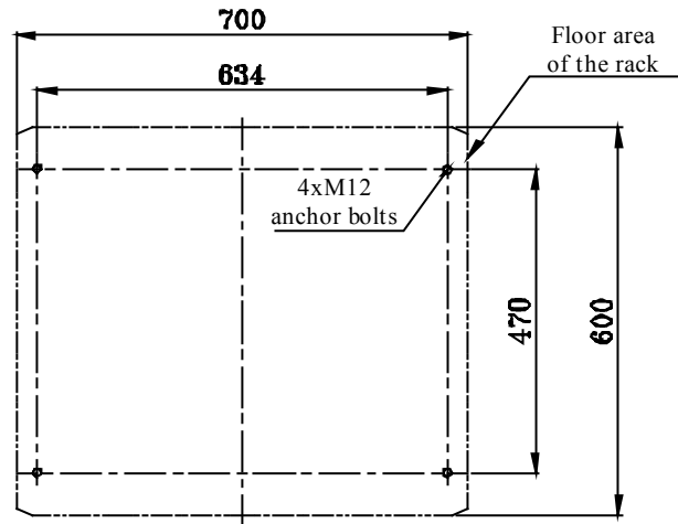
Fig. 4.3-3 Installation Holes of the BTS Rack
