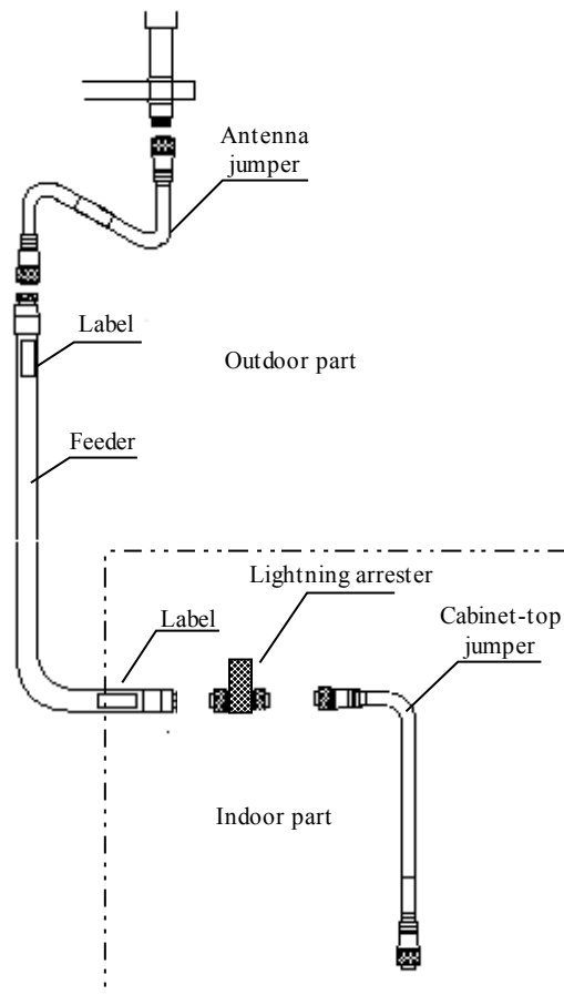
Fig. 10.4-5 Structure of a BTS Feeder
