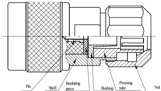
Fig. 11.4-3 Structure of the N-J7A Cable Assembly
