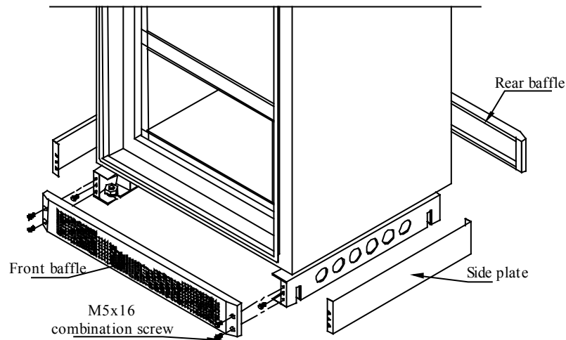
Fig. 4.3-5 Installing the Rack Baffle Plates
