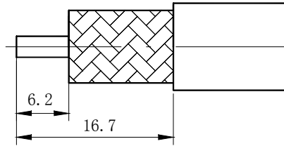
Fig. 11.4-1 Stripping the GPS Coaxial Cable
