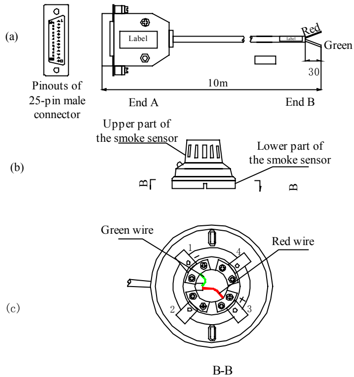
Fig. 9.2-1 Installing the Smog Sensor Base
