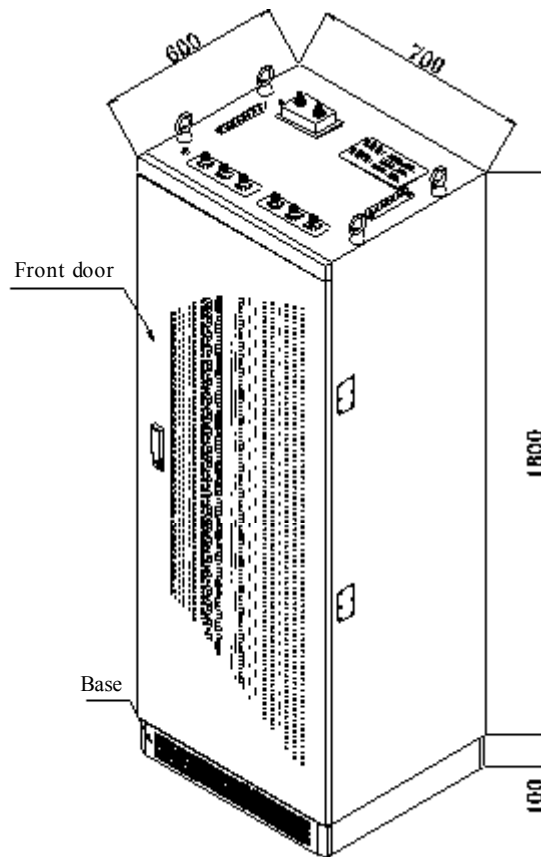
Fig. 4.1-1 Outside View and Dimensions of the Rack
