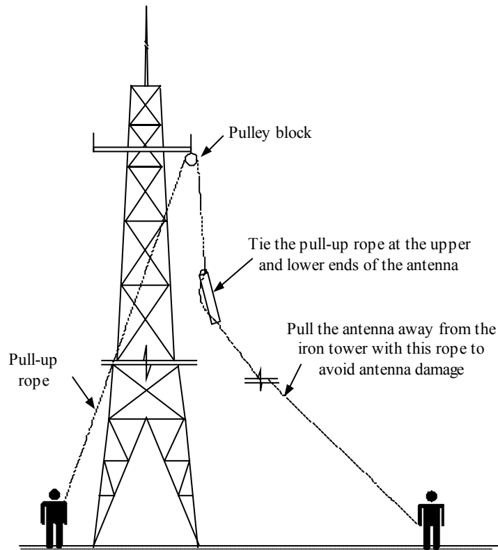
Fig. 10.4-1 Hoisting an Antenna
