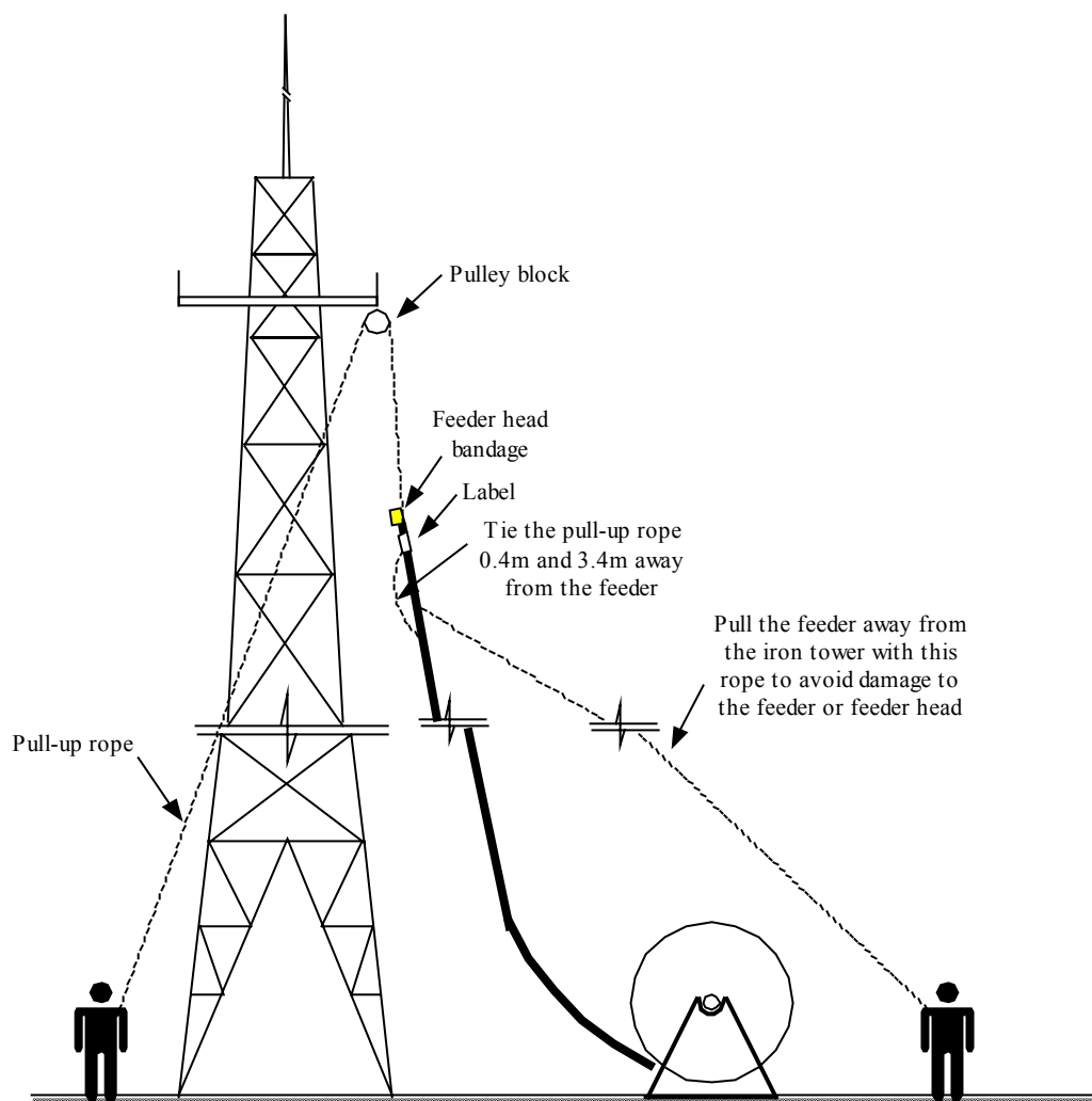
Fig. 10.4-12 Hoisting the Feeder to the Tower
