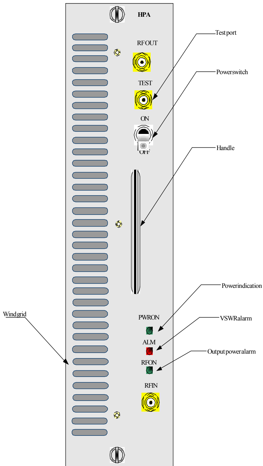
Fig. 12.2-2 Structure of the HPA Front Panel
