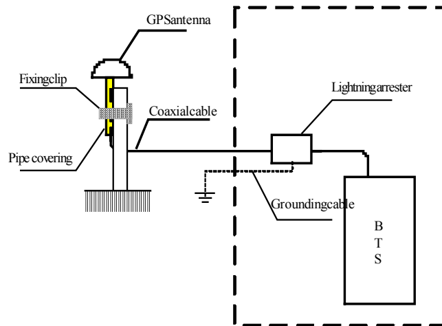
Fig. 11.2-1 Structure of the GPS Antenna Feeder System
