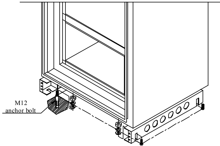
Fig. 4.3-4 Fixing the Rack
