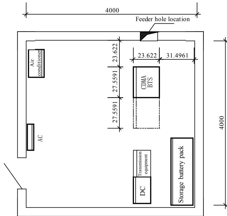
Fig. 4.2-1 Layout of Equipment inside the ZXC10 BTSB I28A Equipment Room
