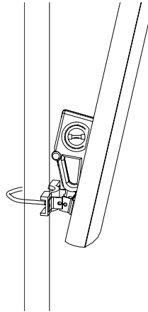
Fig. 10.4-3 Adjusting the Pitch Angle of the Antenna
