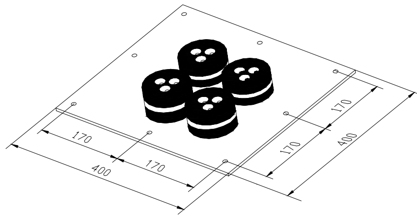
Fig. 10.4-4 Structure of the Feeder Window
