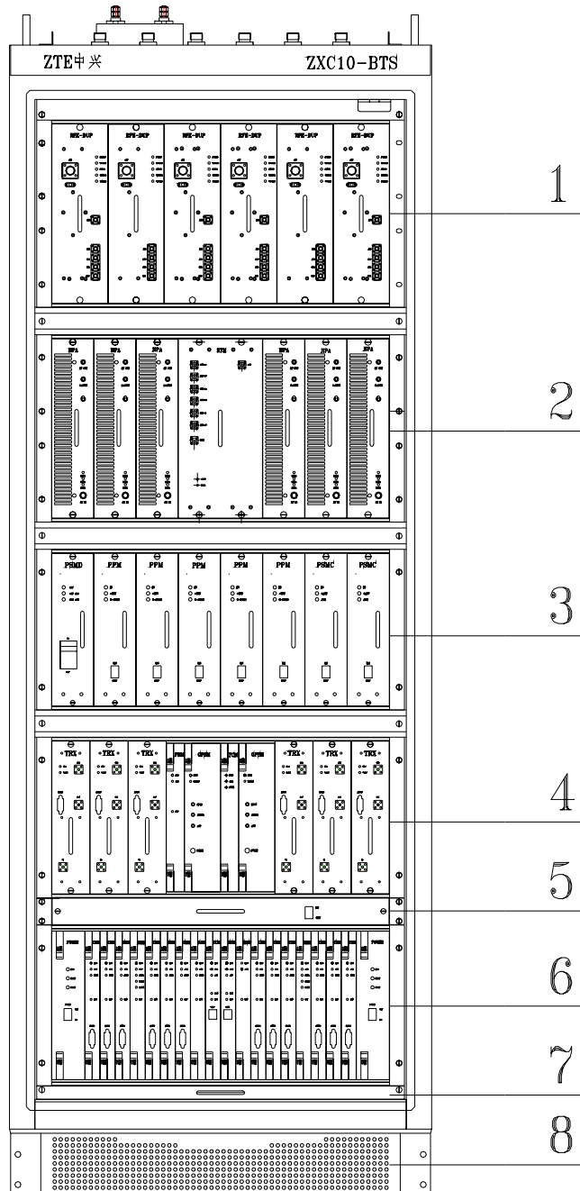
1. RFE plug-in shelf base 2. HPA plug-in shelf 3. PSMD/PSMC plug-in shelf 4. TRX plug-in shelf 5. Fan plug-in shelf 6. BDS plug-in shelf 7. Dust filtering plug-in shelf 8. Base
