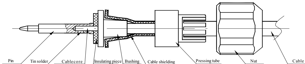
Fig. 11.4-2 Welding the Pins of the GPS Connector
