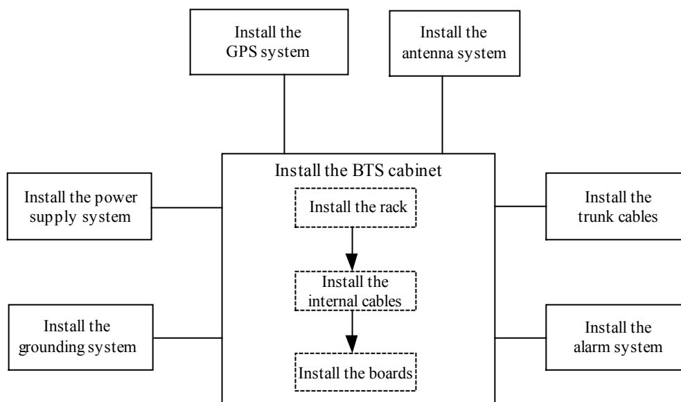
Fig. 1.1-2 Schematic Diagram of the BTS Equipment Installation
