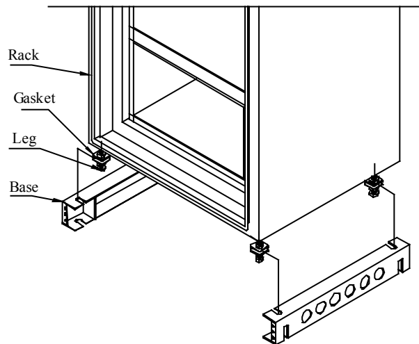
Fig. 4.3-2 Fixing the Base with the Rack
