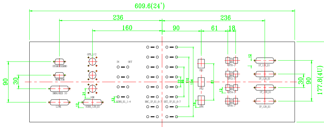
Fig. 7.4-4 BTS Rack-top Interface Board
