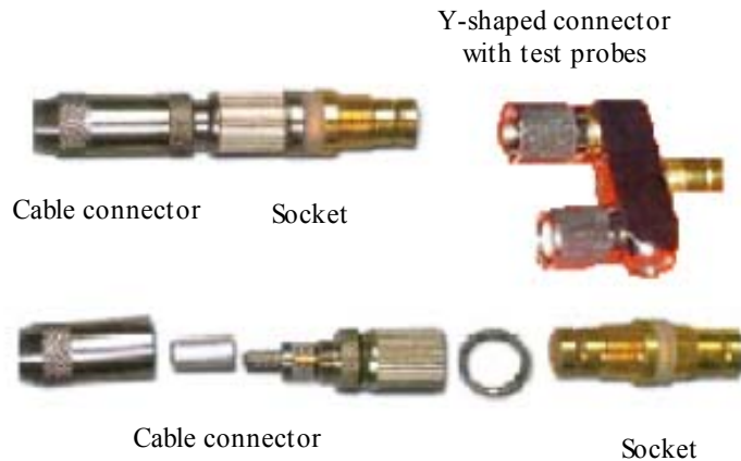
Fig. 8.2-2 Coaxial Connector of the DDF
