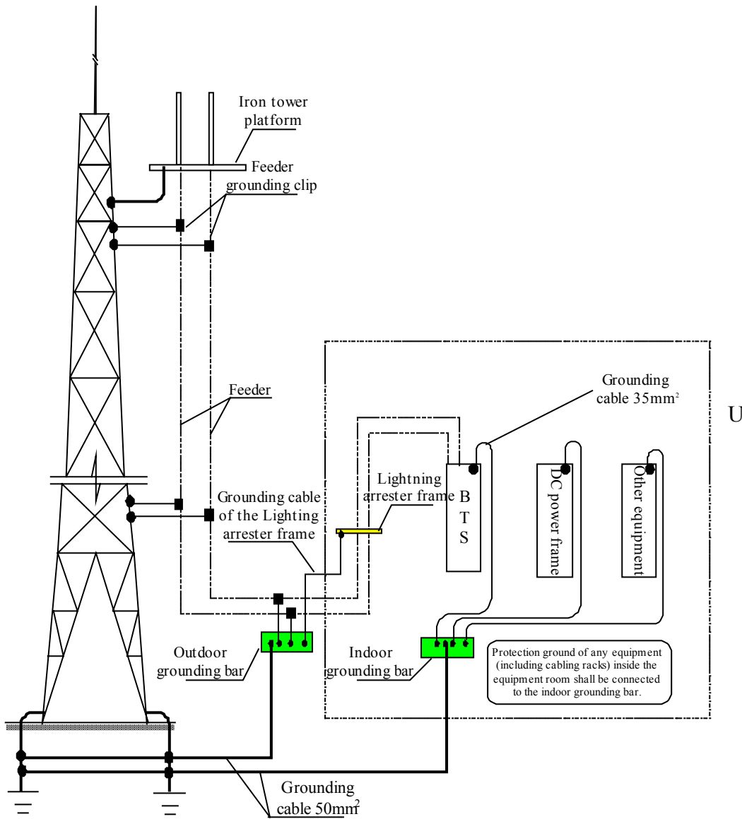
Fig. 6.1-1 Wiring for the BTS Ground
