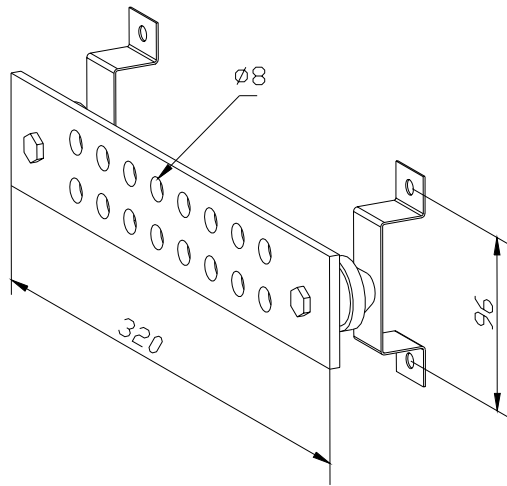
Fig. 6.2-1 Profile of the Grounding Copper Bar
