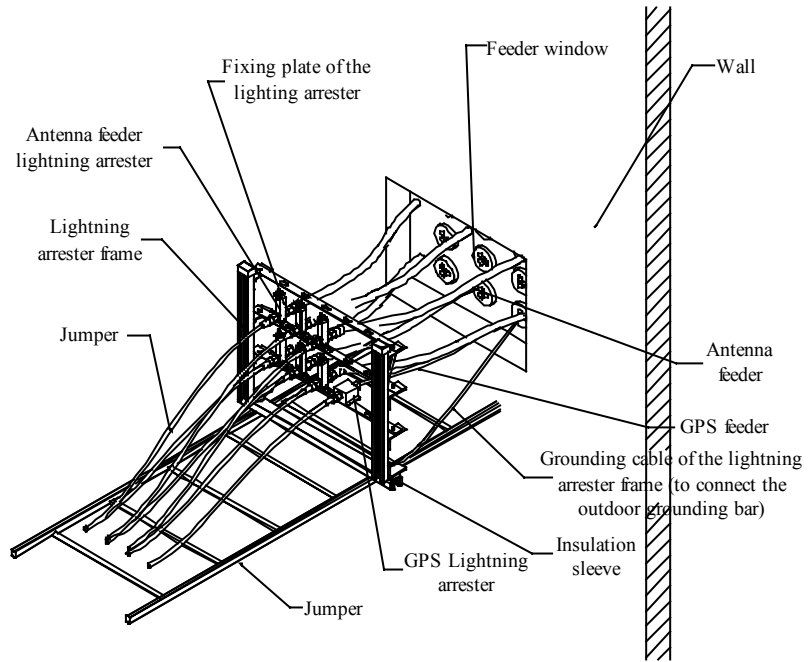
Fig. 6.2-4 Installing the Lightning Arrester Frame
