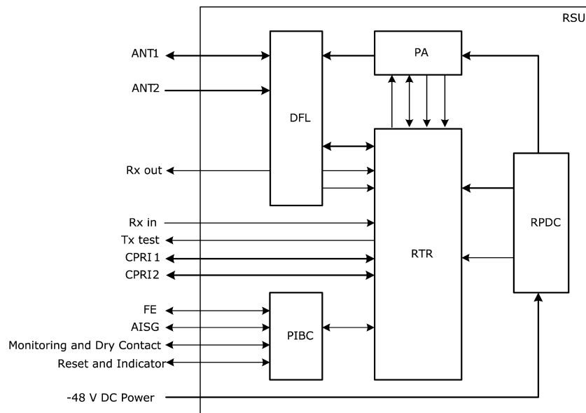
FIGURE 3 SCHEMATIC DIAGRAM OF THE ZXSDR RSUC
