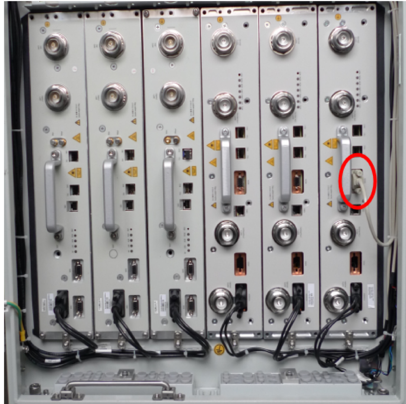
FIGURE 14 INSTALLING THE RSU MONITORING CABLE
