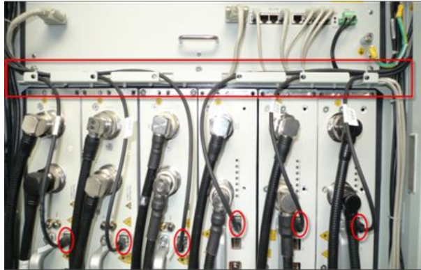
FIGURE 17 LAYOUT OF THE SFP CABLES IN THE RF CABINET
