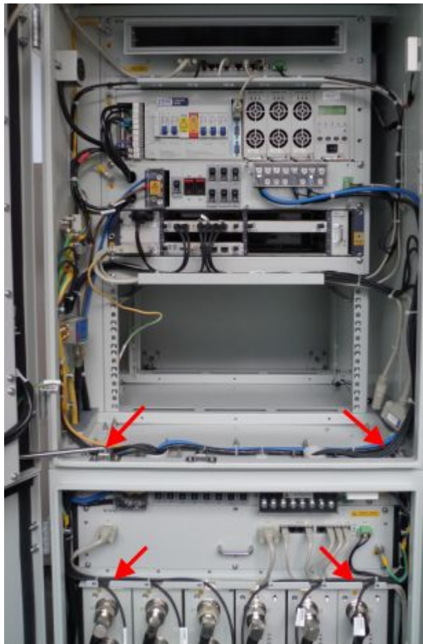
FIGURE 18 SFP CABLE LAYOUT
