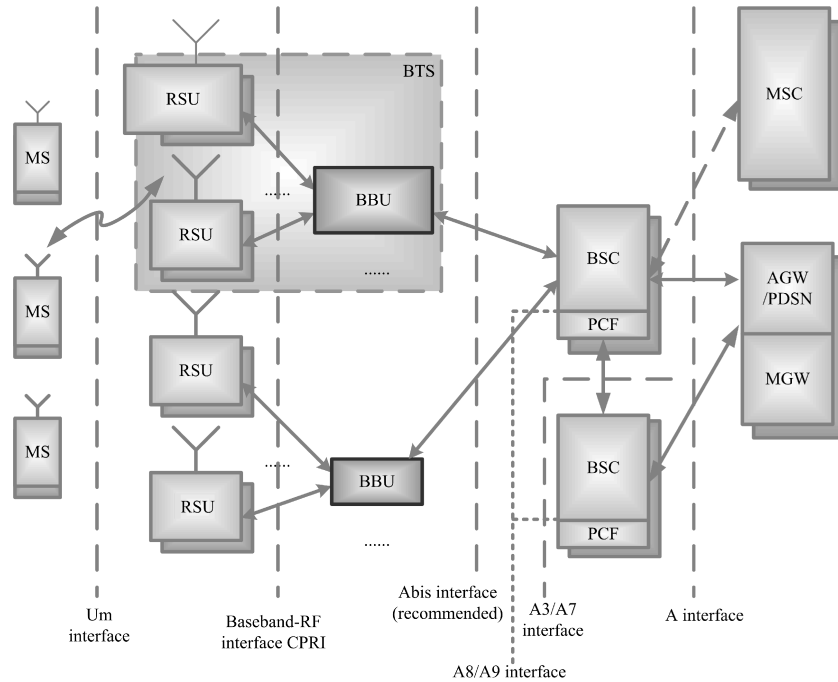
FIGURE 1 ZXSDR RSUC POSITION IN A NETWORK
