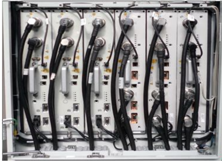
FIGURE 20 ANTENNA FEEDER JUMPER INSTALLED COMPLETELY
