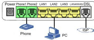
Figure 2-1 Cable Connection
