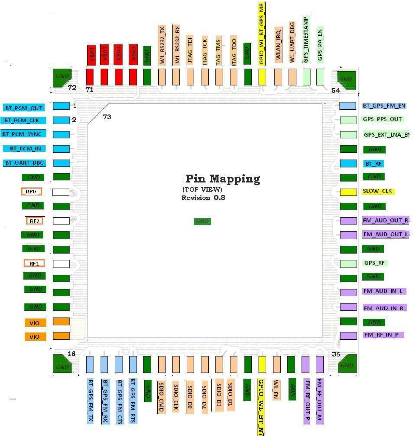
Figure 1 - Pin Map
