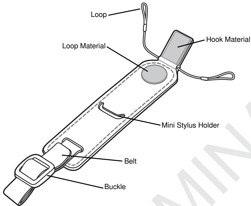
Figure 6-11 Handstrap
