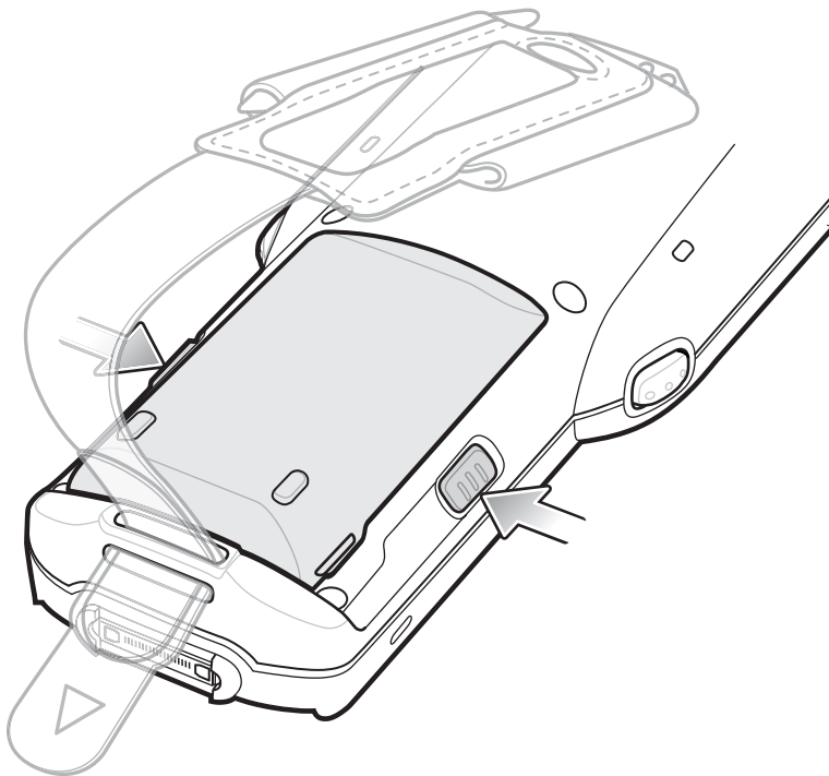
Figure 1-21 Release Battery
