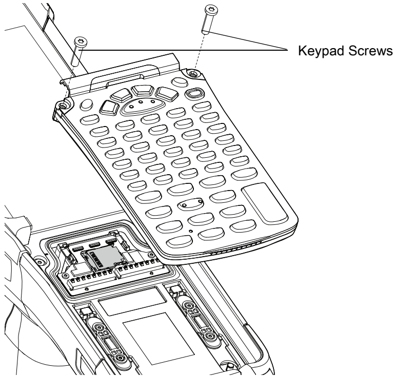
Figure 10 Replace Keypad
