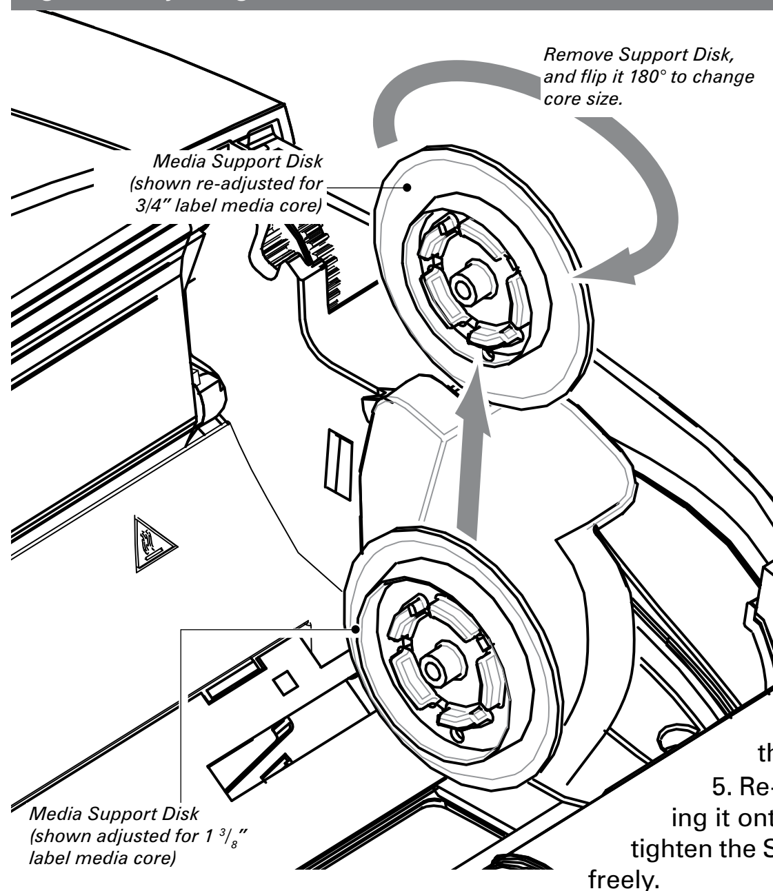
Figure 8- Adjusting the Media Core Diameter
