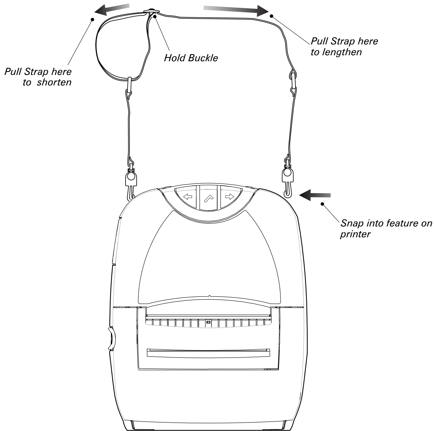
Figure 11- Shoulder Strap
