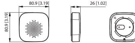
Figure 3-2 Dimensions (inch[mm])
