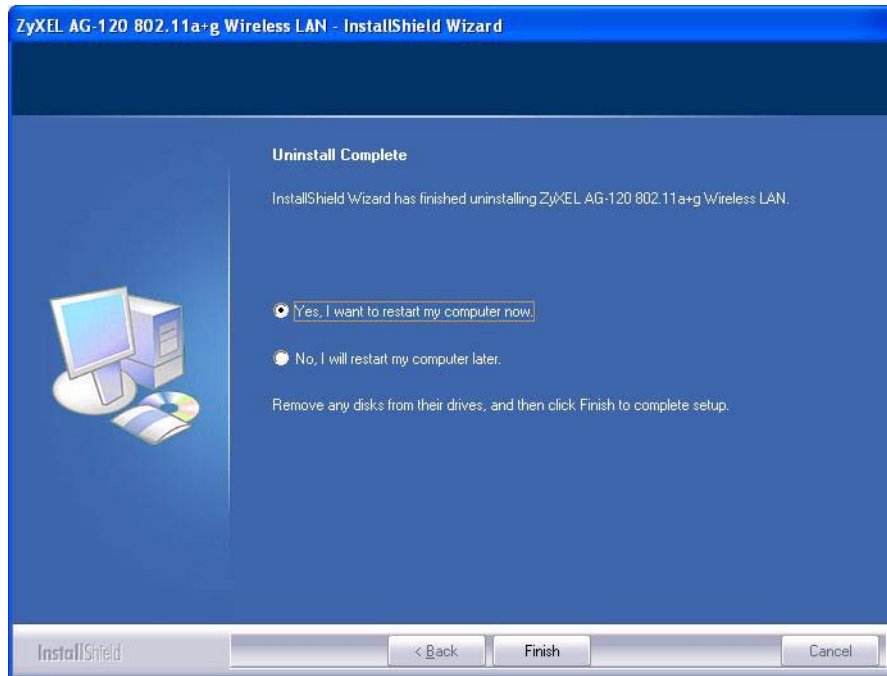
Figure 36 Uninstall: Finish
