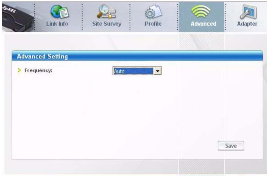
Figure 32 Advanced
