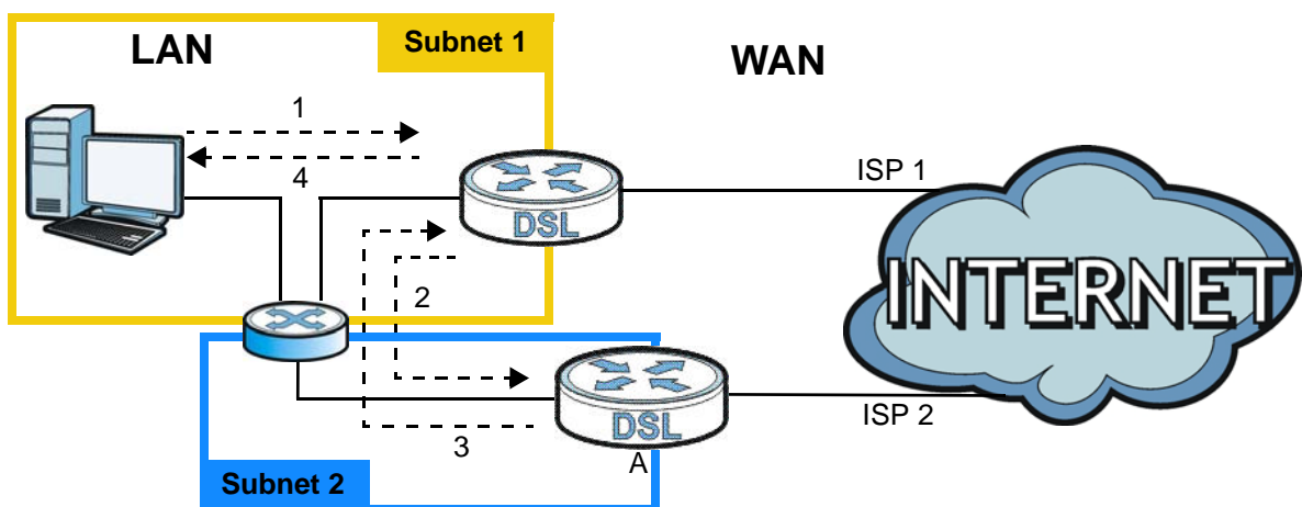
Figure 110 IP Alias
