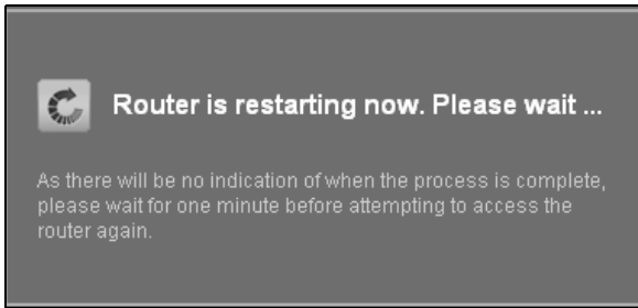
Figure 129 Firmware Uploading
