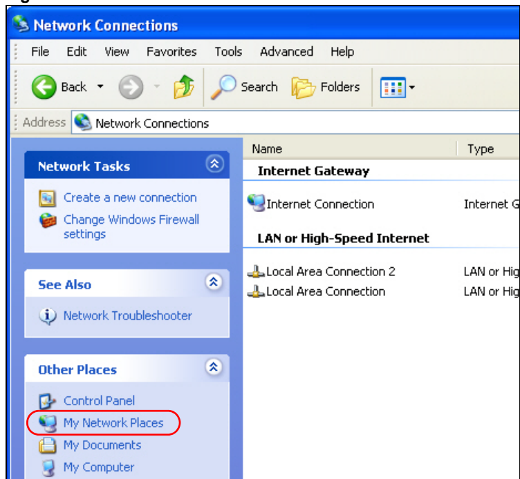
Figure 66 Network Connections
