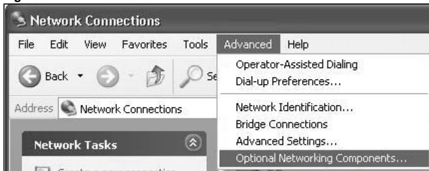
Figure 57 Network Connections
