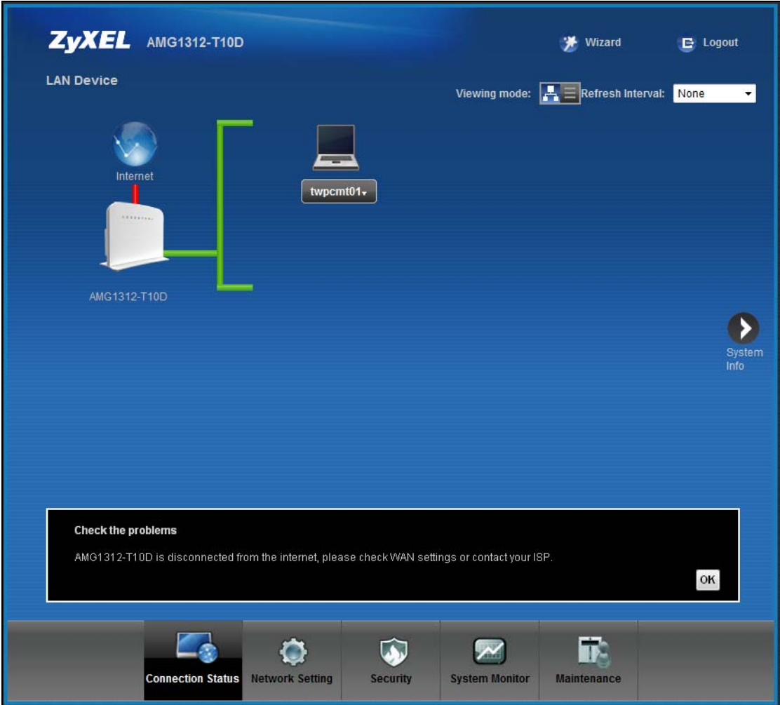
Figure 6 Connection Status
