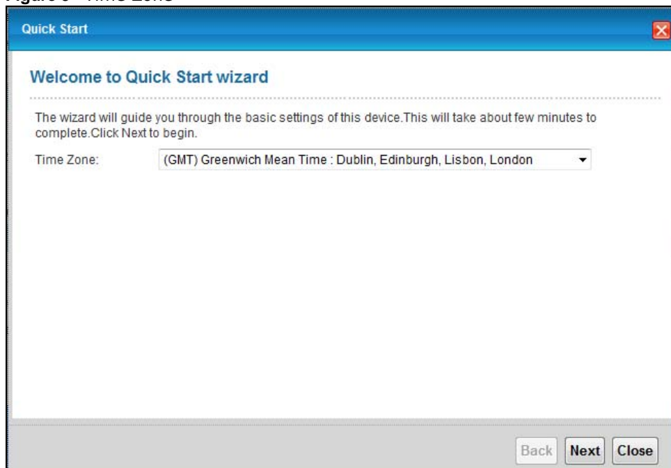
Figure 9 Time Zone
