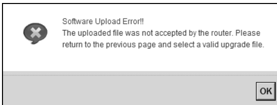
Figure 131 Error Message
