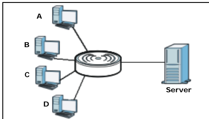
Figure 25 Multicast Example
