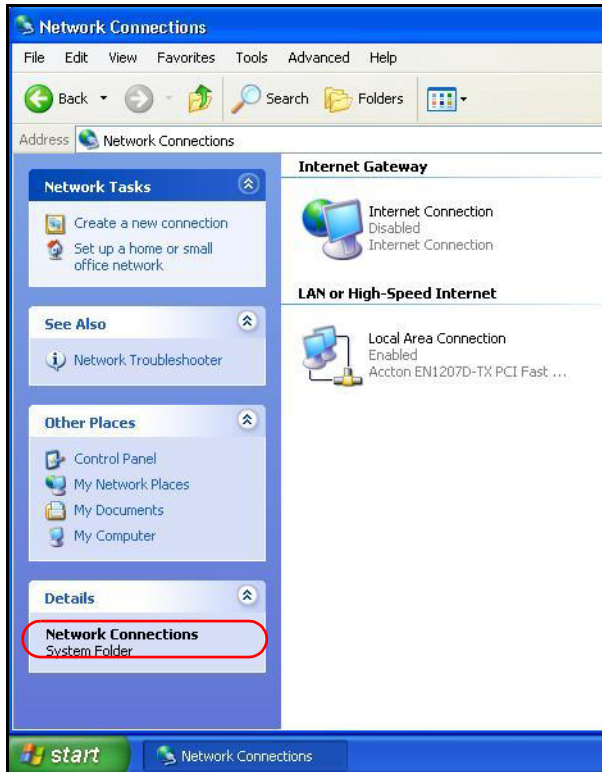
Figure 88 Network Connections
