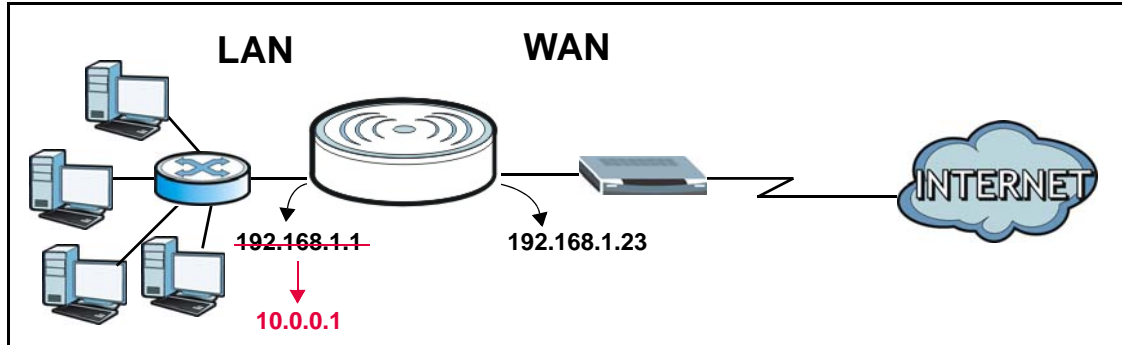
Figure 26 Auto-IP-Change
