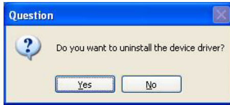
Figure 33 Uninstall: Confirm
