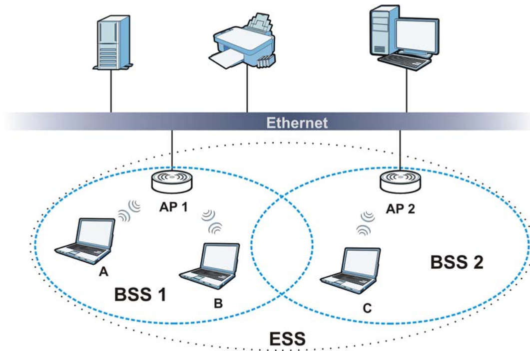
Figure 135 Infrastructure WLAN
