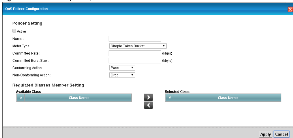
Figure 85 Policer Setup: Add/Edit
