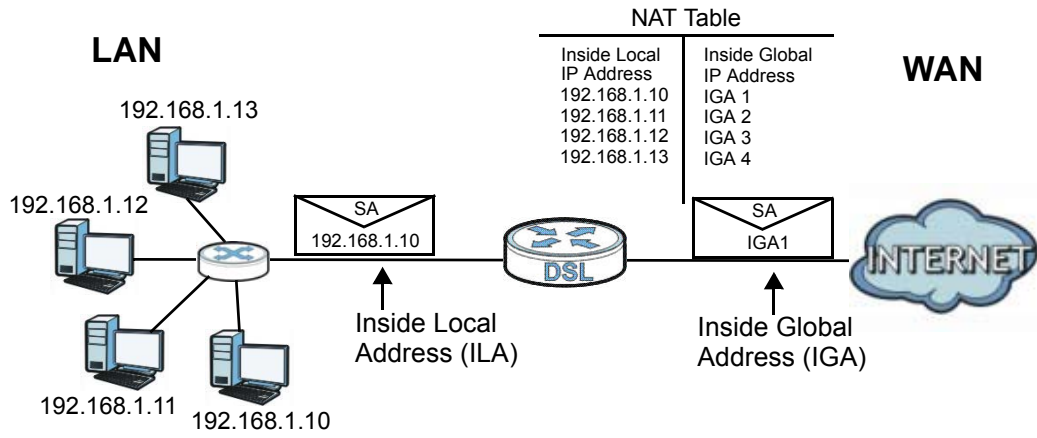
Figure 93 How NAT Works
