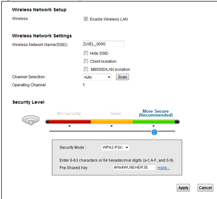
Figure 26 Network Setting > Wireless > General
