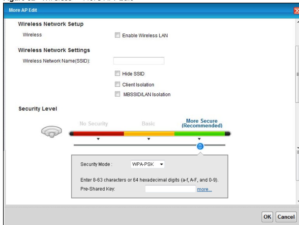
Figure 32 Wireless > More AP: Edit
