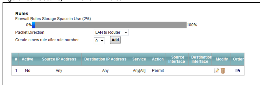
Figure 106 Security > Firewall > Rules
