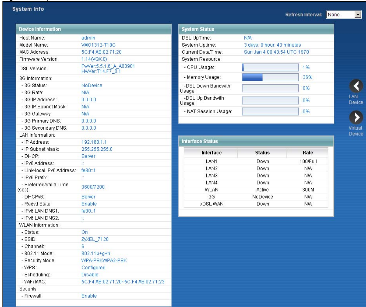
Figure 14 System Info Screen
