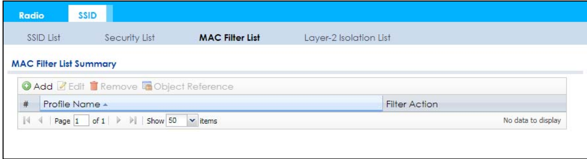
Figure 74 Configuration > Object > AP Profile > SSID > MAC Filter List
