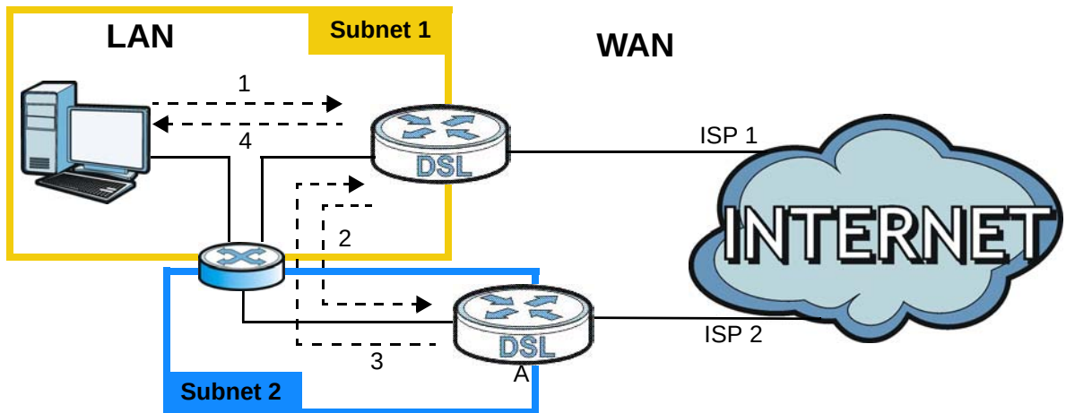
Figure 92 IP Alias
