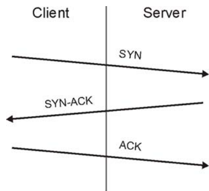
Figure 88 Three-Way Handshake
