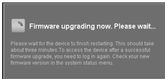
Figure 109 Firmware Uploading
