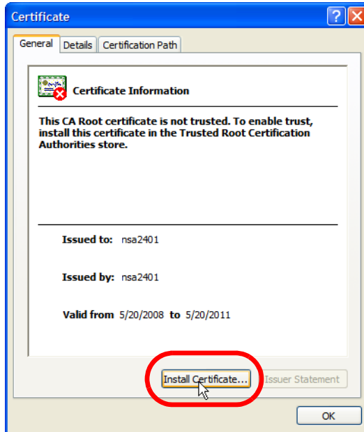
Figure 228 Internet Explorer 7: Certificate
