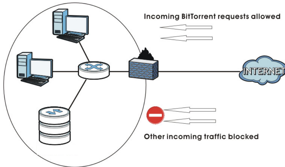
Figure 113 Firewall Configured to Allow Incoming BitTorrent Requests
