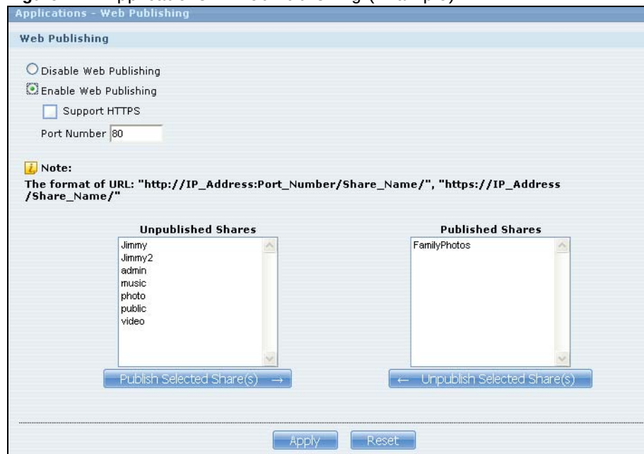
Figure 114 Applications > Web Publishing (Example)
