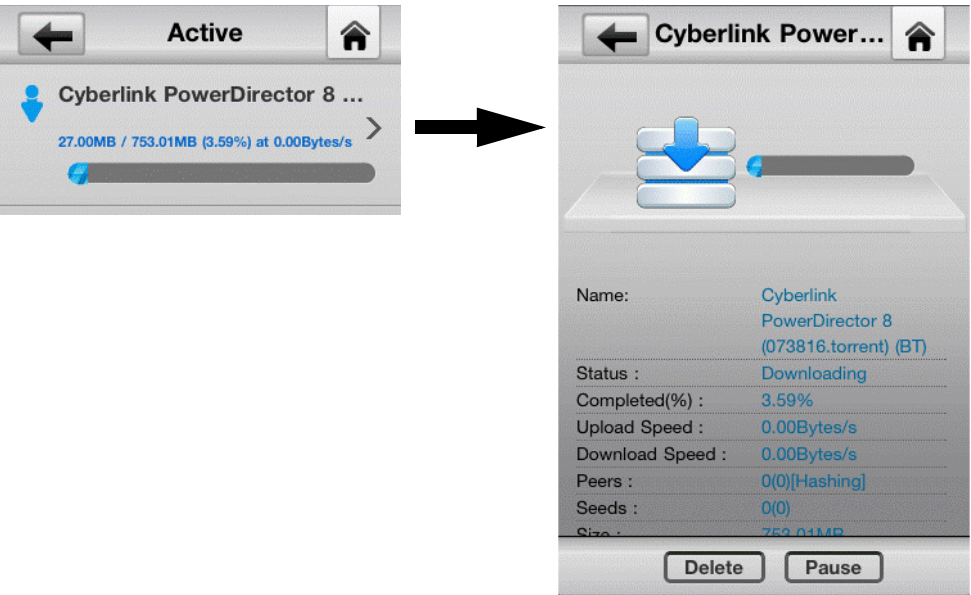
Figure 20 zMedia Download Service Active
