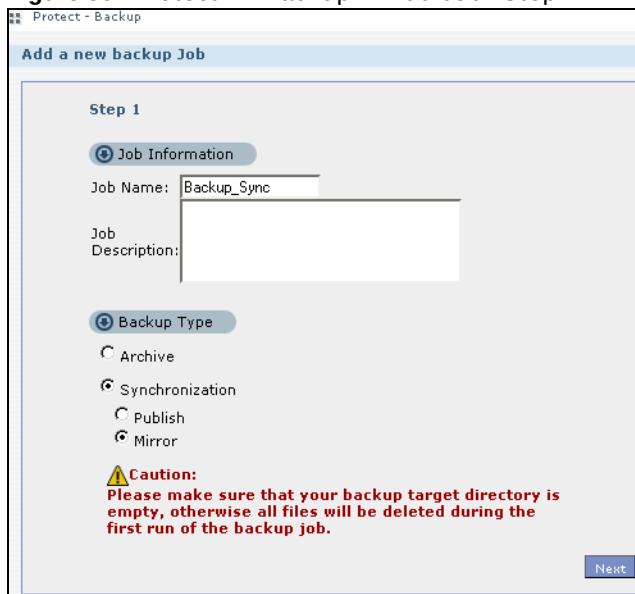
Figure 56 Protect &gt; Backup &gt; Add Job: Step 1
