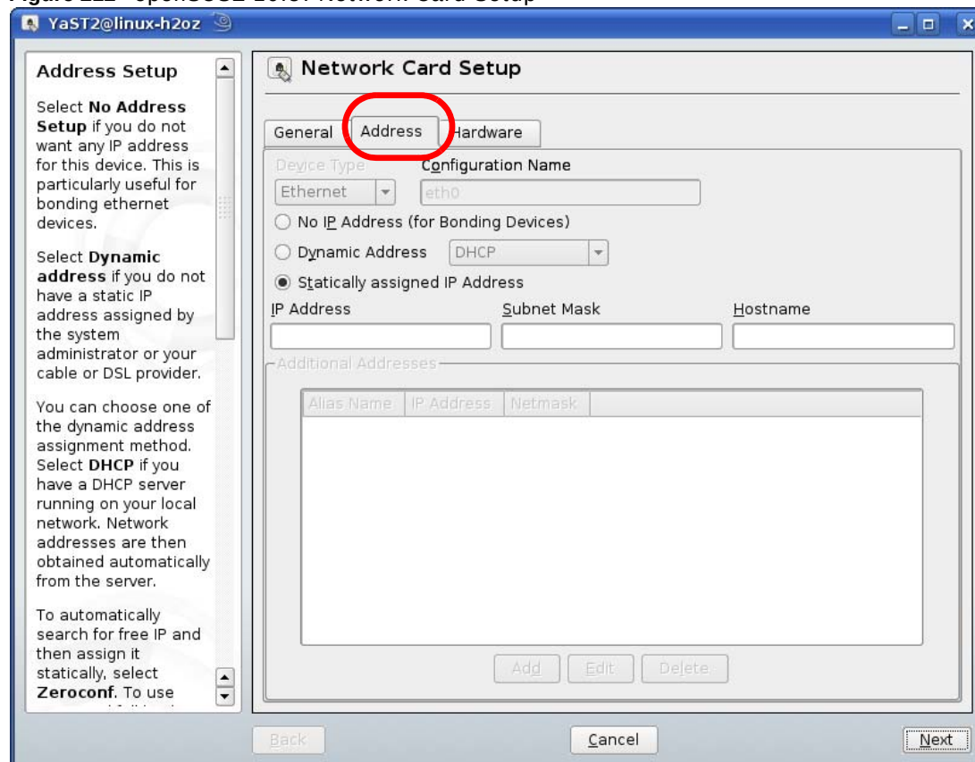
Figure 212 openSUSE 10.3: Network Card Setup
