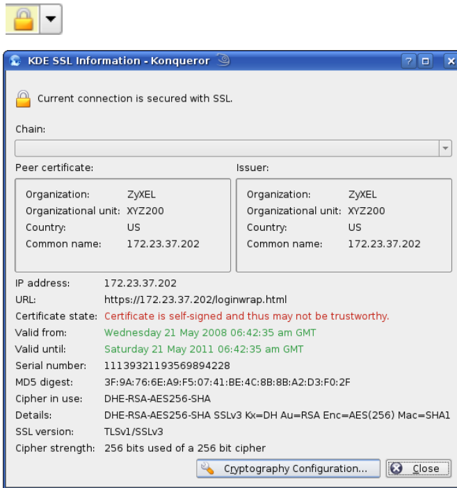
Figure 267 Konqueror 3.5: KDE SSL Information
