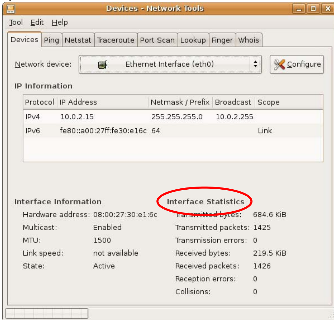
Figure 211 Ubuntu 8: Network Tools
