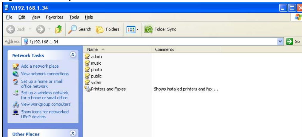
Figure 25 Directory
