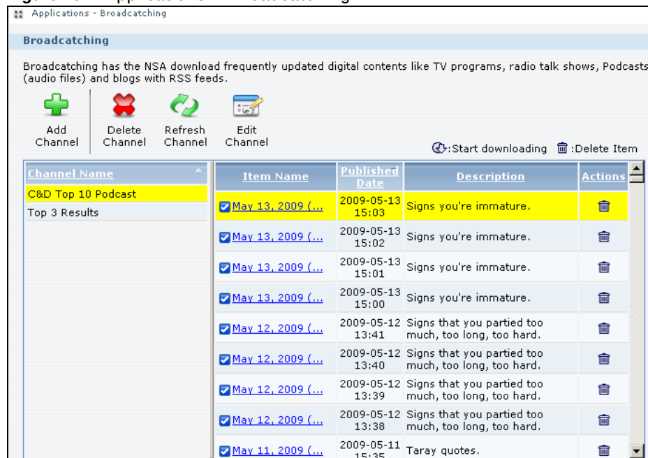
Figure 101 Applications > Broadcatching
