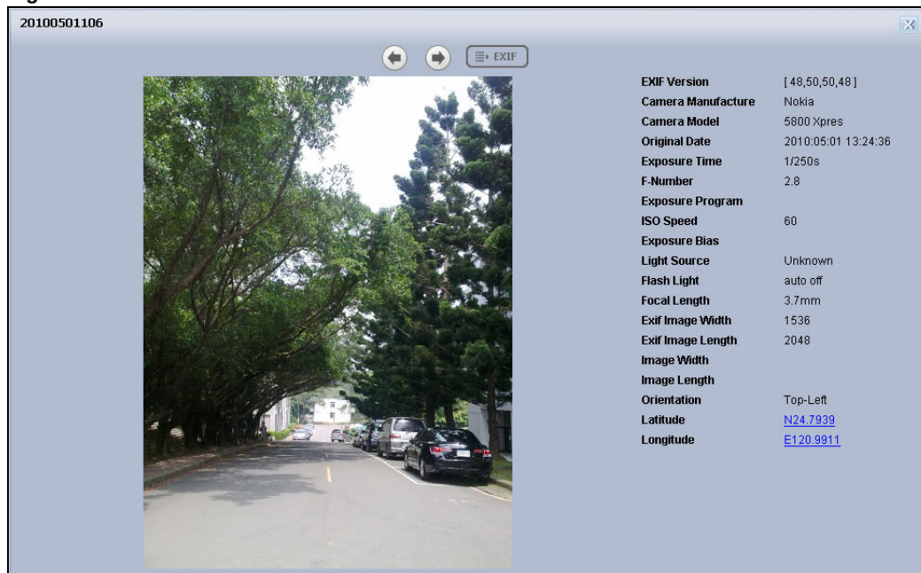
Figure 41 Exif Information
