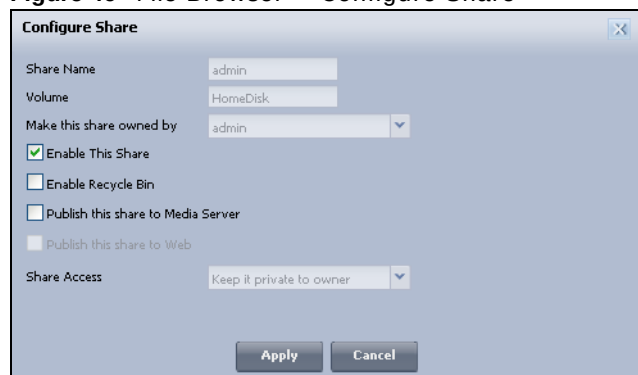
Figure 46 File Browser > Configure Share
