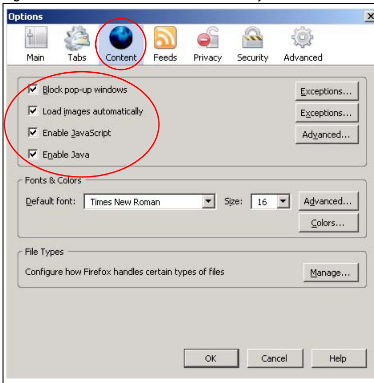
Figure 224 Mozilla Firefox Content Security
