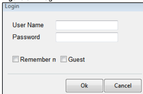
Figure 32 Login
