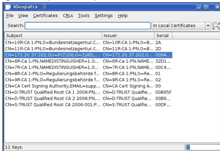
Figure 270 Konqueror 3.5: Kleopatra
