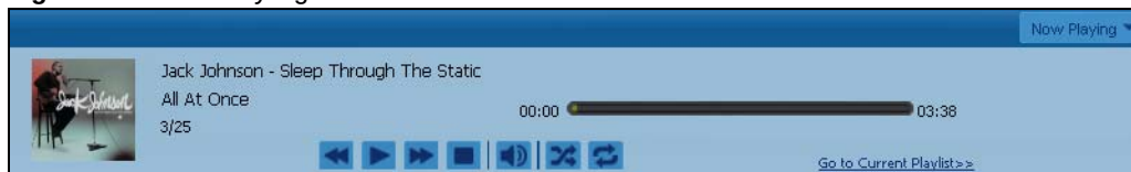
Figure 40 Now Playing
