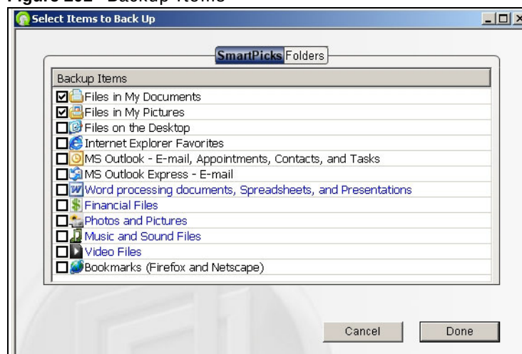
Figure 201 Backup Items
