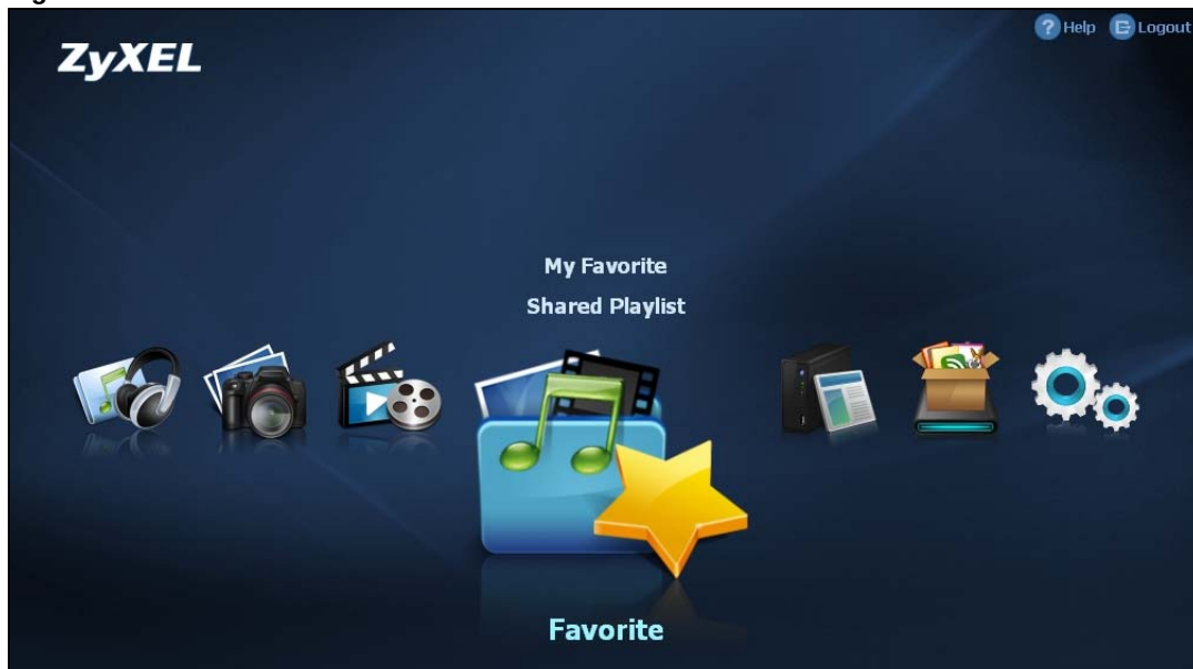
Figure 38 Home
