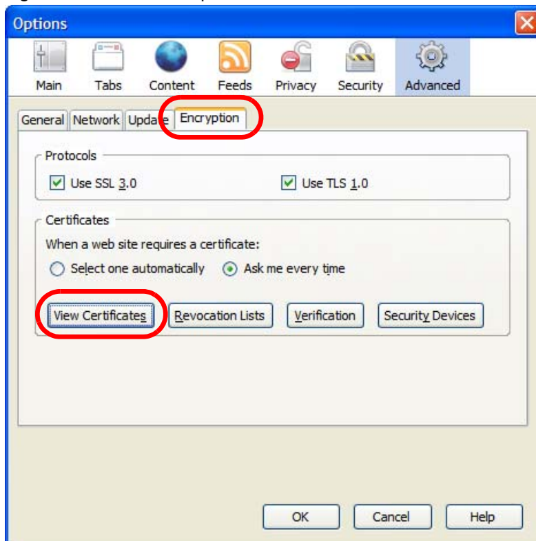
Figure 251 Firefox 2: Options
