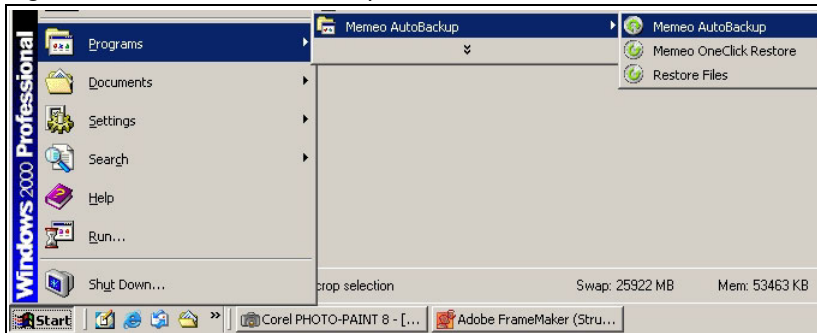
Figure 204 Memeo Autobackup
