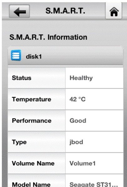
Figure 15 zMedia S.M.A.R.T.
