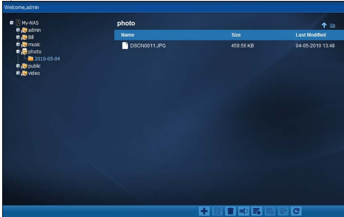
Figure 45 File Browser
