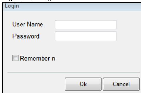
Figure 26 Login
