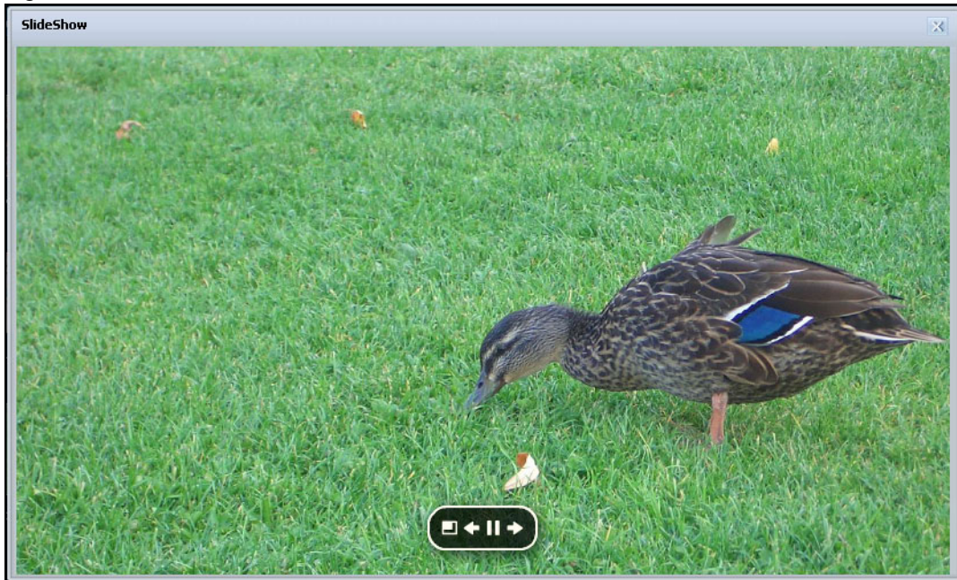
Figure 43 Slideshow
