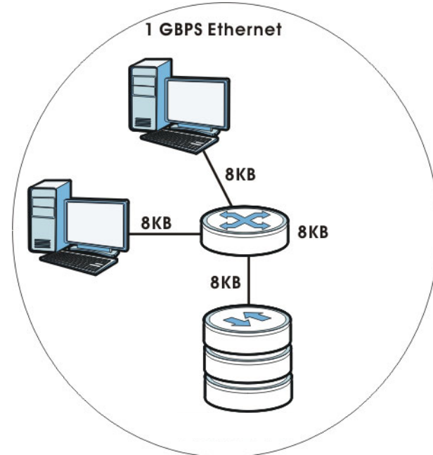
Figure 79 Jumbo Frames
