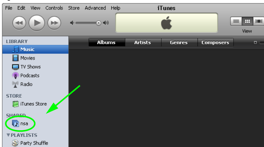
Figure 208 iTunes Reconnected
