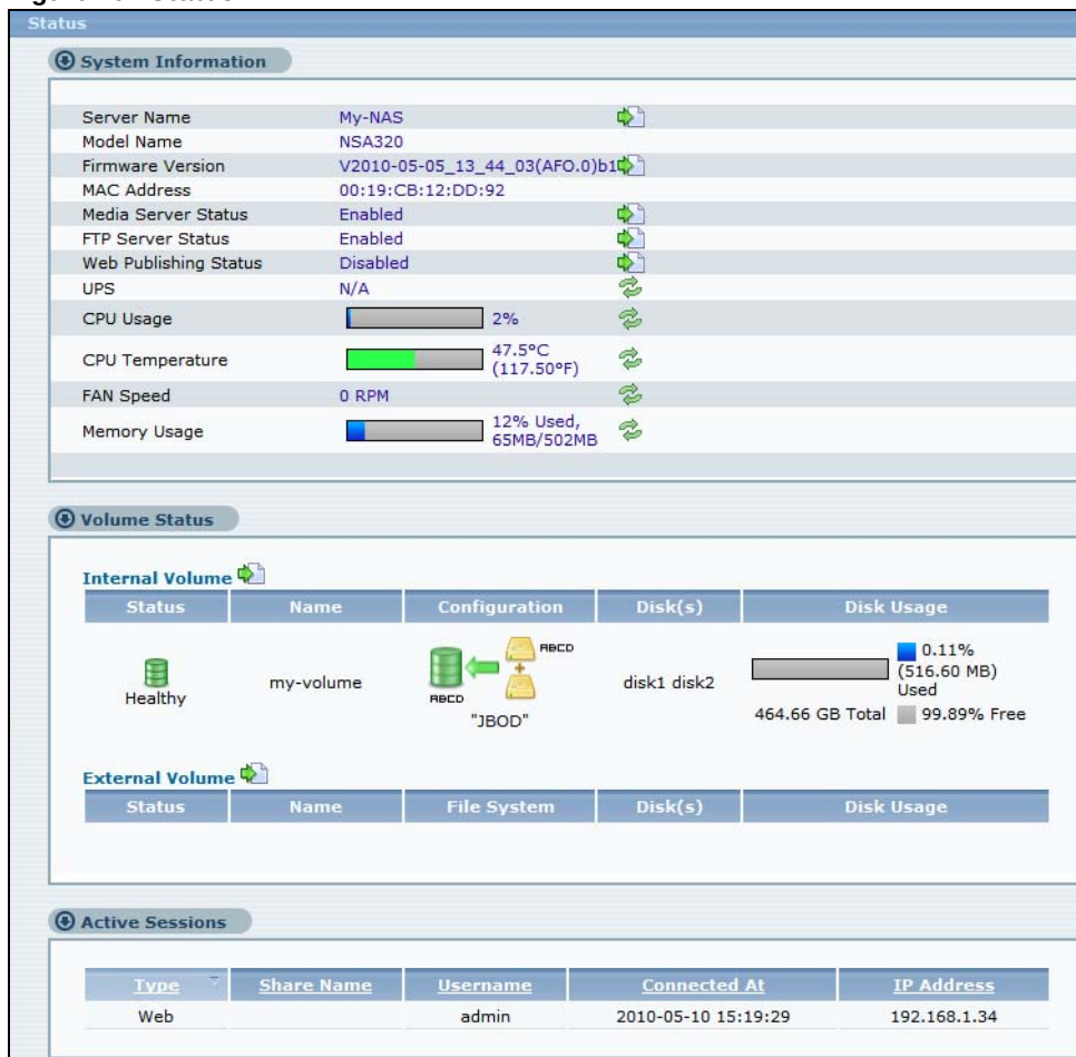
Figure 70 Status
