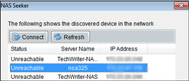
Figure 22 NAS Seeker
