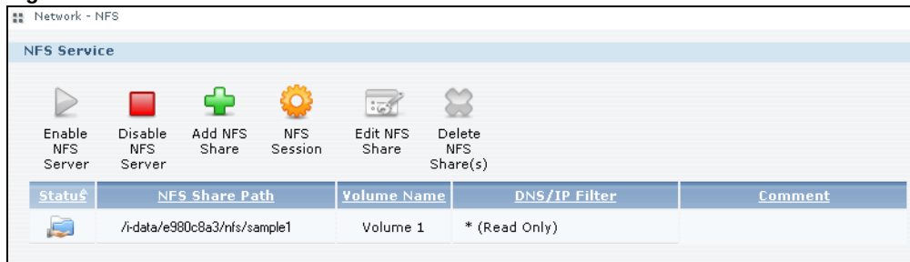
Figure 124 Network > NFS
