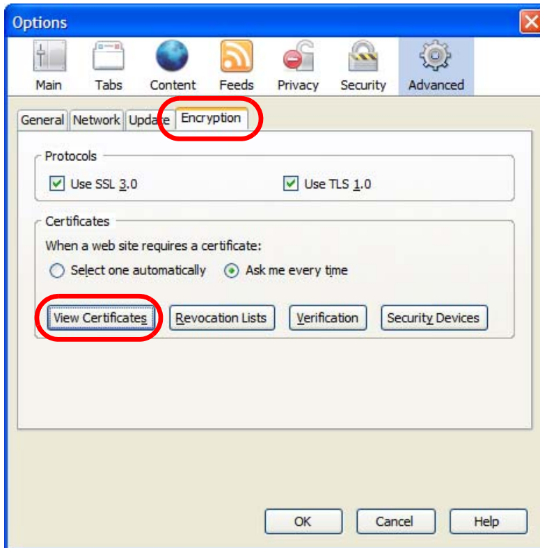
Figure 247 Firefox 2: Options
