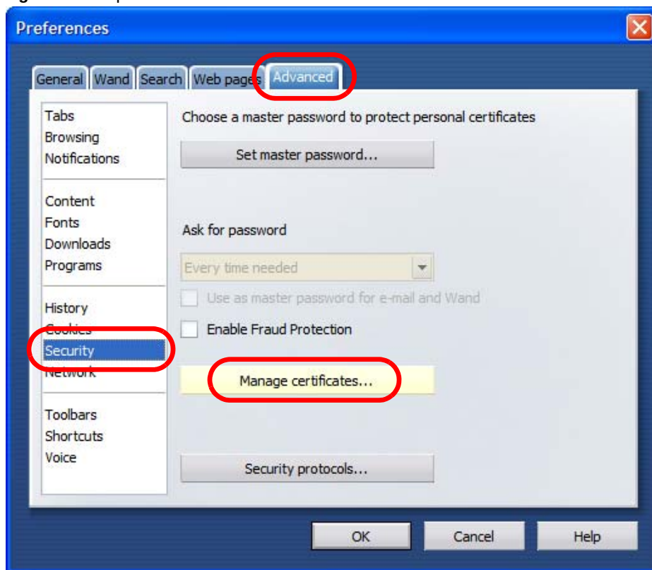
Figure 263 Opera 9: Preferences
