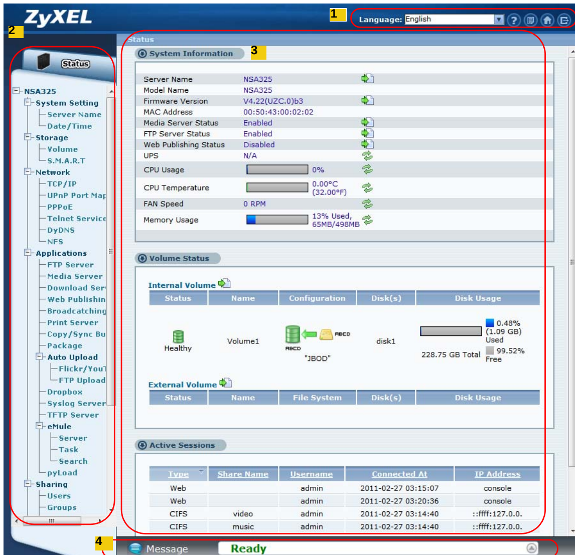
Figure 49 Status
