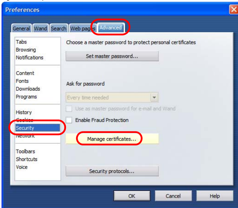
Figure 257 Opera 9: Preferences
