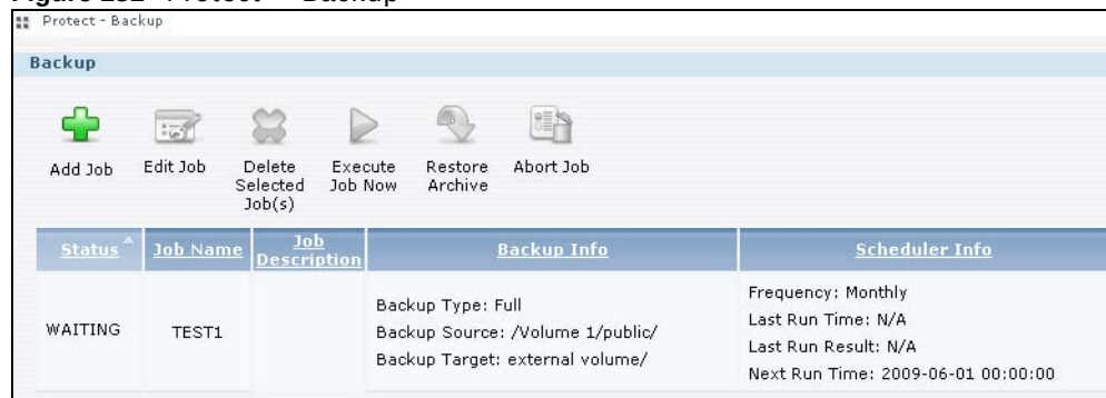
Figure 131 Protect > Backup
