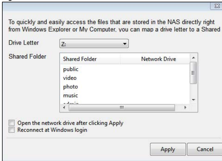
Figure 31 Network Drive
