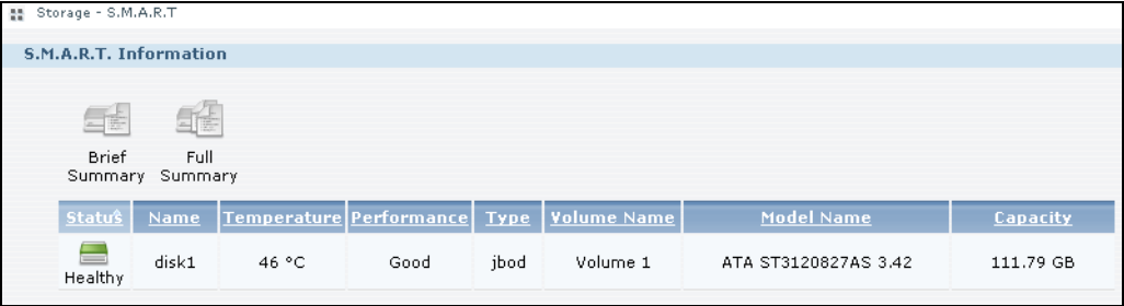
Figure 128 Storage > S.M.A.R.T
