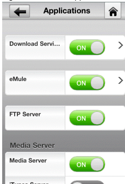
Figure 18 zMedia Applications
