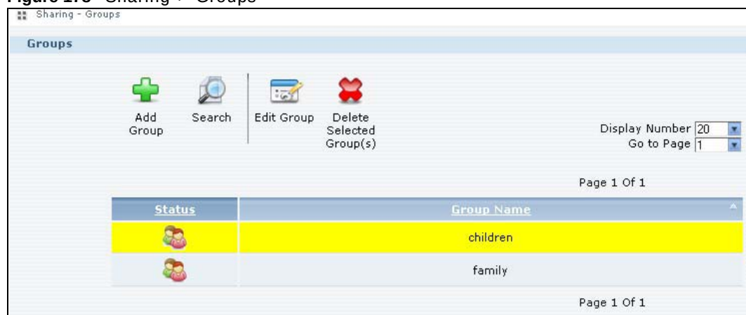
Figure 178 Sharing > Groups
