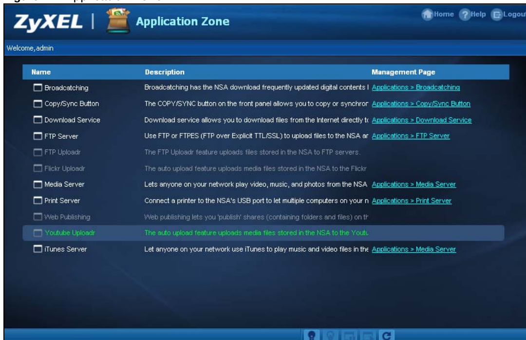
Figure 47 Application Zone
