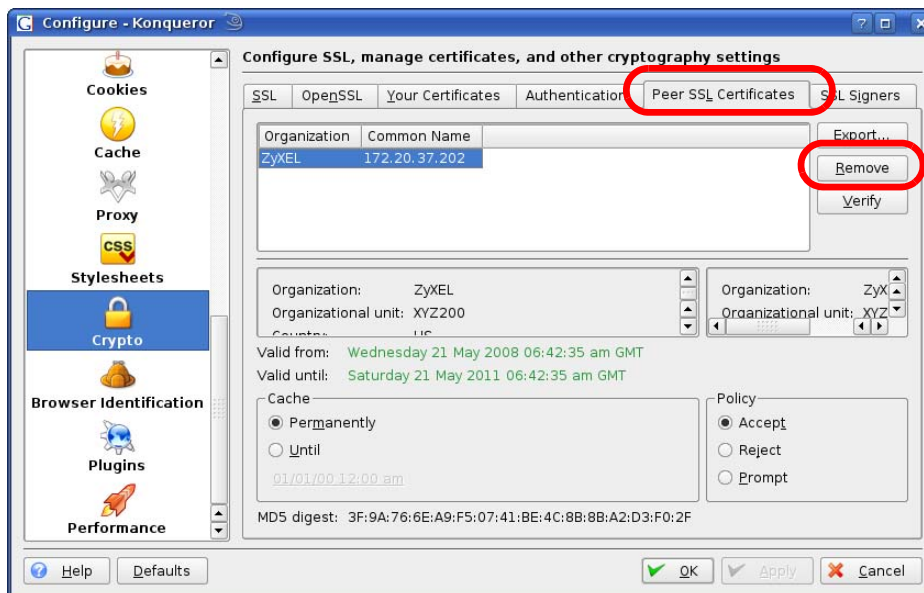
Figure 272 Konqueror 3.5: Configure
