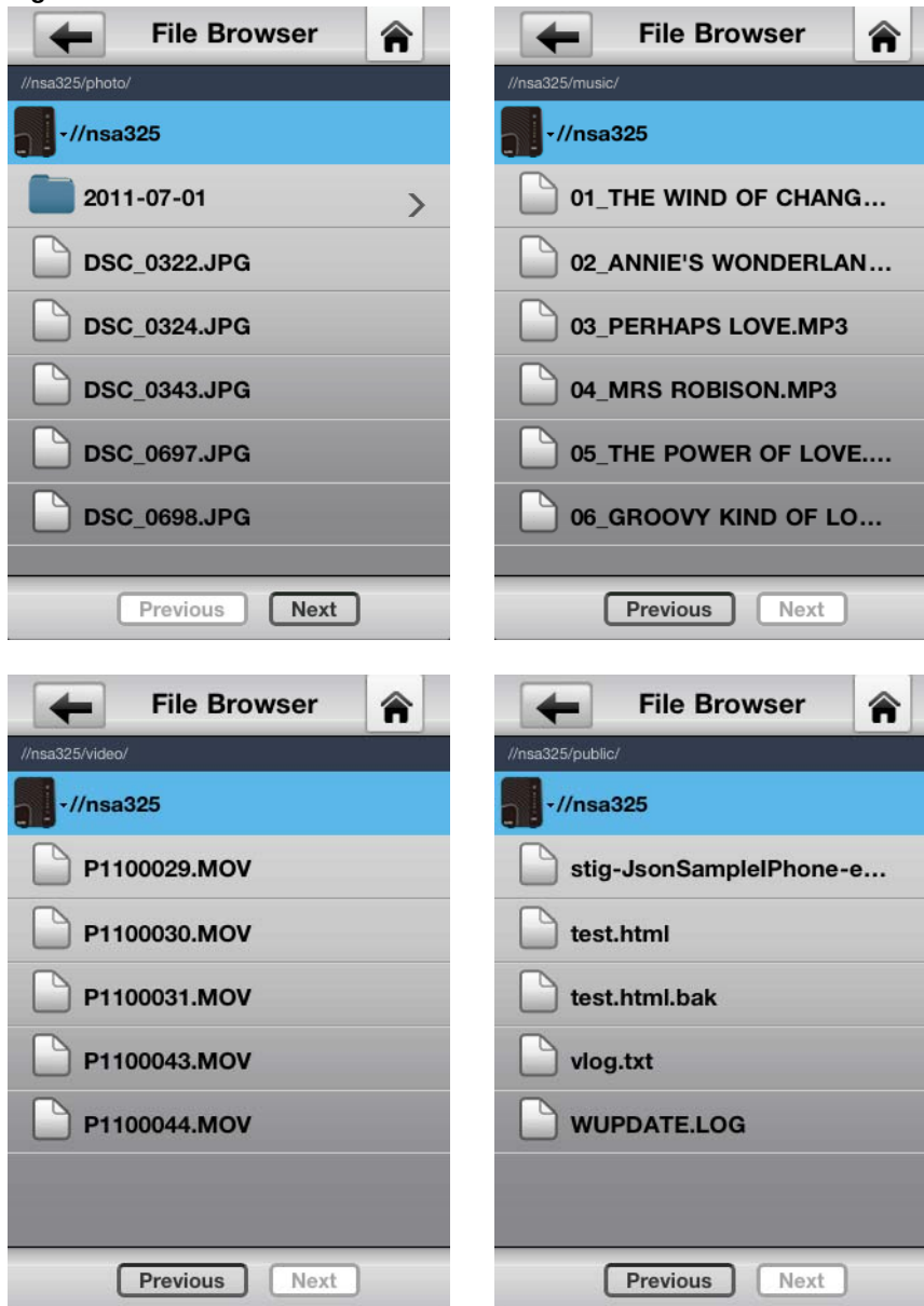
Figure 8 zMedia Shares
