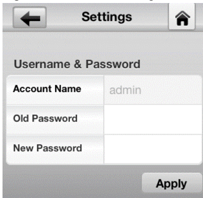
Figure 11 zMedia Settings
