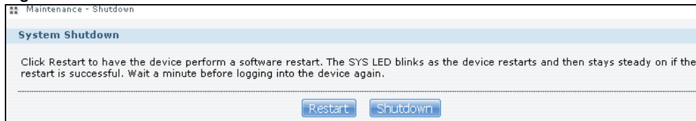
Figure 196 Maintenance > Shutdown
