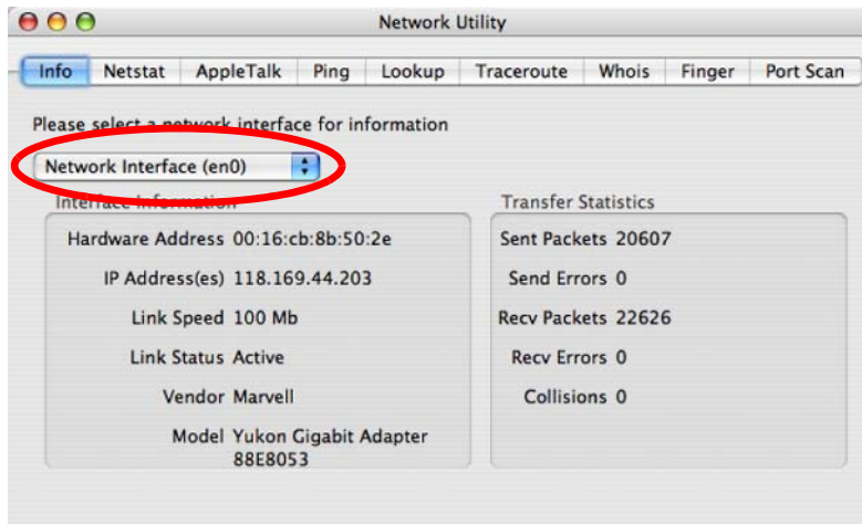
Figure 209 Mac OS X 10.4: Network Utility
