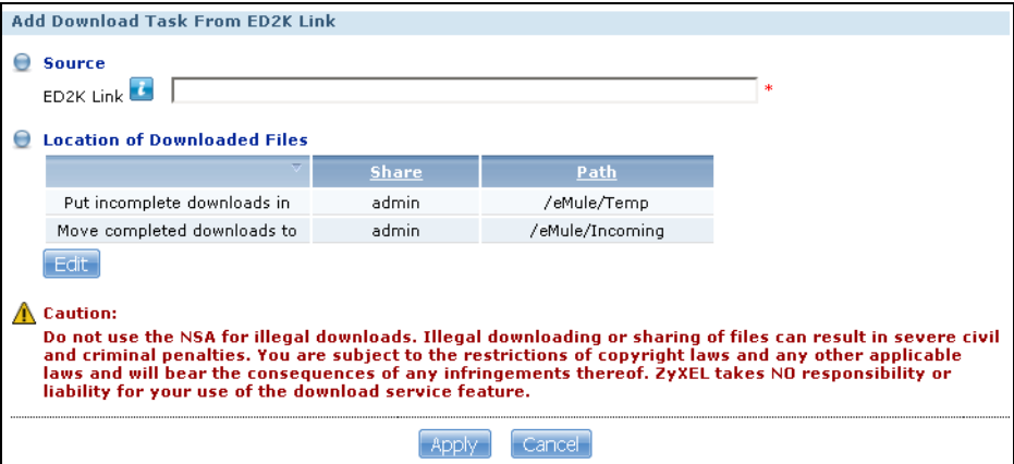
Figure 154 Applications > eMule > Task: Add
