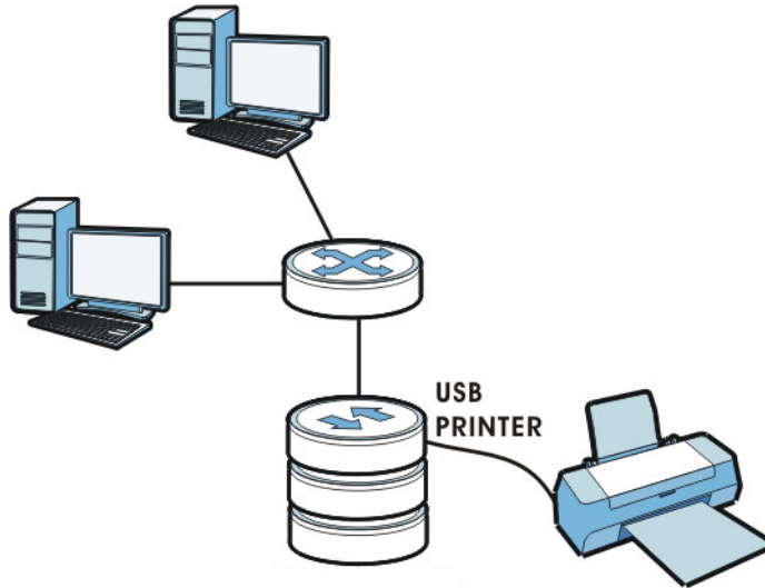
Figure 117 Printer Sharing
