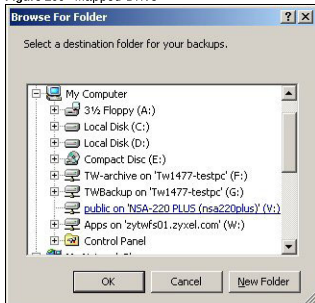
Figure 200 Mapped Drive
