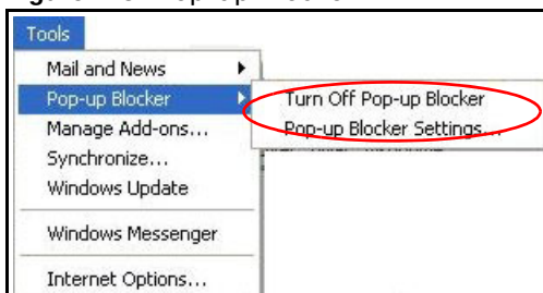
Figure 215 Pop-up Blocker
