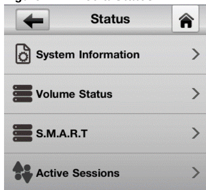
Figure 12 zMedia Status
