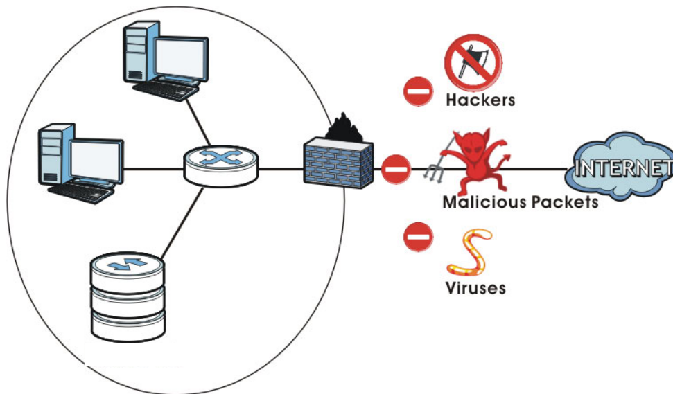
Figure 111 Firewall
