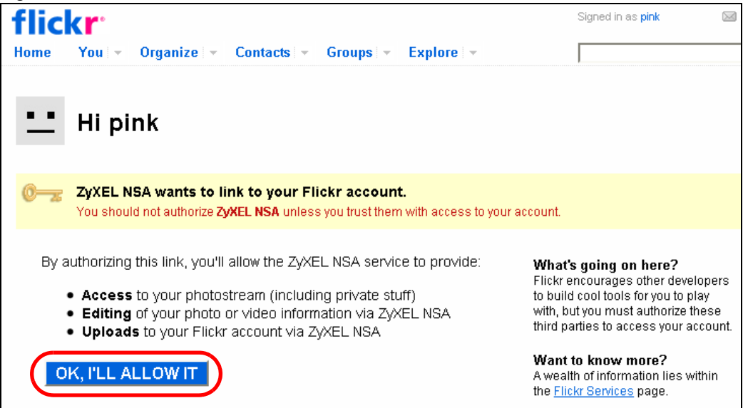
Figure 164 Flickr Authorization
