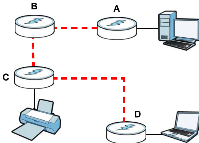
Figure 11 Removing Devices From an Existing Powerline Network
