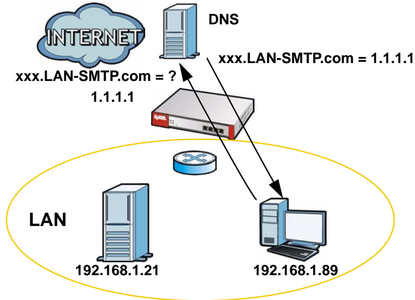
Figure 197 LAN Computer Queries a Public DNS Server
