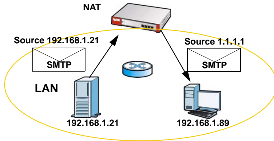
Figure 199 LAN to LAN Return Traffic
