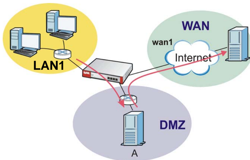
Figure 200 HTTP Redirect Example
