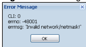
Figure 15 Warning Message
