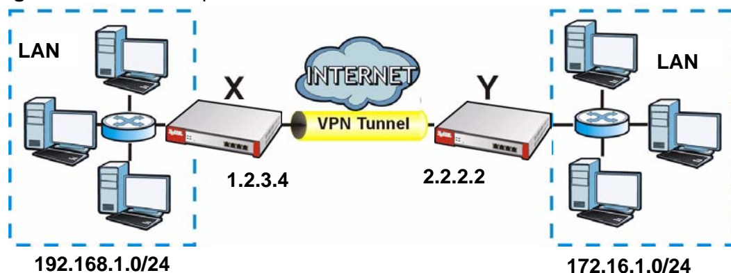
Figure 68 VPN Example
