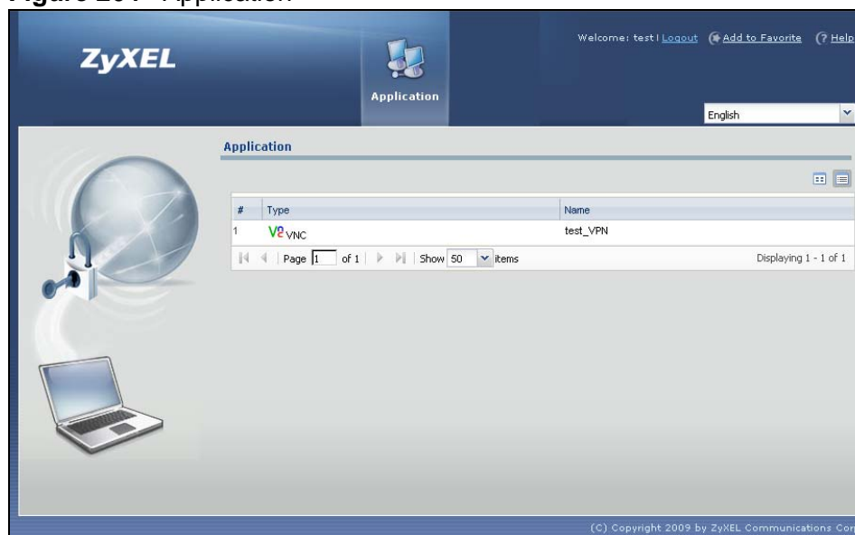
Figure 264 Application
