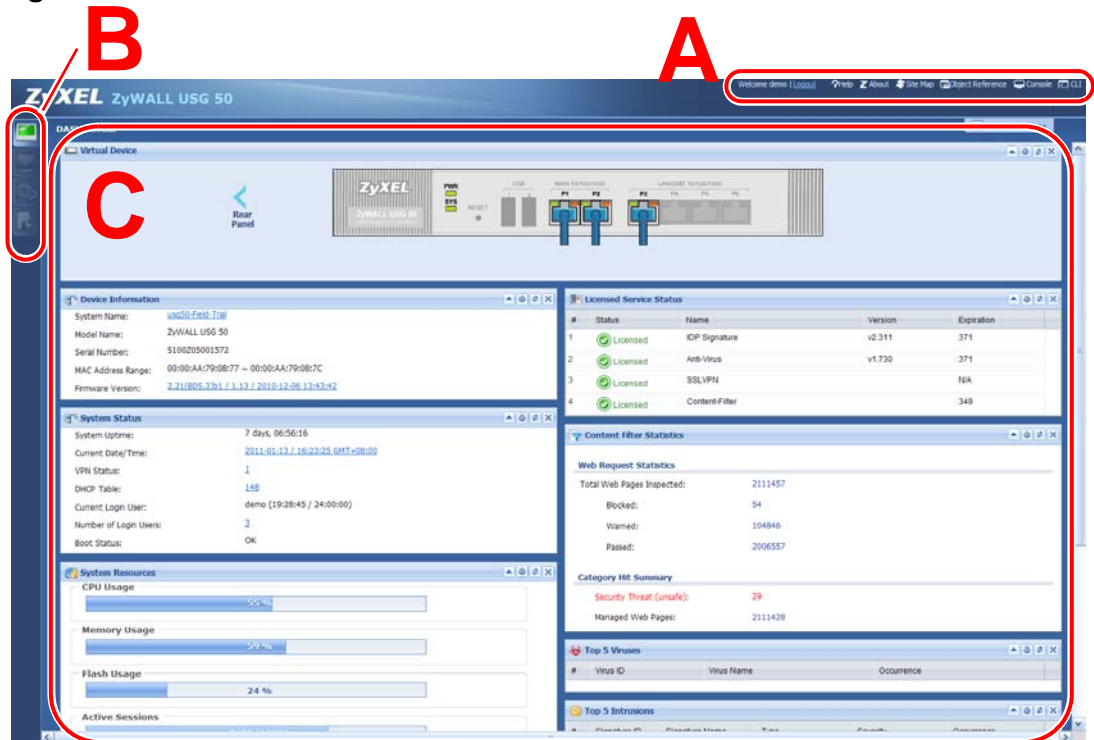
Figure 11 Dashboard
