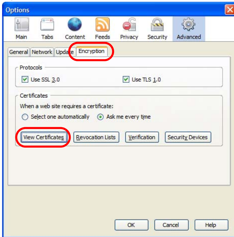
Figure 500 Firefox 2: Options
