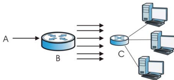
Figure 311 Smurf Attack
