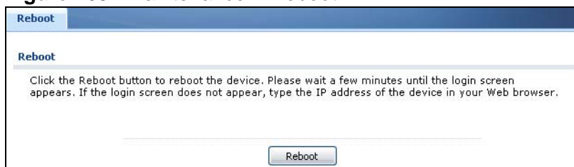
Figure 465 Maintenance > Reboot
