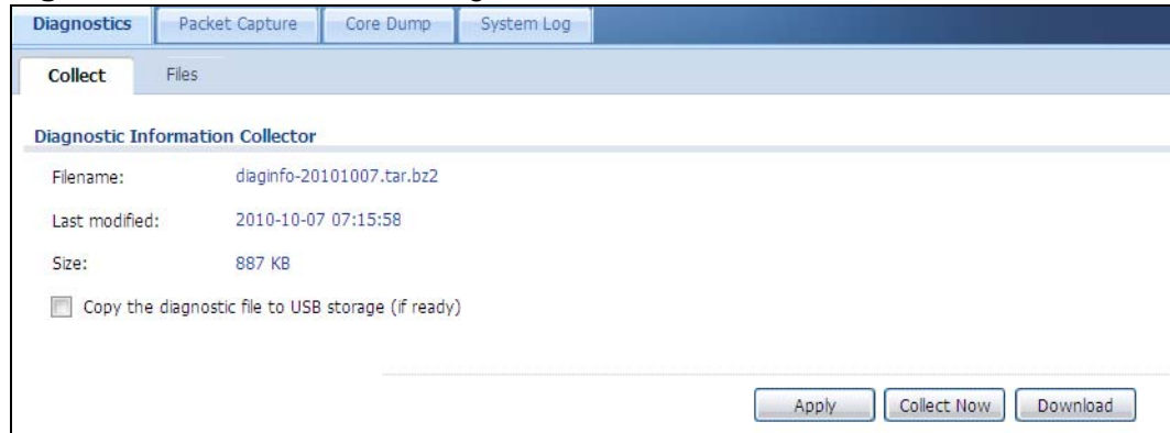
Figure 445 Maintenance > Diagnostics
