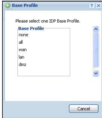
Figure 292 Base Profiles
