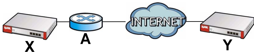
Figure 240 VPN/NAT Example
