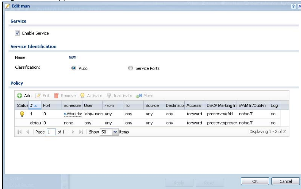
Figure 280 Application Edit
