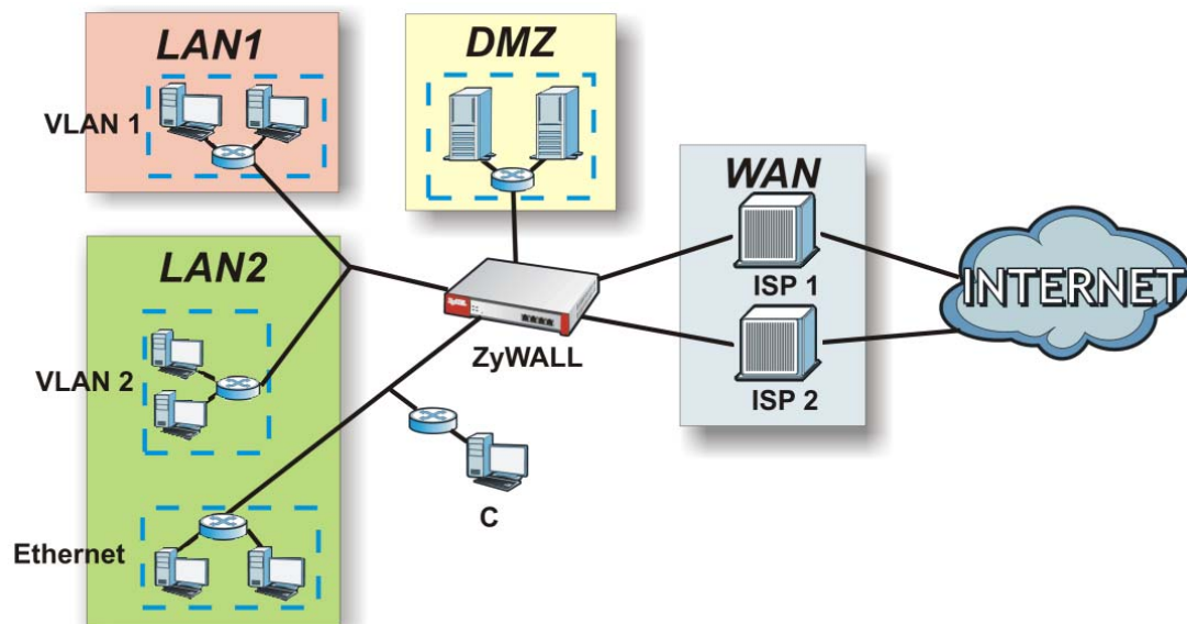
Figure 190 Example: Zones
