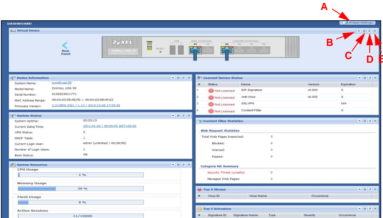
Figure 115 Dashboard
