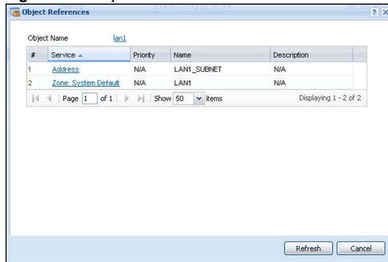
Figure 157 Object References
