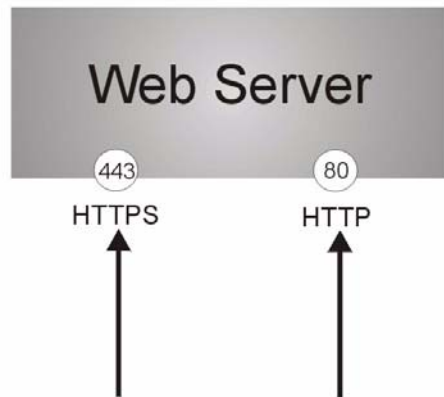
Figure 395 HTTP/HTTPS Implementation
