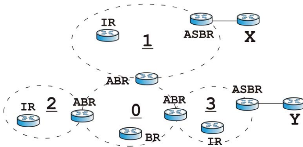
Figure 185 OSPF: Types of Routers
