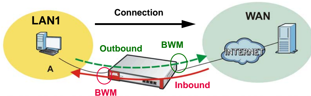
Figure 270 LAN1 to WAN Connection and Packet Directions
