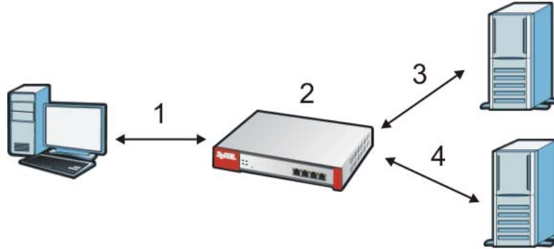
Figure 320 Content Filter Lookup Procedure
