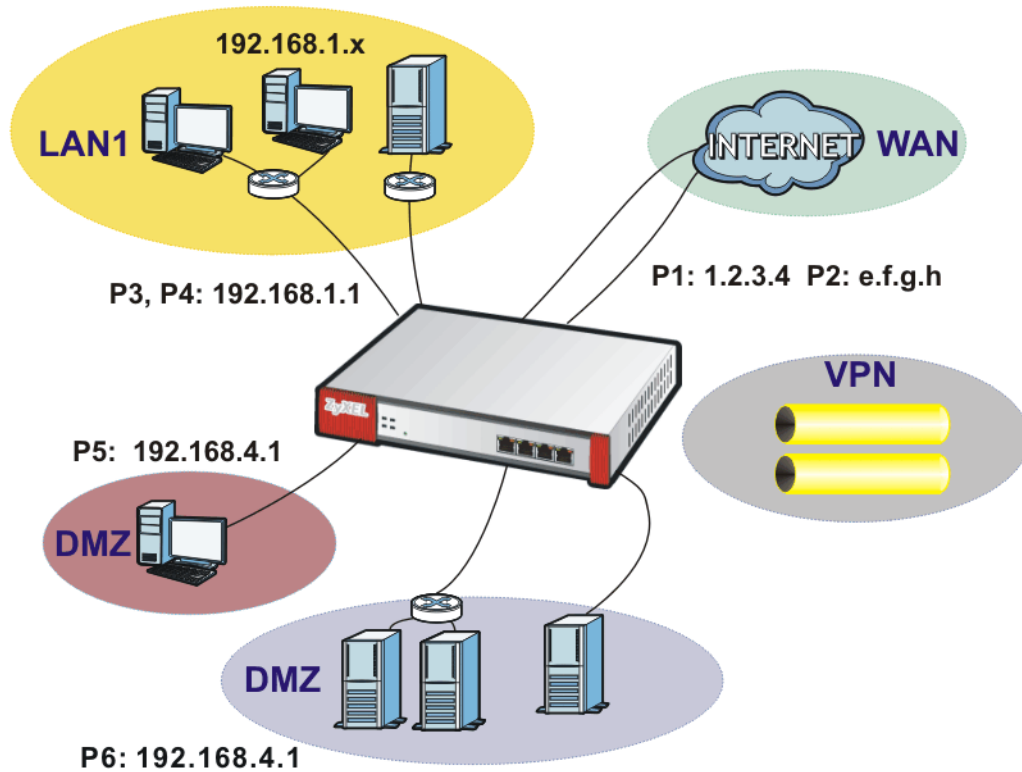
Figure 56 Ethernet Interface, Port Roles, and Zone Configuration Example
