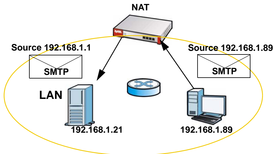
Figure 198 LAN to LAN Traffic
