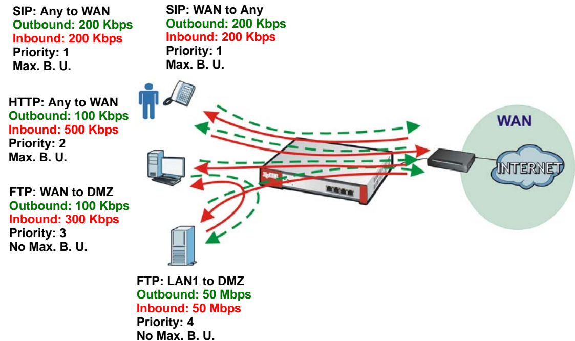
Figure 273 Application Patrol Bandwidth Management Example
