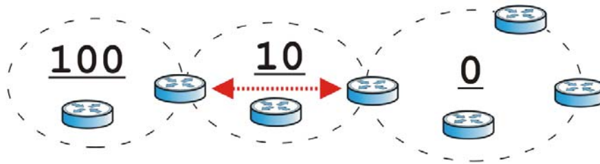
Figure 186 OSPF: Virtual Link
