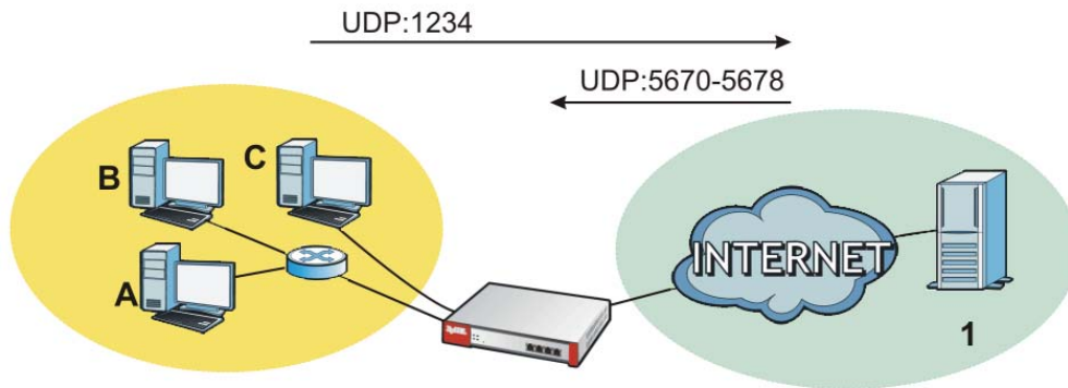
Figure 182 Trigger Port Forwarding Example
