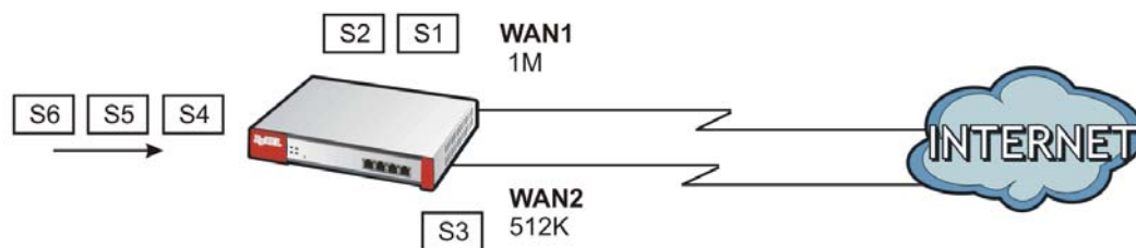
Figure 174 Spillover Algorithm Example
