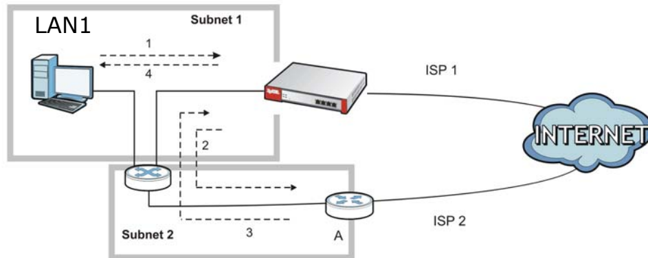
Figure 225 Using Virtual Interfaces to Avoid Asymmetrical Routes
