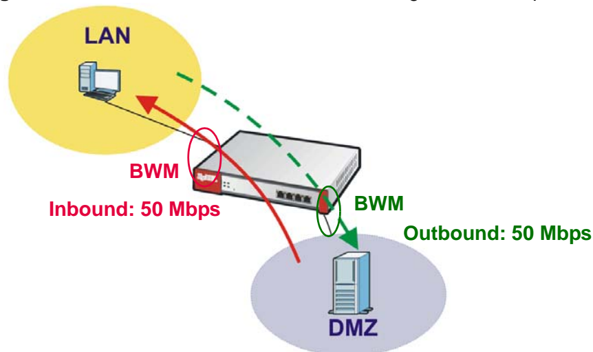
Figure 277 FTP LAN to DMZ Bandwidth Management Example
