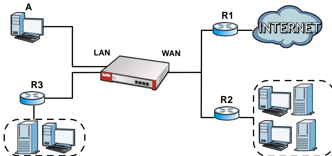
Figure 177 Example of Policy Routing Topology
