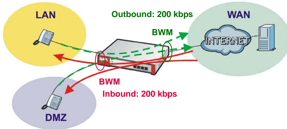
Figure 274 SIP Any to WAN Bandwidth Management Example
