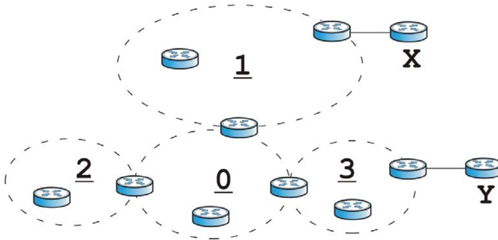
Figure 184 OSPF: Types of Areas
