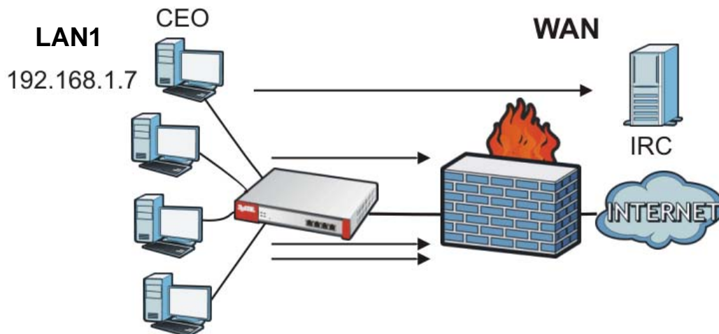
Figure 219 Limited LAN to WAN IRC Traffic Example
