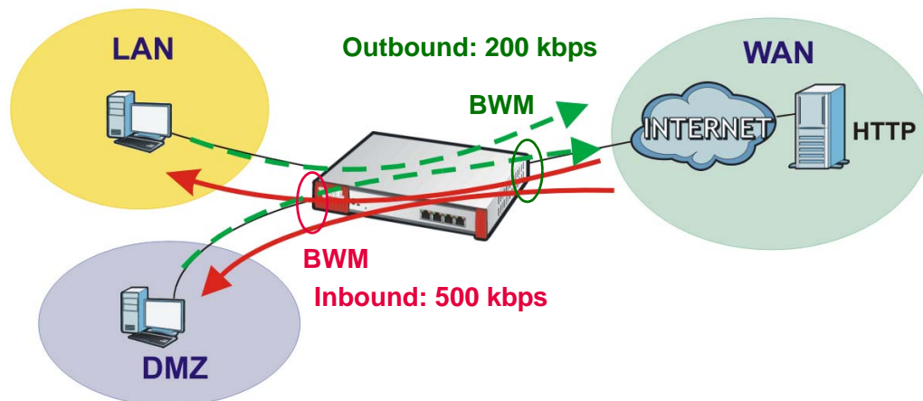
Figure 275 HTTP Any to WAN Bandwidth Management Example
