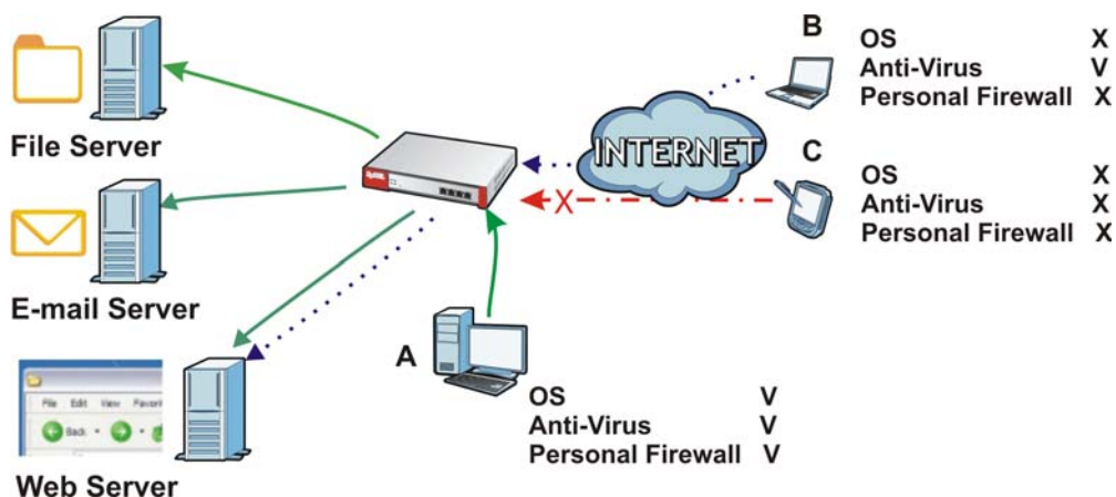
Figure 382 Endpoint Security
