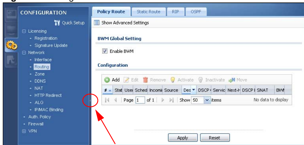
Figure 14 Navigation Panel
