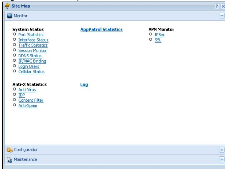
Figure 16 Site Map
