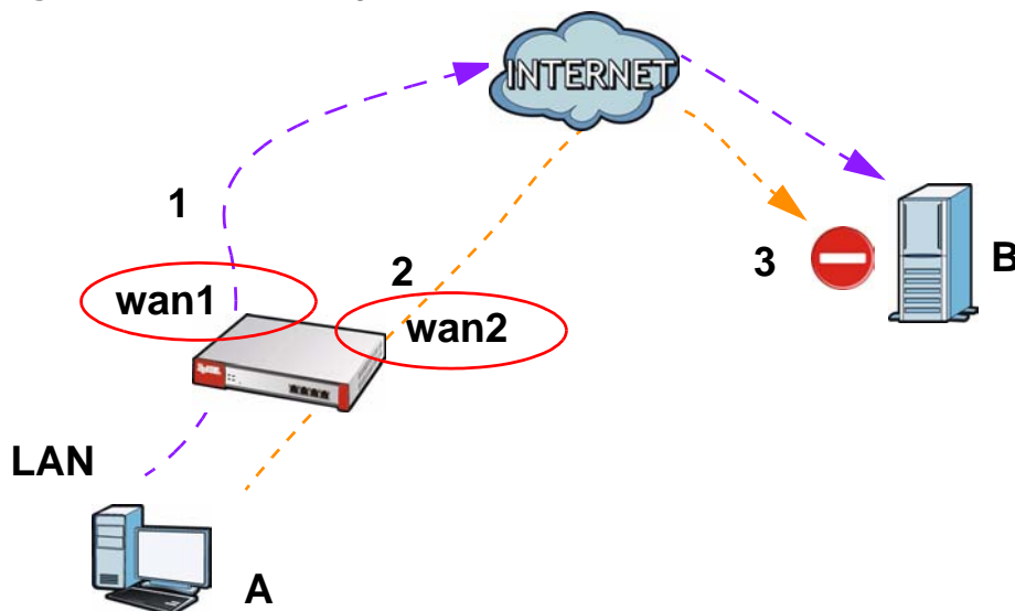
Figure 171 Link Sticking
