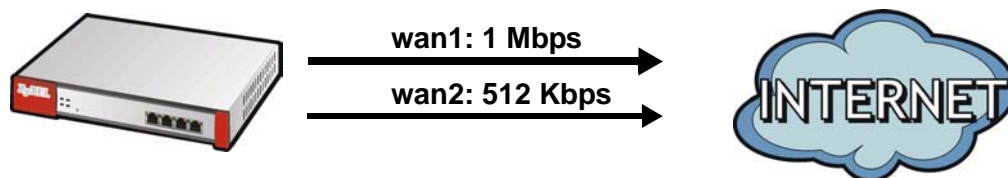
Figure 64 Trunk Example
