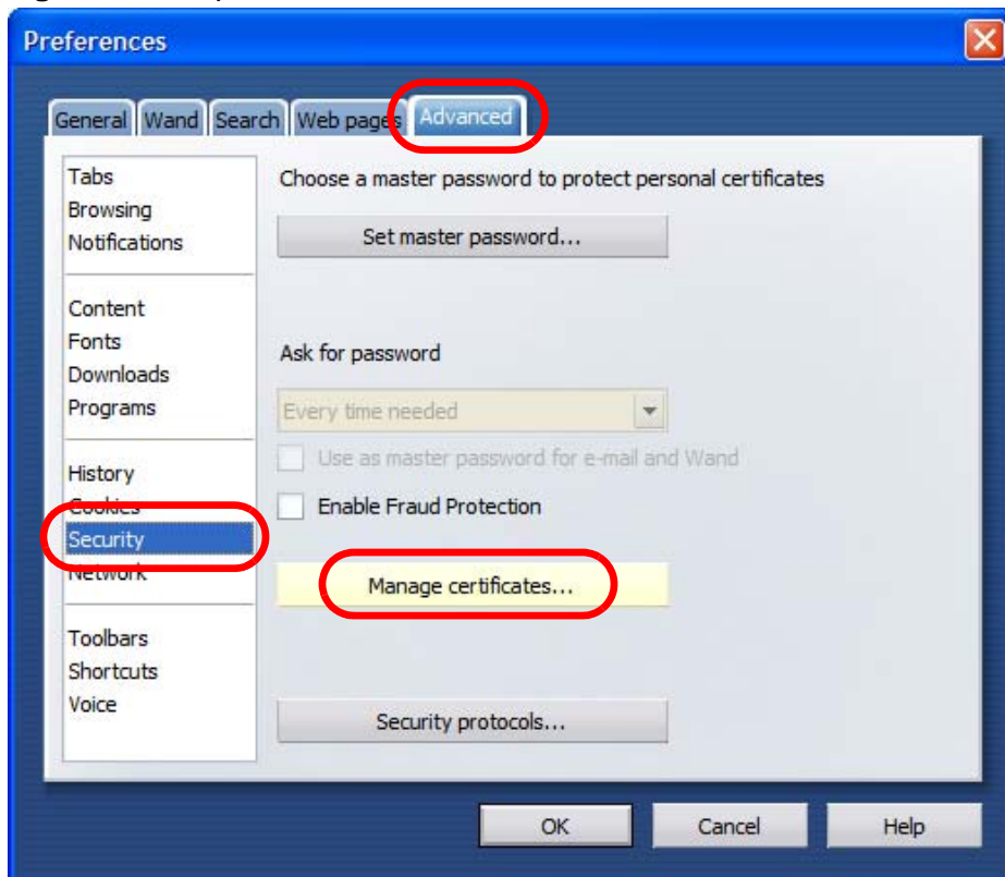
Figure 516 Opera 9: Preferences
