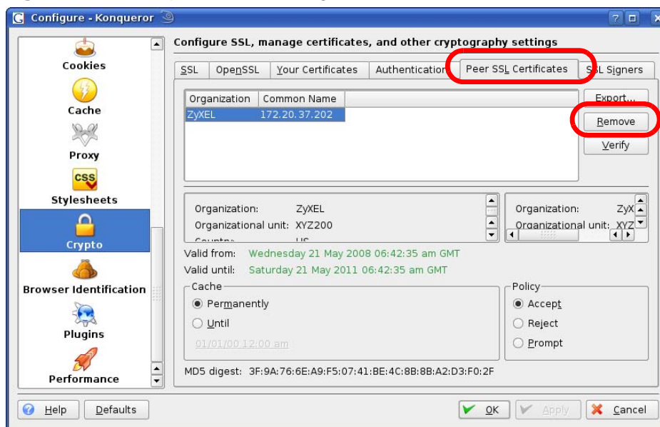
Figure 525 Konqueror 3.5: Configure
