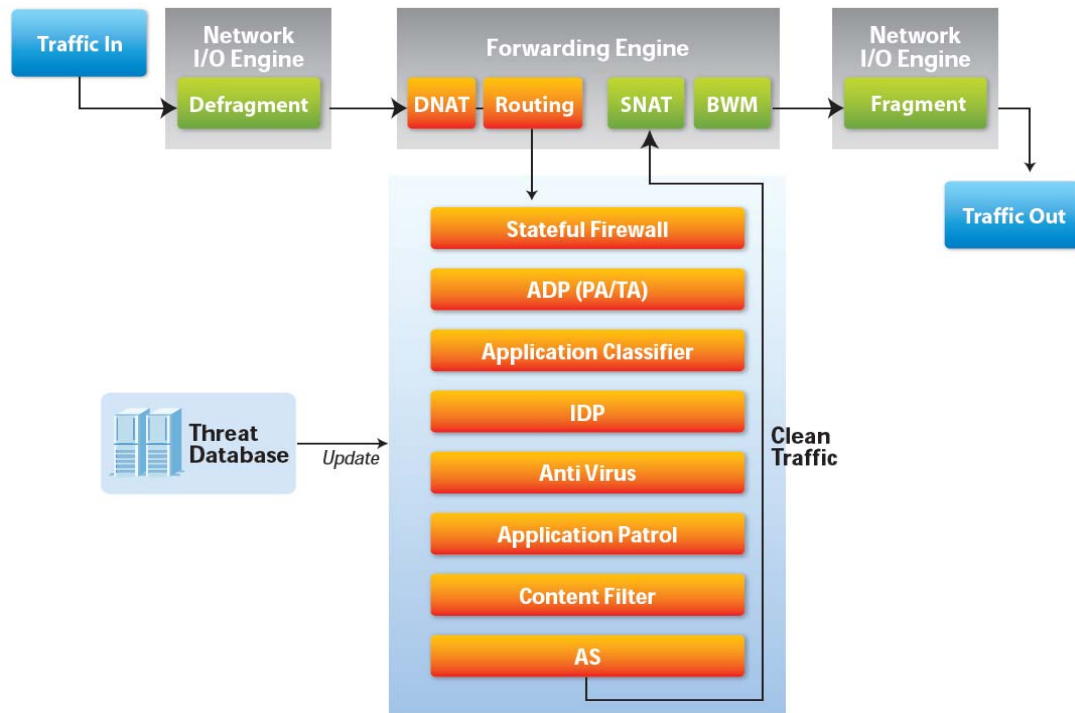
Figure 53 Packet Flow
