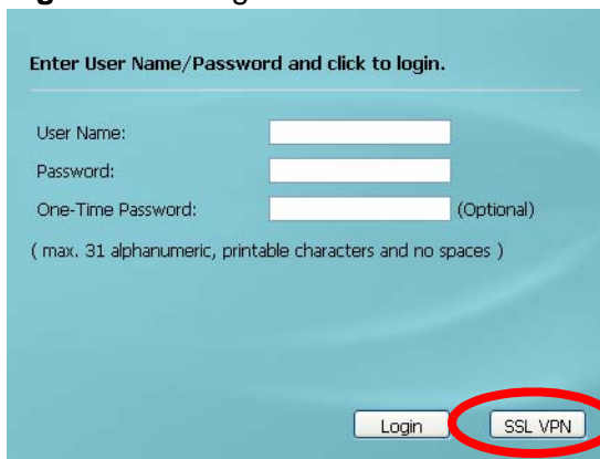
Figure 253 Login Screen
