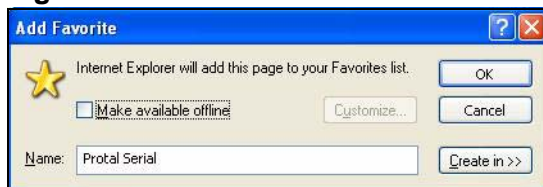
Figure 261 Add Favorite
