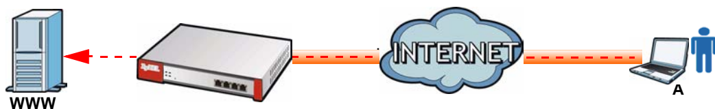
Figure 250 Network Example
