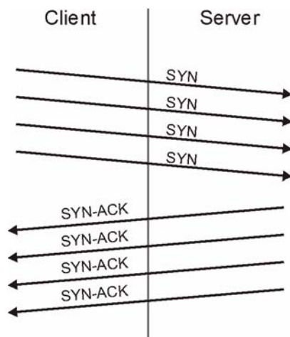
Figure 313 SYN Flood
