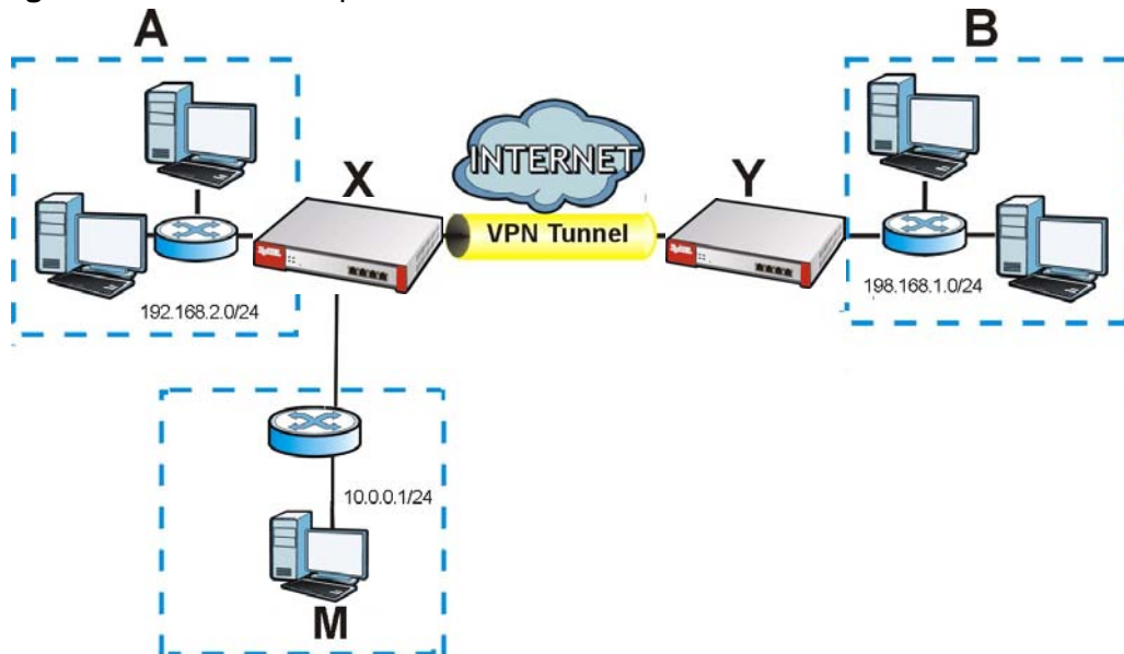
Figure 242 VPN Example: NAT for Inbound and Outbound Traffic
