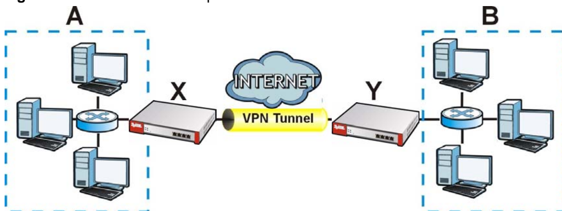
Figure 230 IPSec VPN Example
