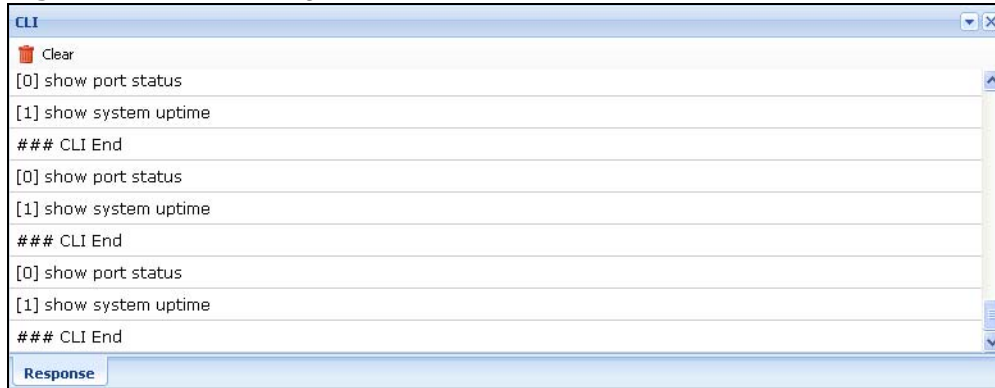
Figure 18 CLI Messages
