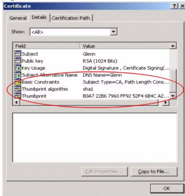
Figure 368 Certificate Details
