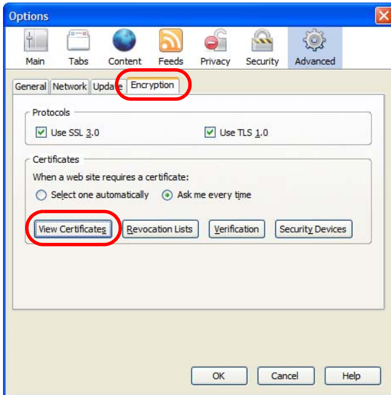
Figure 504 Firefox 2: Options
