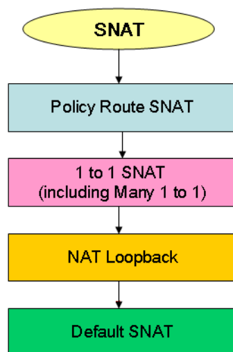
Figure 55 NAT Table Checking Flow
