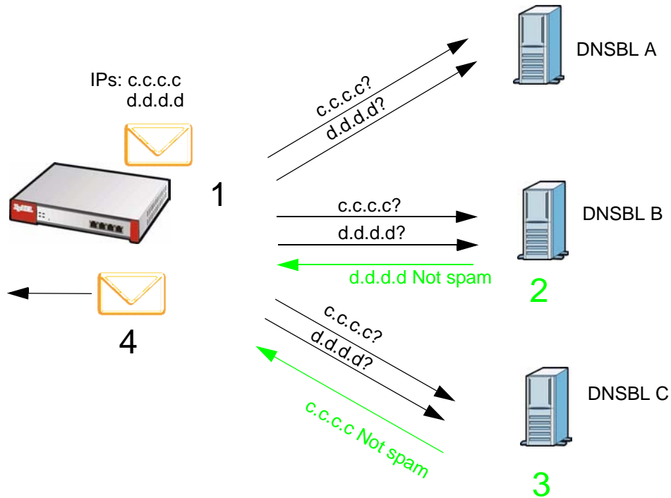
Figure 335 DNSBL Legitimate E-mail Detection Example
