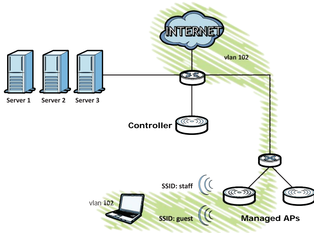
Figure 19 Tutorial Guest VLAN Example
