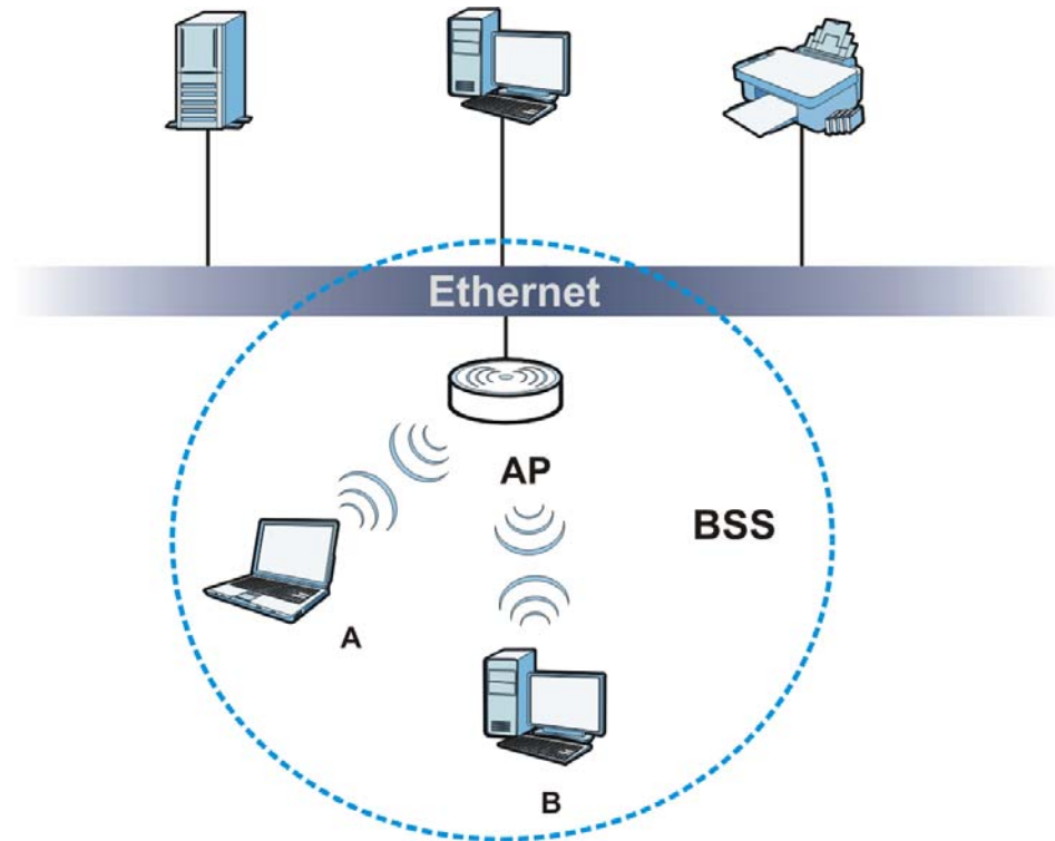
Figure 128 Basic Service Set
