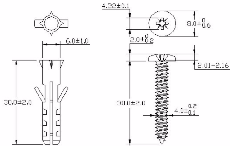
Figure 126 Masonry Plug and M4 Tap Screw
