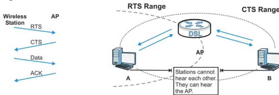
Figure 199 RTS/CTS
