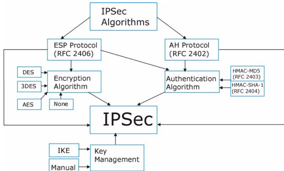
Figure 121 IPsec Architecture
