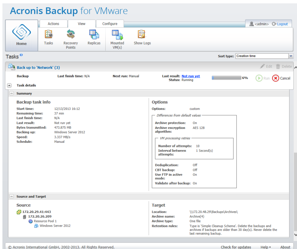
Managing tasks, View task details, Summary tab, Source and Target tab
