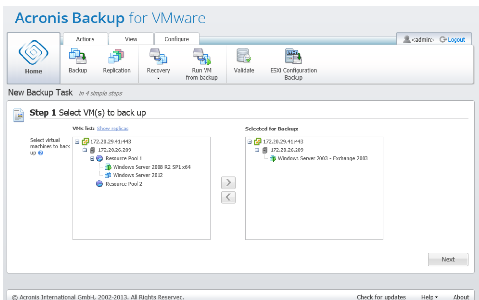
New Backup Task wizard, Step 1 "Select VM(s) to back up"
