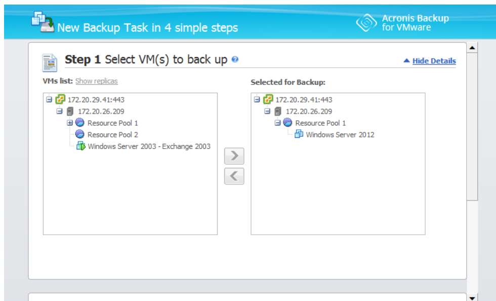
vCenter Integration, New Backup Task, step 1
