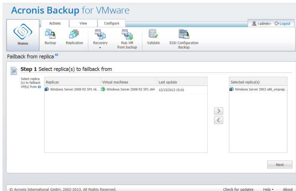
Failback from Replica, step 1 “Select Replica(s) to failback from”
