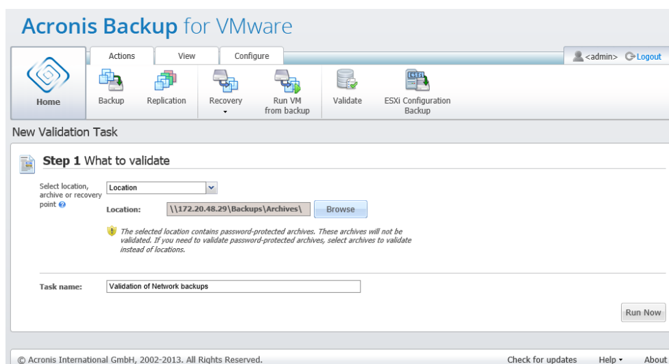
New Validation Task. What to validate. Location.
