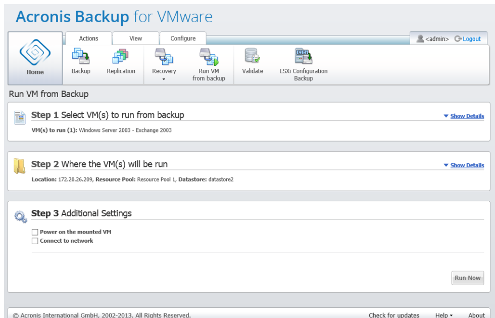
Run VM from Backup wizard, Step 3 “Additional Settings”
