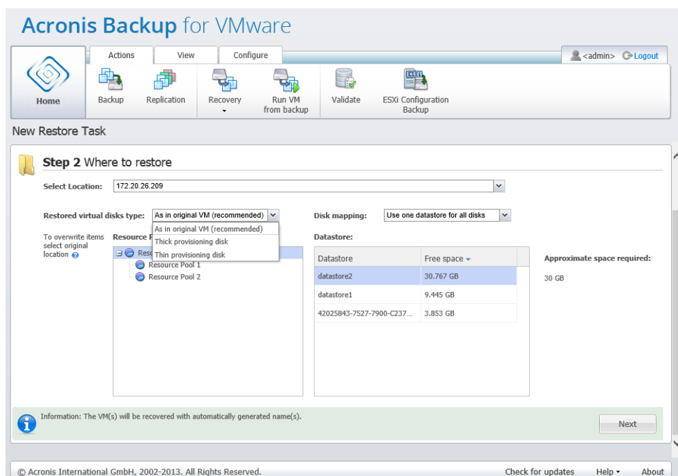
New Restore Task wizard, Step 2 “Where to restore”
