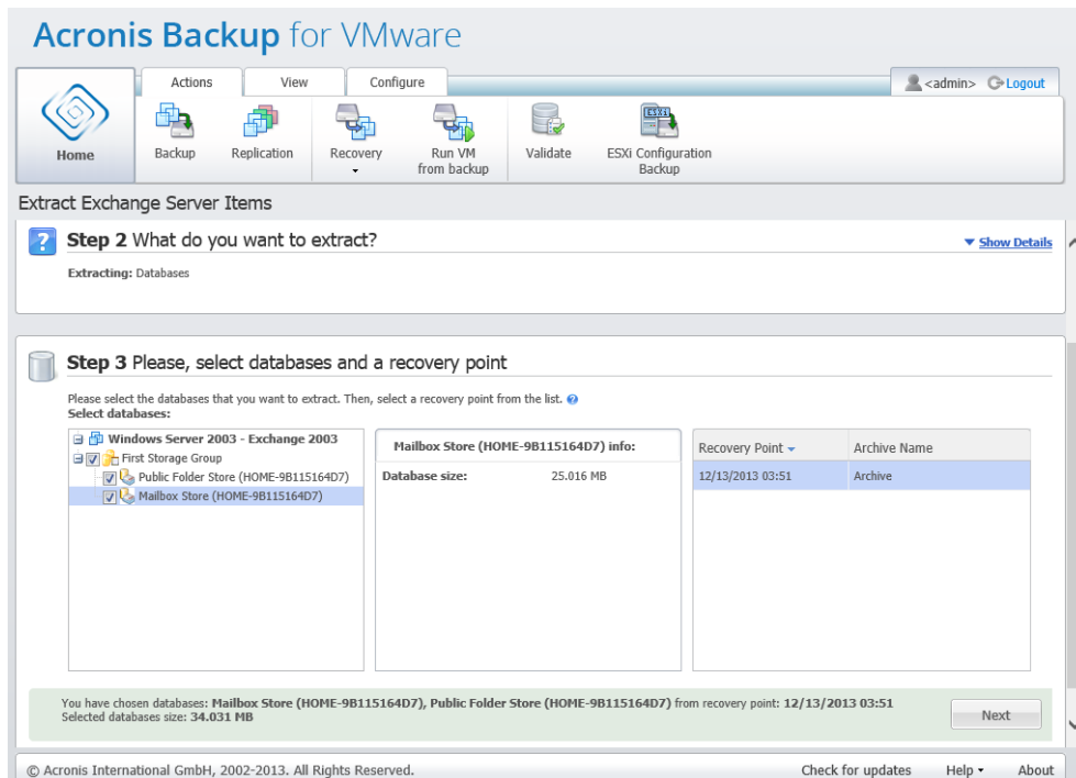
Extract Exchange Server Items, Selecting databases and a recovery point
