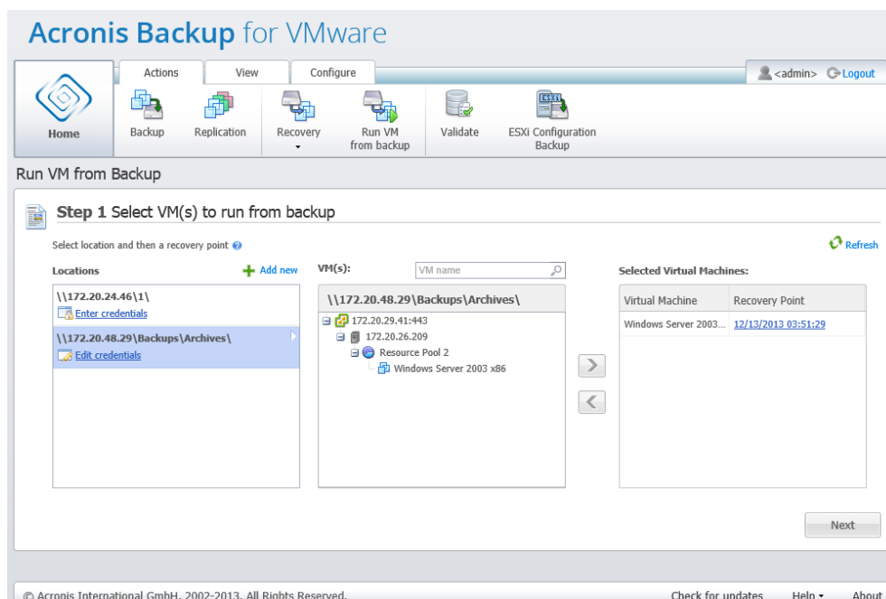
Run VM from Backup wizard, Step 1 “Select VM(s) to run from backup”
