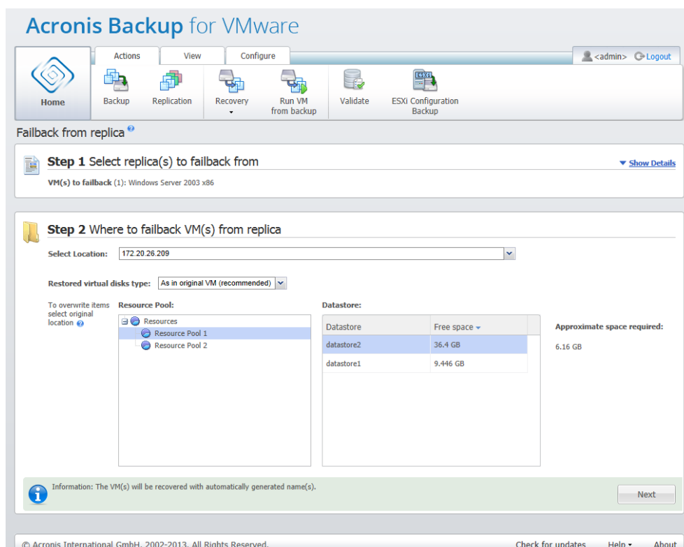
Failback from Replica, step 2 “Where to failback VM(s) from replica”
