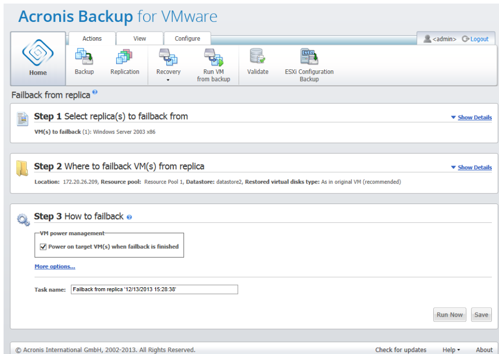
Failback from Replica, step 3 “How to failback”
