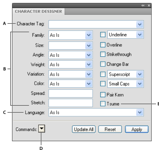
Character Designer
