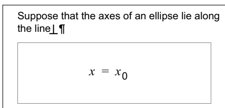
Inserted elements
