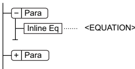
Equation element
