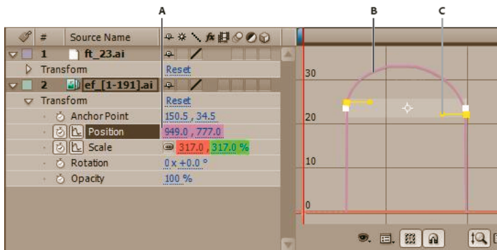
A Value at the current-time indicator B Speed graph C Direction handle (controls speed)
