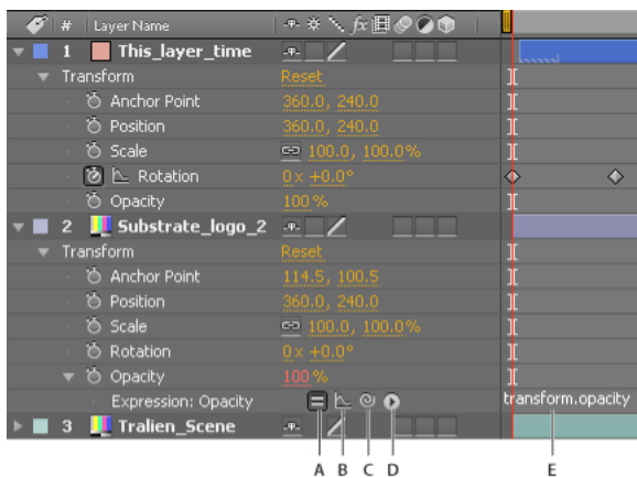
A Enable Expression switch B Show Post-Expression Graph button C Pick whip D Expression Language menu E Expression field
