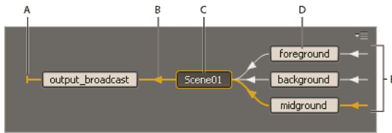
A Indicator that composition does not flow into other compositions B Flow direction C Active (current) composition D Upstream compositions E Indicators that other compositions flow into these compositions
