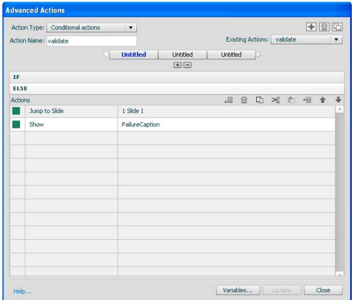
ELSE condition in the 'validate' advanced action
