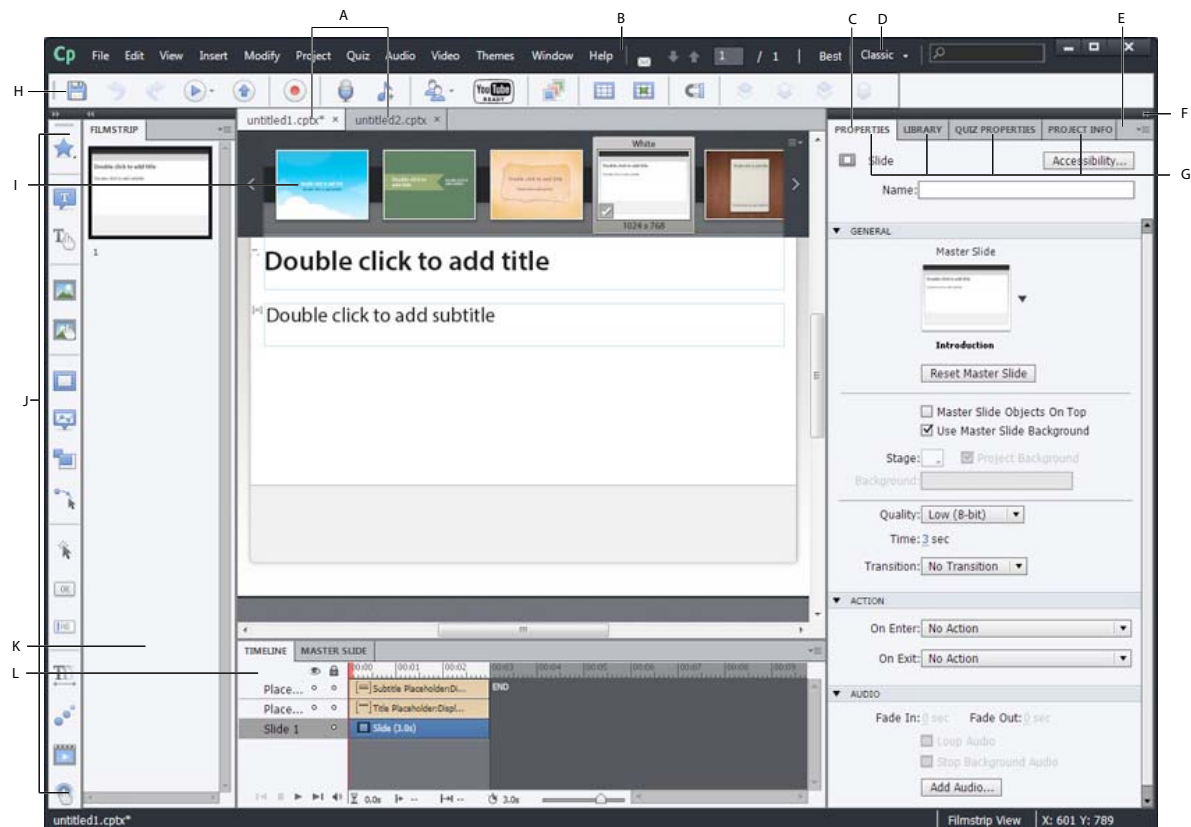
A. Tabbed Document windows B. Application bar C. Property Inspector D. Workspace Switcher E. Panel title bar F. Collapse to icons button G. Panel groups in vertical dock H. Control Panel I. Themes bar J. Object toolbar K. Filmstrip L. Timeline
