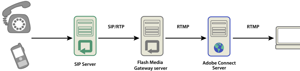
Audio flows from a phone, through an audio conference server (not pictured), through a SIP server, through Flash Media Gateway, to an Adobe Connect meeting room.
