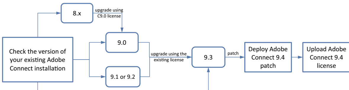
Adobe Connect 9.4 upgrade workflows
