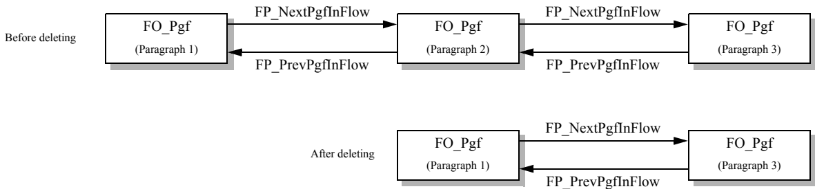
Figure 8-4 FO_Pgfl objects in a flow before and after deleting an FO_Pgfl object
