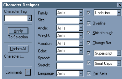
Figure 2-16 Character Designer
