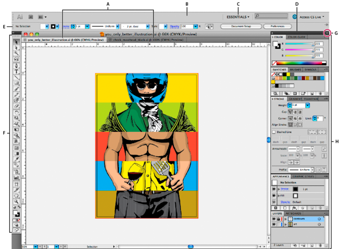
Default Illustrator workspace A Tabbed Document windows B Application bar C Workspace switcher D Panel title bar E Control panel F Tools panel G Collapse To Icons button H Four panel groups in vertical dock
