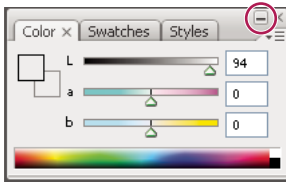
Minimize button
