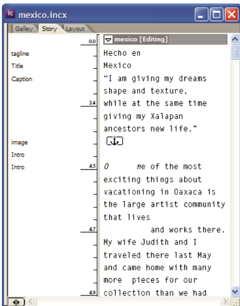
Story view
