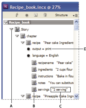
Structure pane
