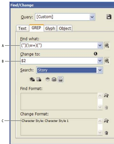
GREP example
