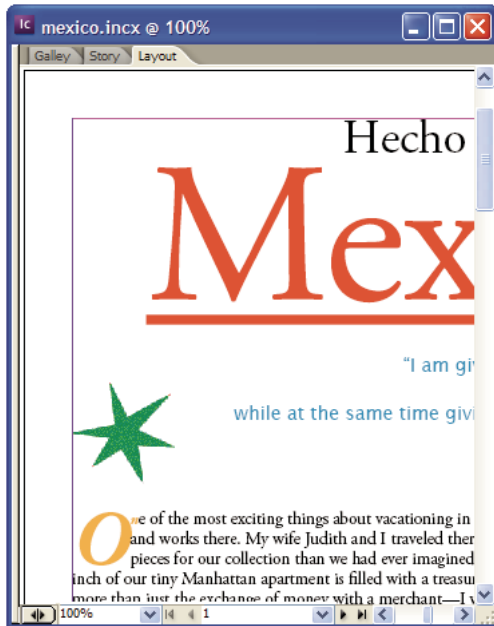
Layout view
