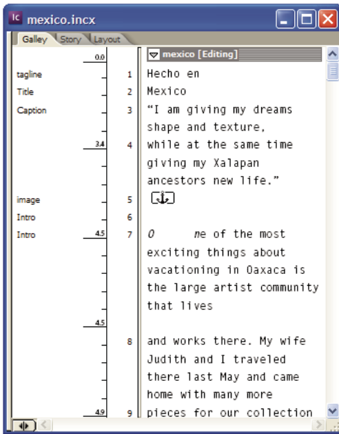
Galley view
