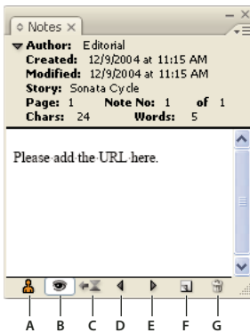
Notes panel
