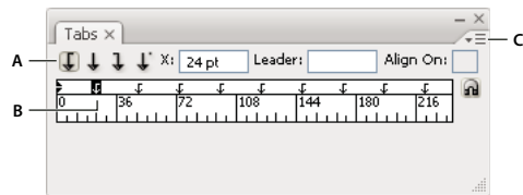
Repeated tabs
