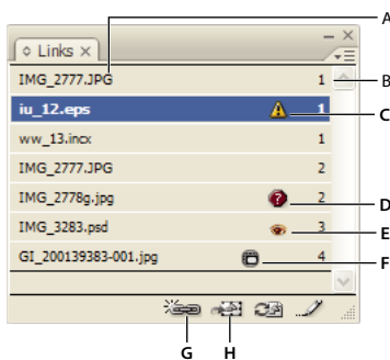
Links panel
