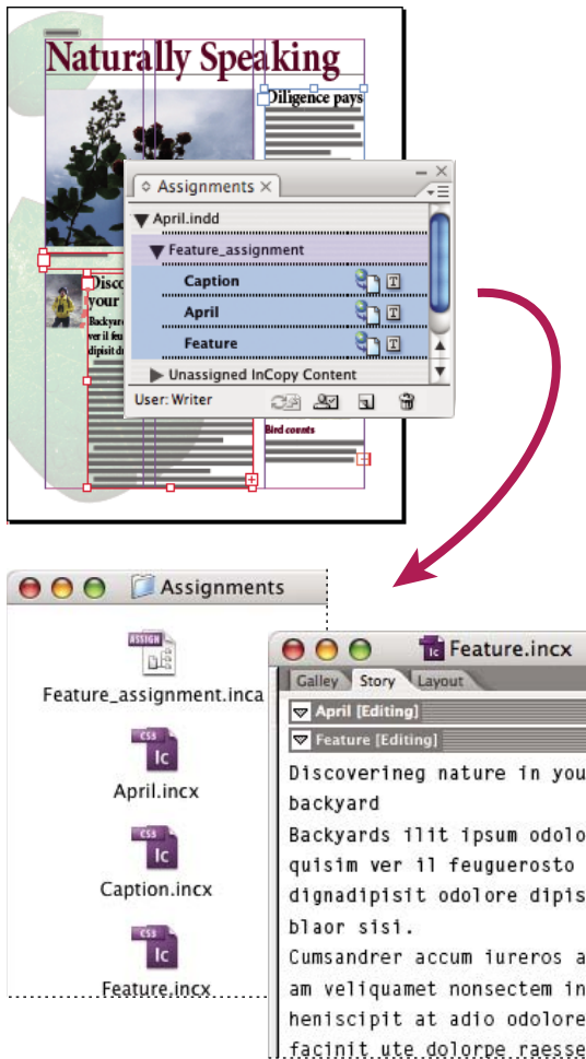
InDesign document (.indd) with assignment file (.inca) composed of three linked content files (.incx). Assignment and its components are listed in Assignments panel and are opened in InCopy.
