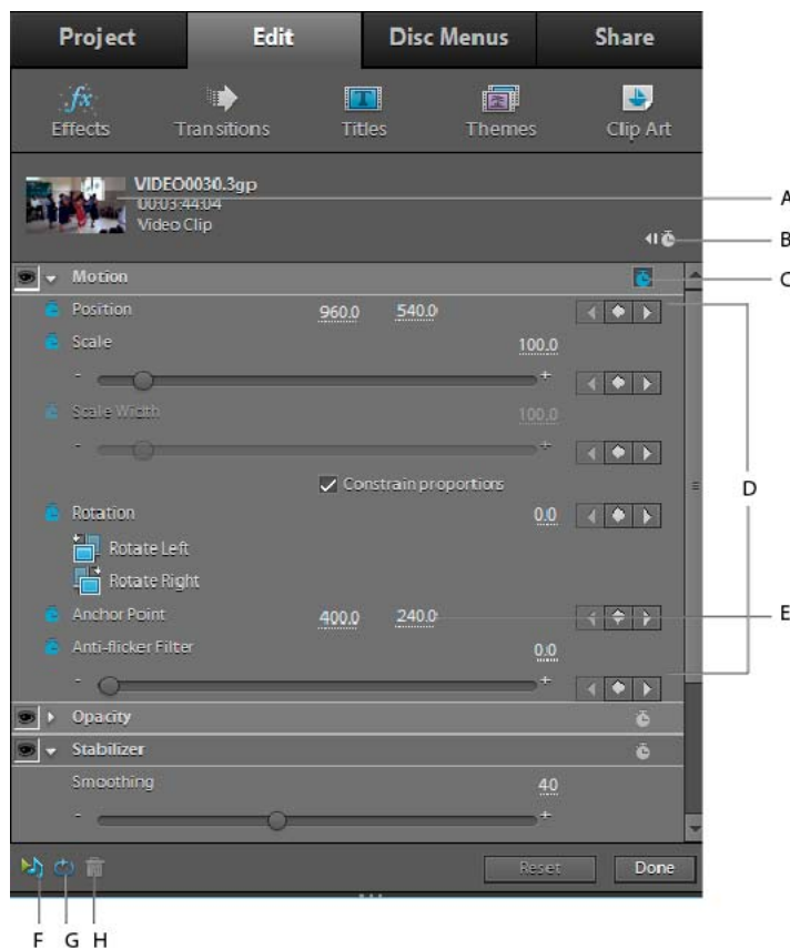
Properties view
