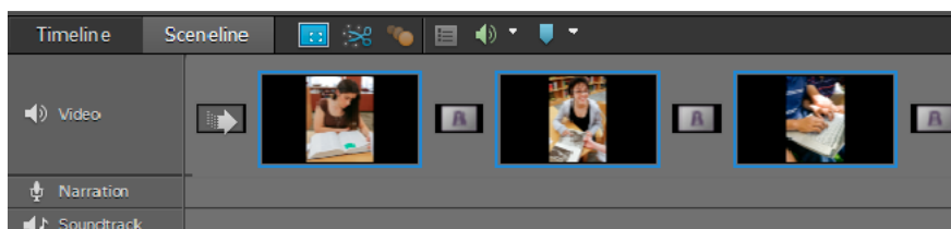
Sceneline
