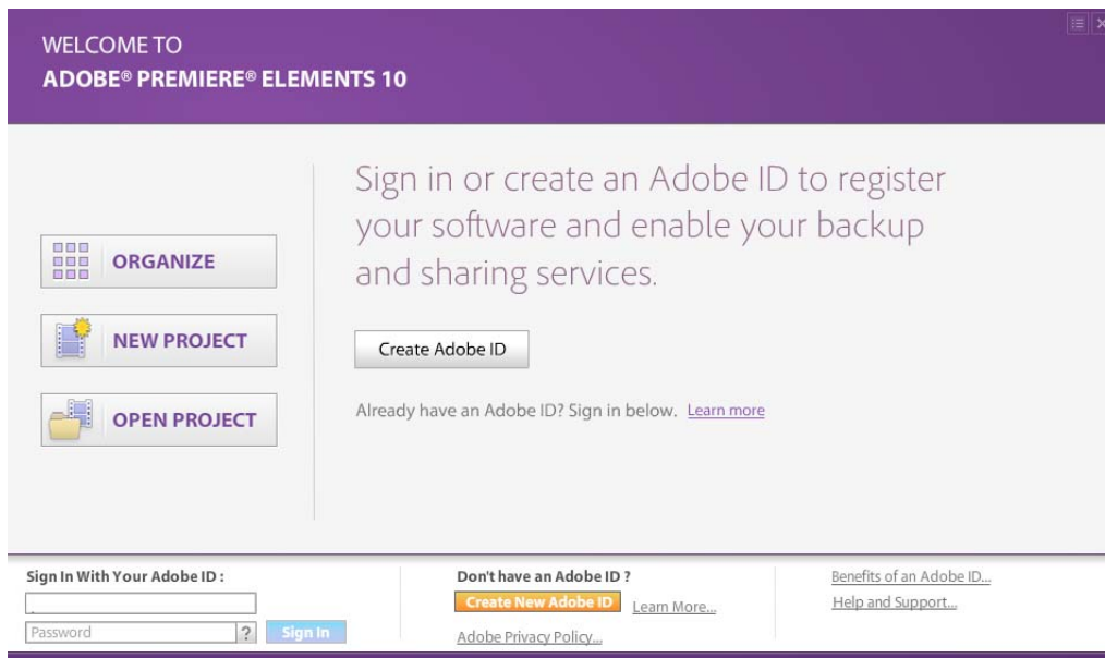
Welcome screen
