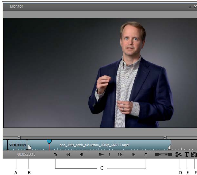
Monitor panel
