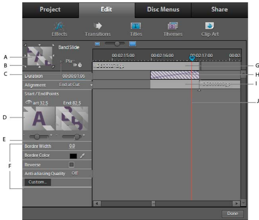
Properties view
