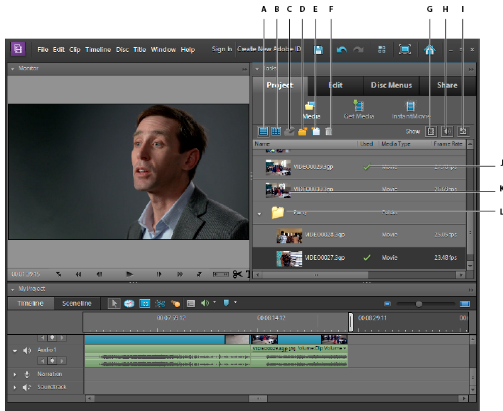
Project view
