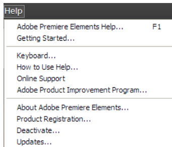
Help menu
