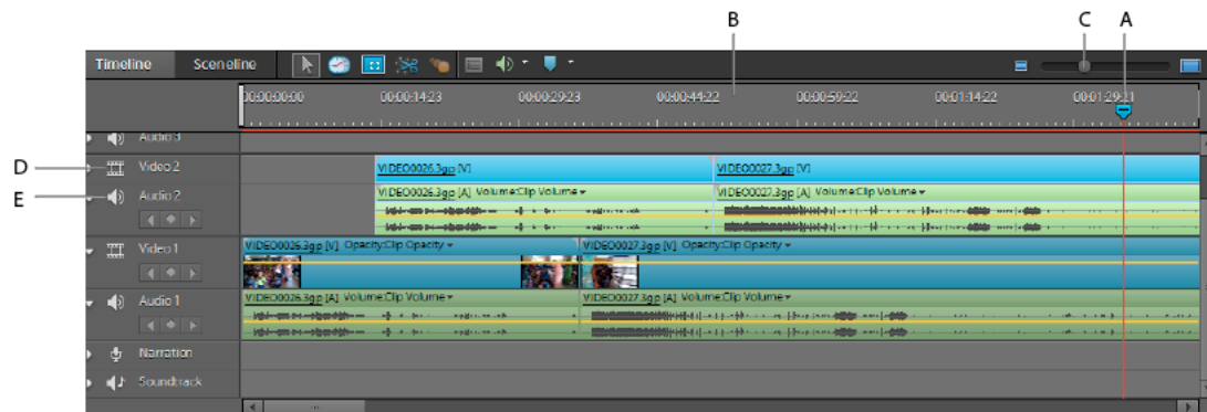
Timeline
