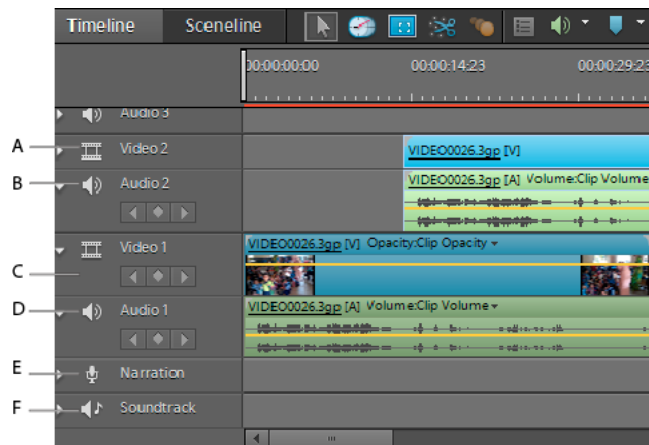
Default tracks
