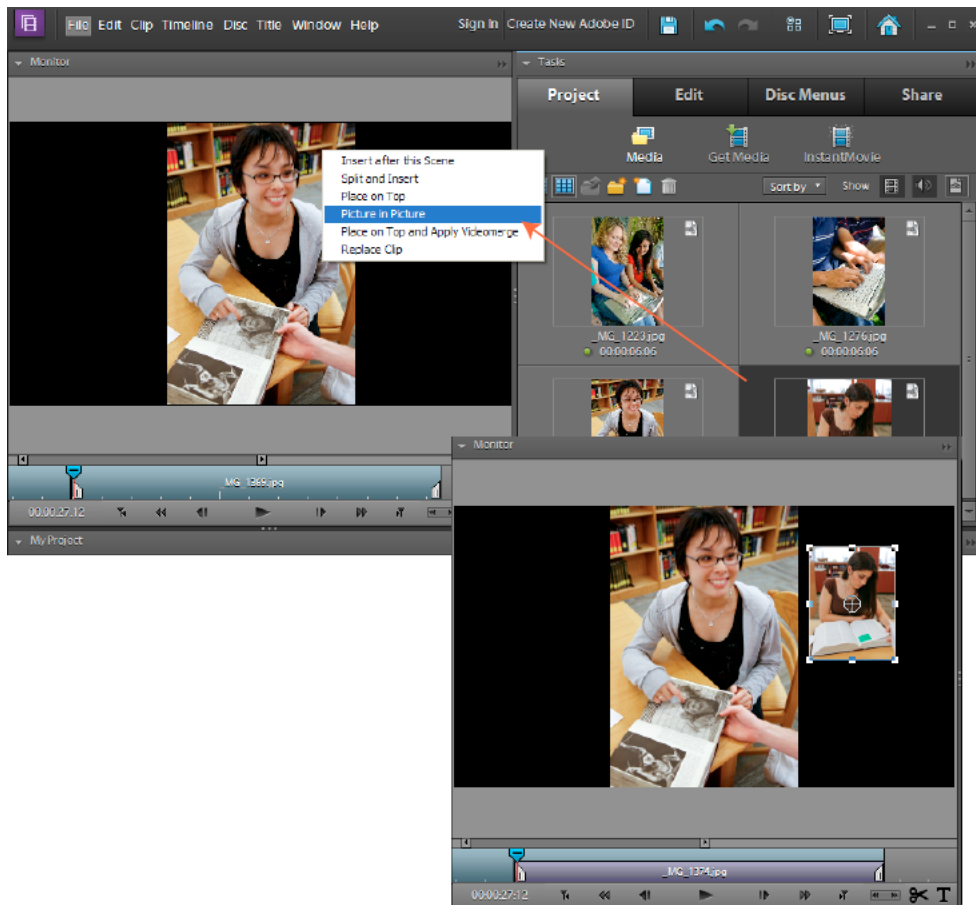
Picture-in-picture overlay
