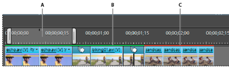
Timeline
