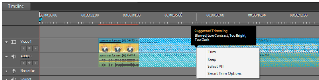
Smart Trim
