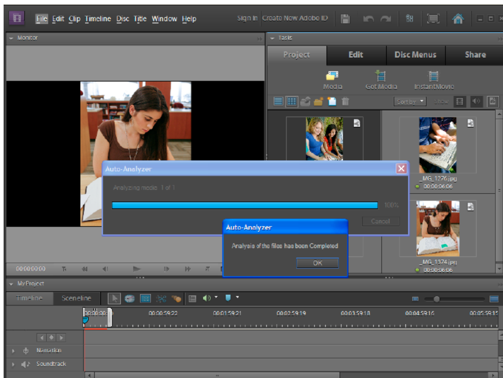
Auto-Analyzer window
