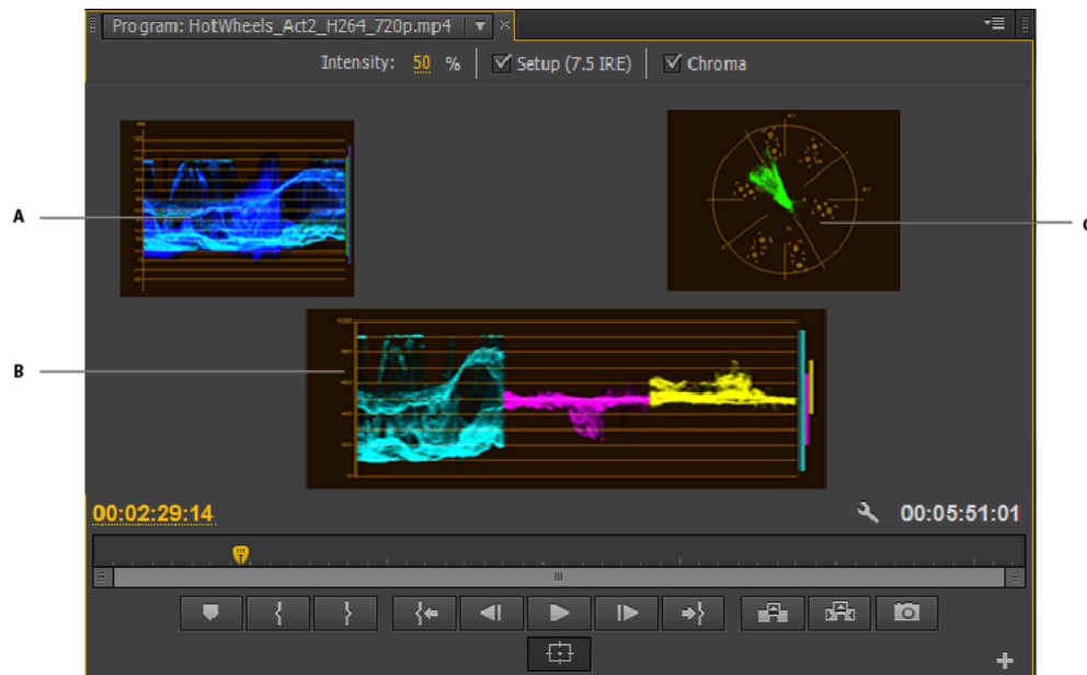
Program Monitor set to Vect/YC Wave/YCbCr Parade A Waveform monitor B YCbCr Parade C Vectorscope
