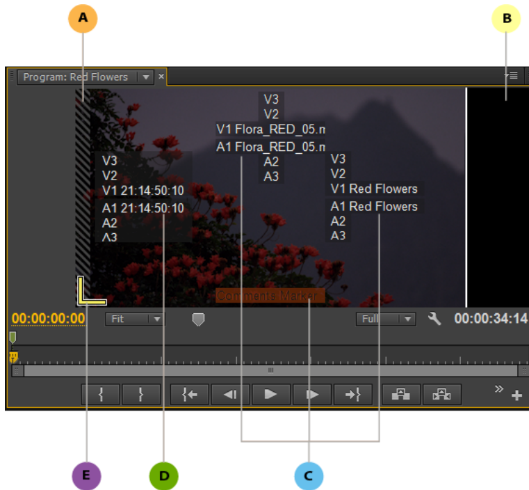
A Media Limit indicator B End Of Media indicator C Metadata aligned Right, Bottom Middle, and Top Middle D Source Timecode aligned Left E Edit Point indicator
