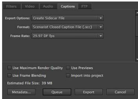
Export Setting for Closed Captions
