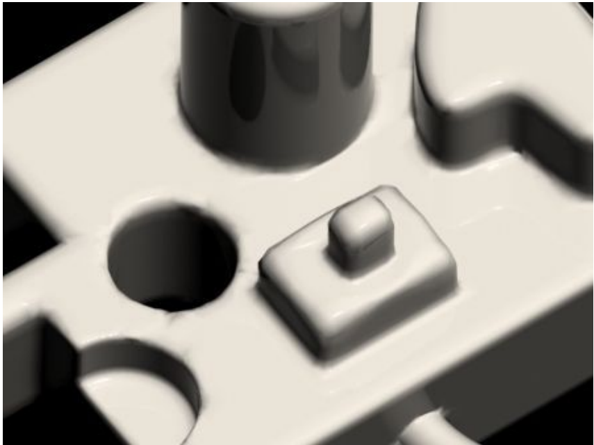
When rendered, misshapen geometry results from the presence of coplanar edges.
