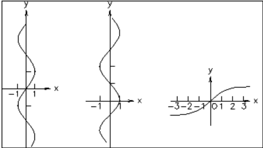
Graphs of basic arc functions
