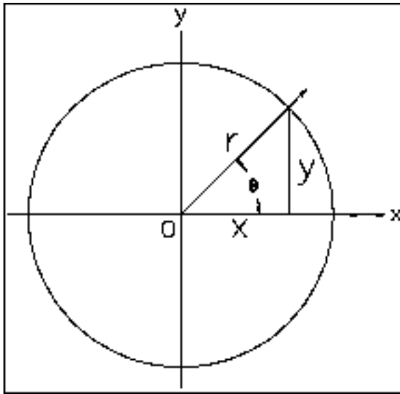
Trigonometric functions based on the unit circle
