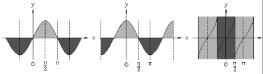
Graphs of basic trigonometric functions
