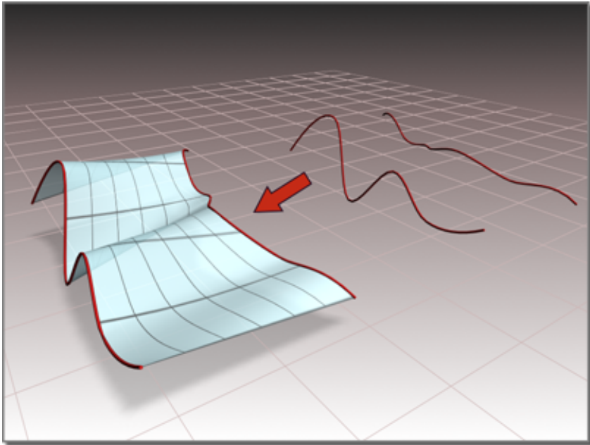
Using two curves to create a ruled surface
