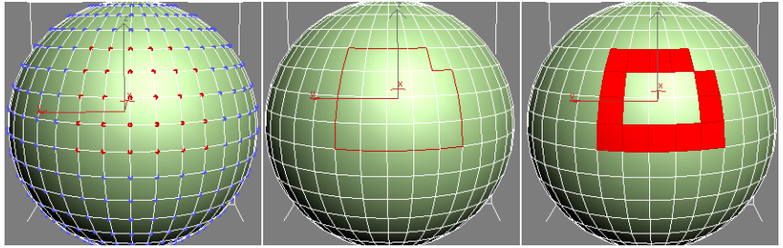
Vertex selection (left) converted to edge border (center) and face border (right)
