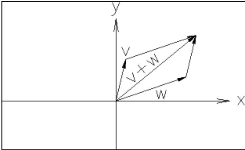
Adding two vectors
