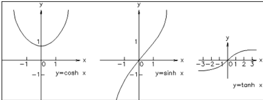
Graphs of basic hyperbolic functions
