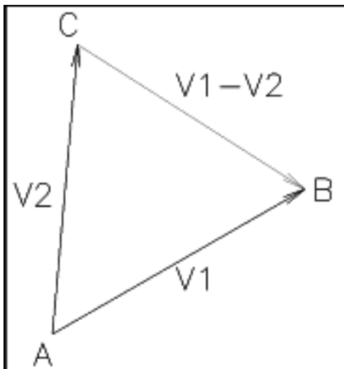
Subtracting two vectors
