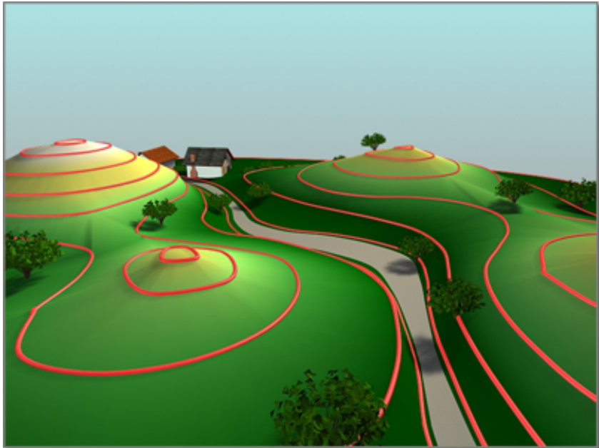
Terrain created as a graded surface
