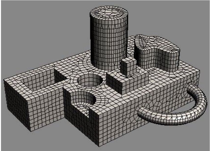
Quad meshing with Quad Size %=2.0
