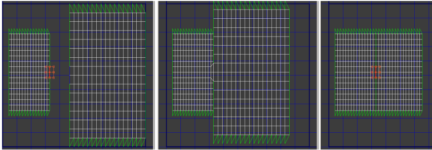
Edges chosen to stitch (left); Clusters aligned (center); Clusters aligned and scaled, with Bias=0 (right)
