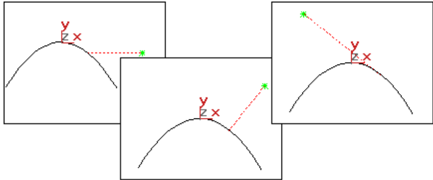
Offset, normal, and tangent displacement of a curve point
