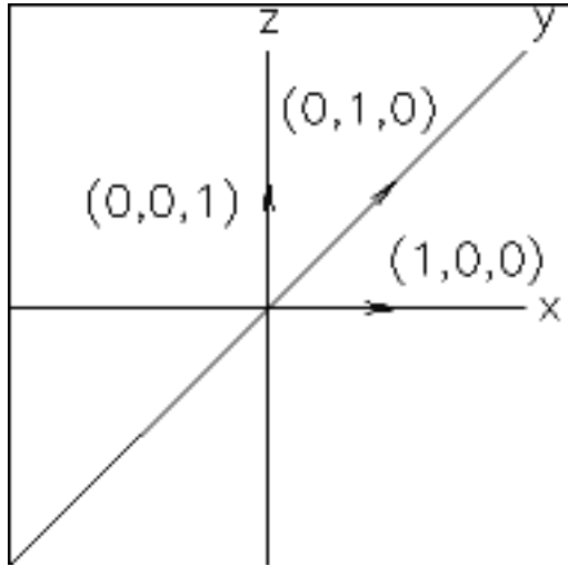
Basic vectors and the XYZ axes
