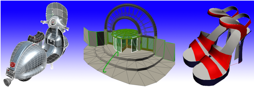
Three types of surface models: patch (left); mesh (center); NURBS (right)
