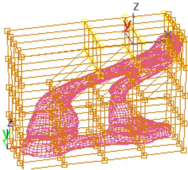
Object and object surrounded by an FFD lattice
