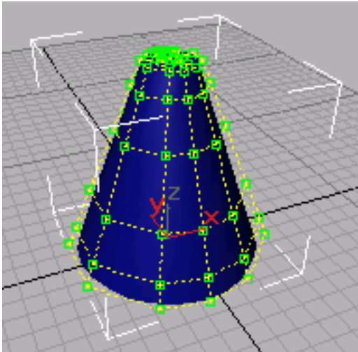
Cone-shaped NURBS surface with its control lattice (CVs are displayed as green squares)
