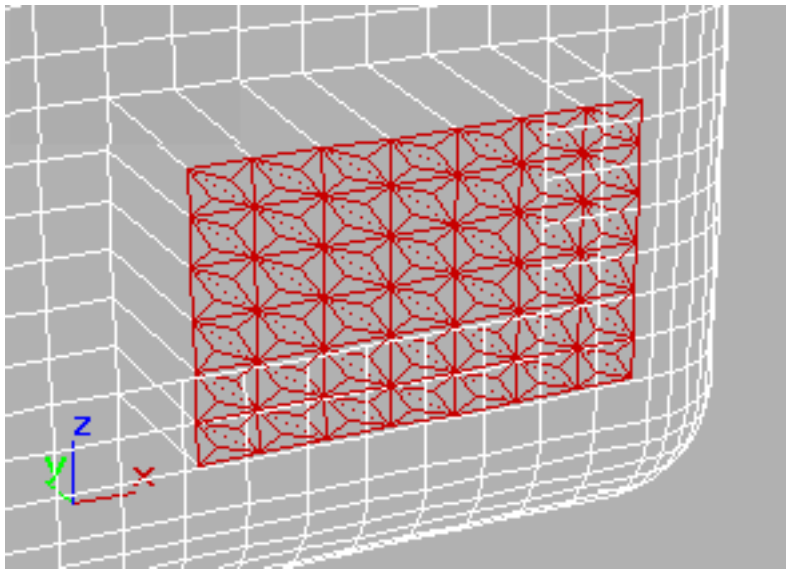
Set of polygons showing Face-Center tessellation
