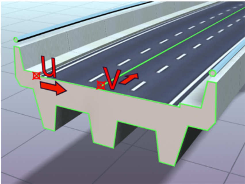
Mapped roadway showing U and V dimensions for the loft
