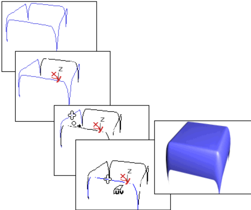
Using perpendicular curves to create a UV loft surface
