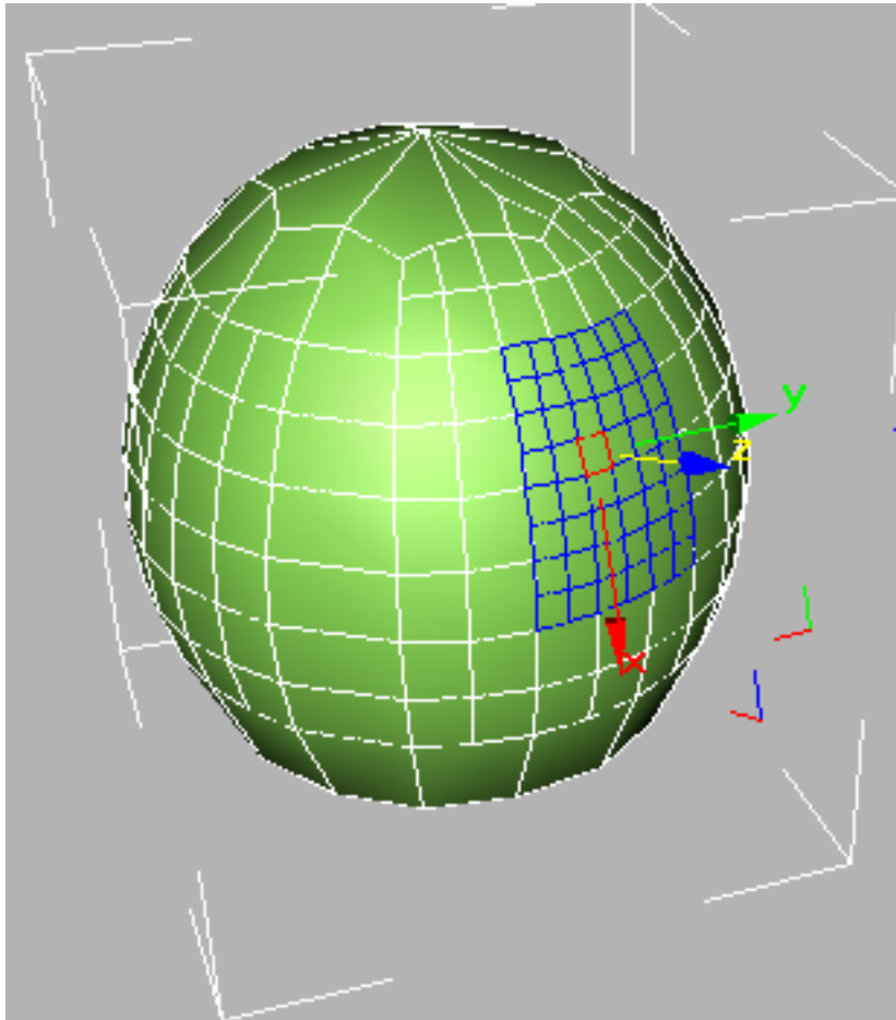
A control grid on a sphere at level 2. Subdivisions at lower levels are visible as gold lines.
