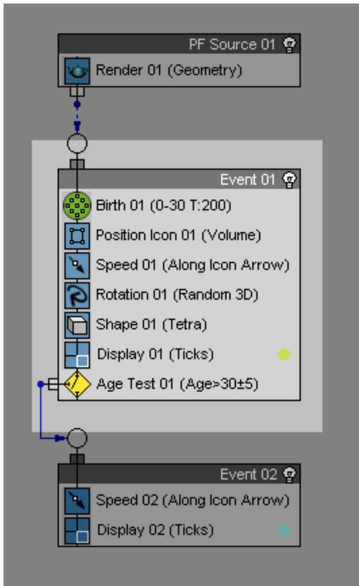
Birth event (highlighted)
