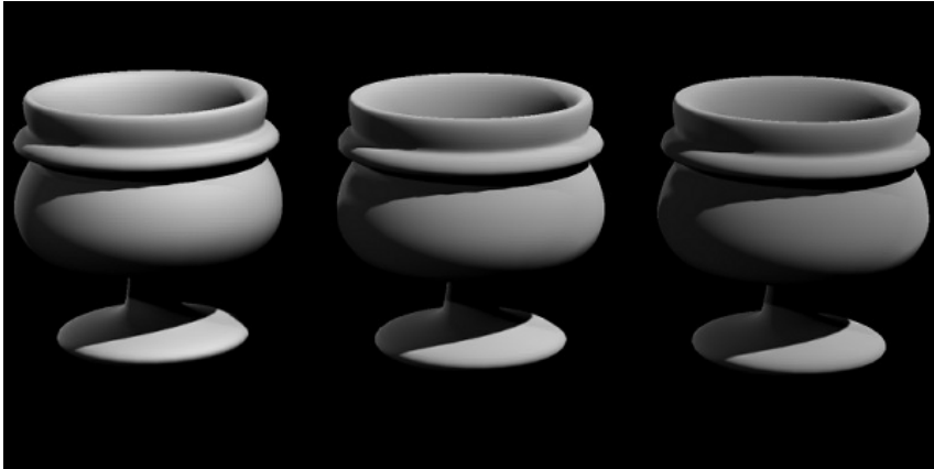
Left: Roughness=0.0; Center: 0.5; Right: 1.0
