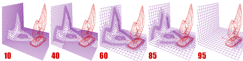
Radiosity solutions with different Contrast Threshold values. The best solution is at the center, with Contrast Threshold=60.
