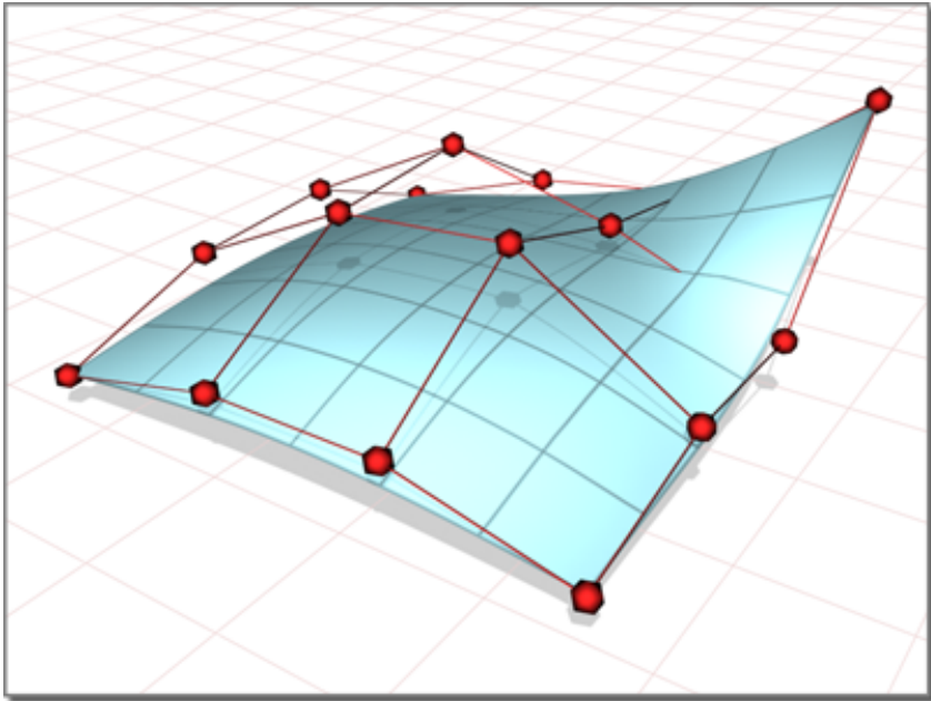
CVs (control vertices) in the lattice surrounding a NURBS surface
