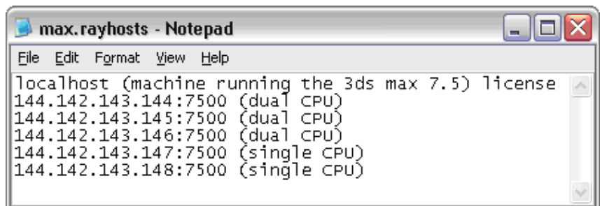
Figure 1 - Example of a rayhost file
