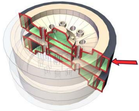
Red line shows the section shape based on the structure.
