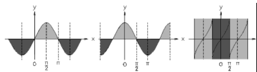
Graphs of basic trigonometric functions
