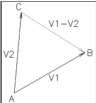
Subtracting two vectors
