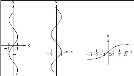
Graphs of basic arc functions
