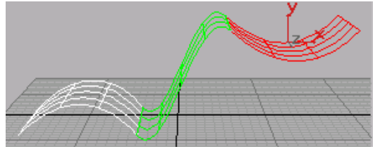
Moving a parent surface changes the blend surface (the blend surface is displayed in green)
