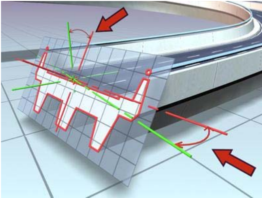
Roadway lofted with teeter turned on. Teeter affects the X and Y axis orientation of the shape in relation to the path.
