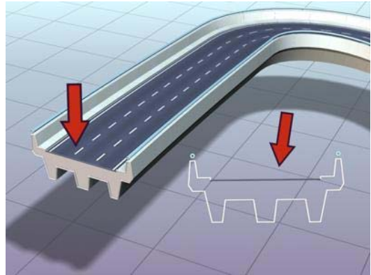
Shape material IDs used to give the roadway two materials: concrete for supports and railings, asphalt with white lines for the traffic lanes
