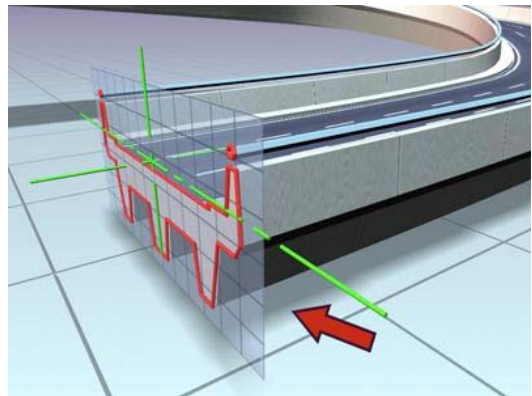
Roadway lofted with no teeter
