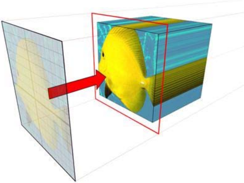
Planar map projection
