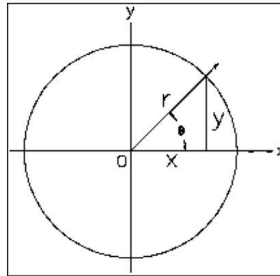
Trigonometric functions based on the unit circle
