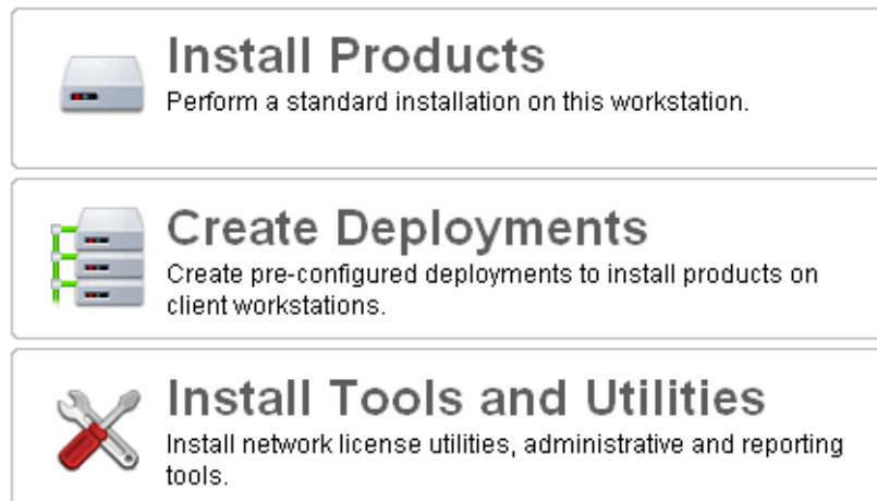
Figure 1. Installation Wizard.
