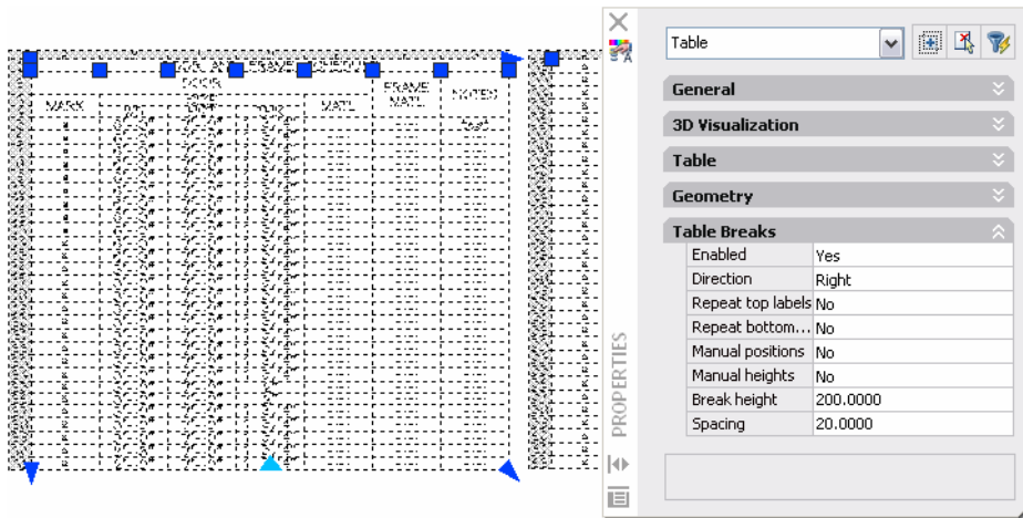
Figure 73. Table Wrapping.
