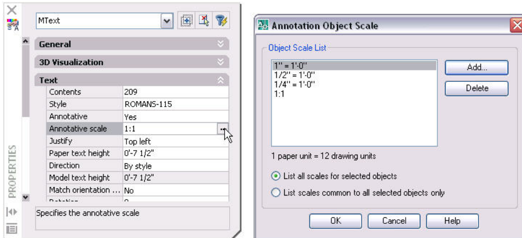
Figure 35. Annotative Scales.
