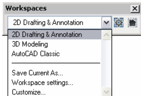
Figure 7. Workspaces.
