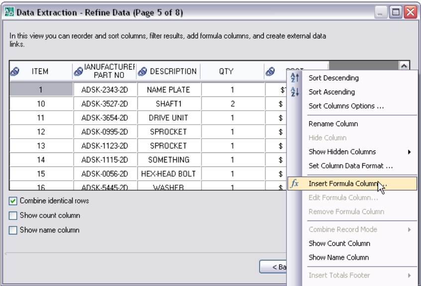
Figure 71. Formula Columns.
