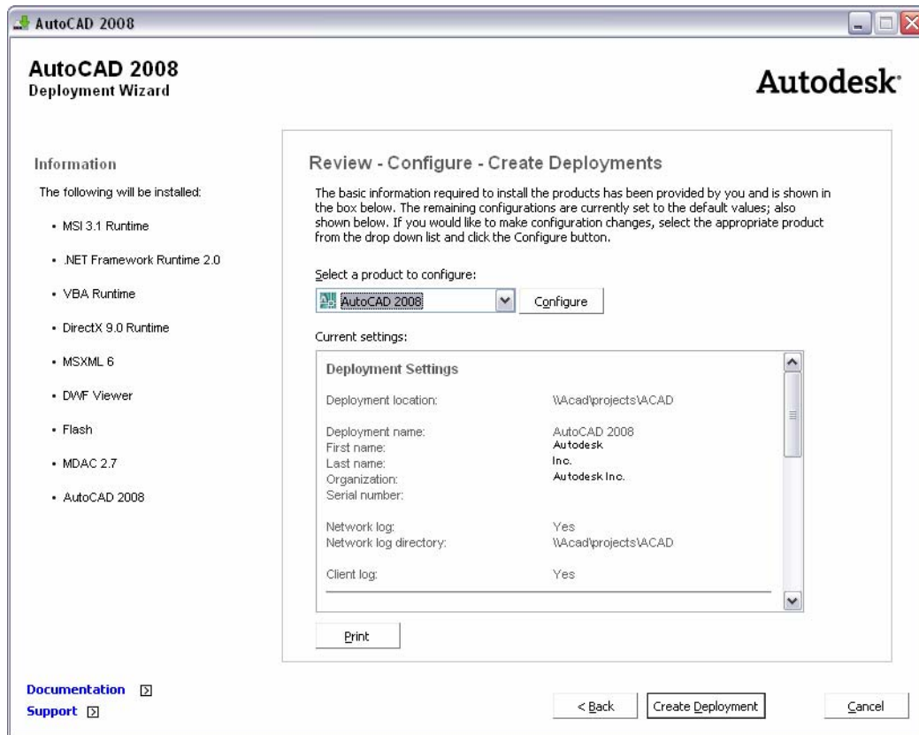
Figure 3. Deployment Wizard.
