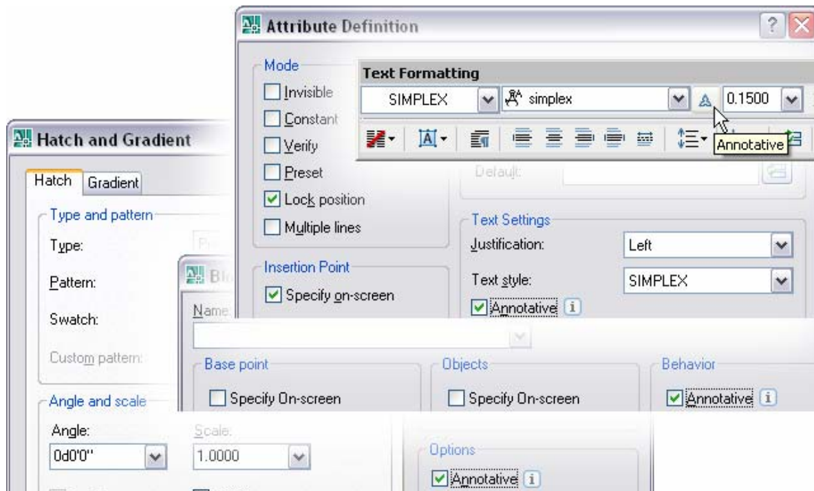
Figure 32. Annotative toggles.
