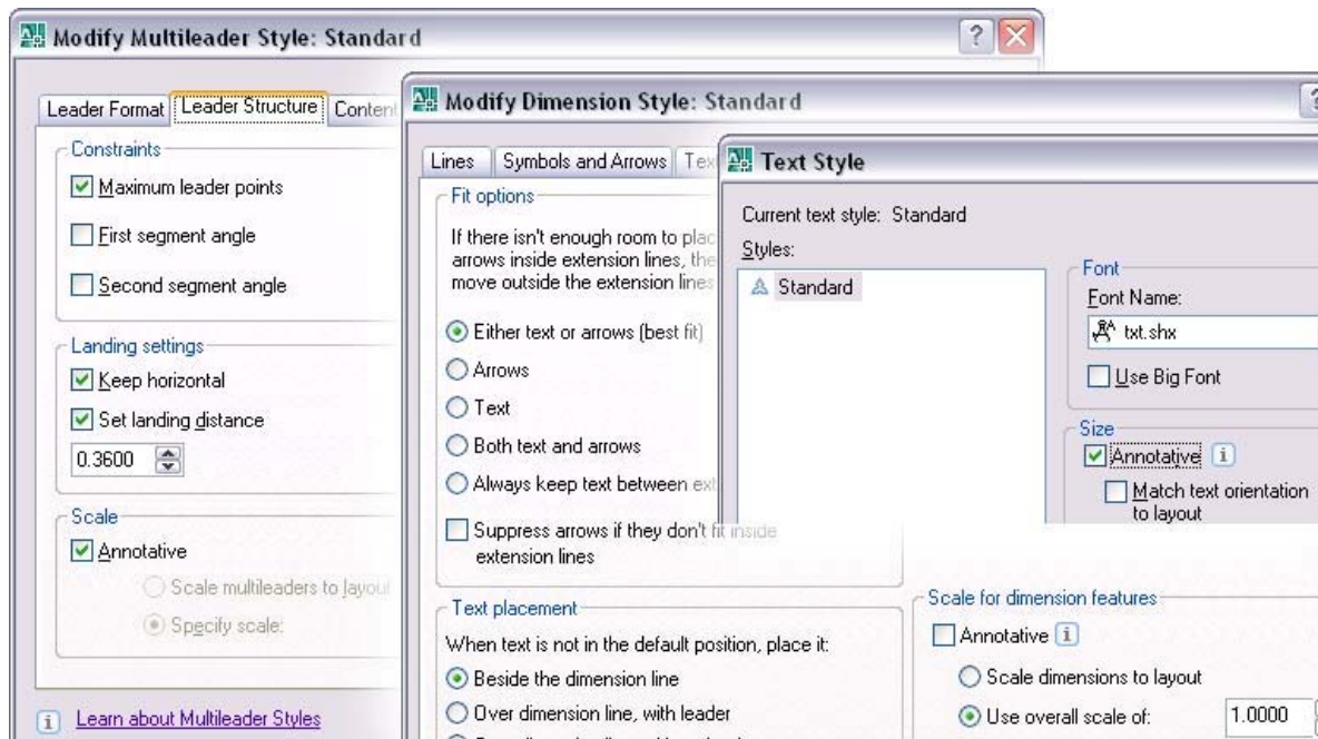
Figure 34. Annotative Styles.
