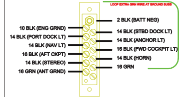
GROUND BUSS
